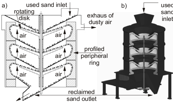
Figure 1. a) Schematic representation of grain movement phases in a centrifugal reclamation unit with profiled rotating disc and specially profiled peripheral ring, b) general view of a reclaimer Slika 1. a) Shematski prikaz faza kretanja zrnaca u uređaju za centrifugalno obnavljanje s profiliranom rotirajućom pločom i posebno profiliranim perifernim prstenom, b) Izgled regeneratora
