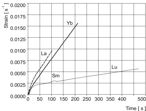
Figure 1. A comparison of compressive creep behavior of RE-Si-Mg-O-N glasses (RE = La, Sm, Yb and Lu)
