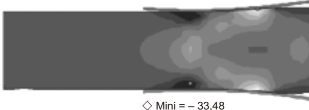
Figure 3. Distribution of stresses \sigma_m within the roll gap, with h_0 = 105,76 mm, \epsilon = 10\% , \theta = 0^\circ , positive values mean compression
