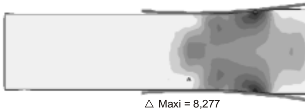
Figure 2. Distribution of stresses \sigma_y within the roll gap, with h_0 = 105,76 mm, \epsilon = 10\% , \theta = 0^\circ
