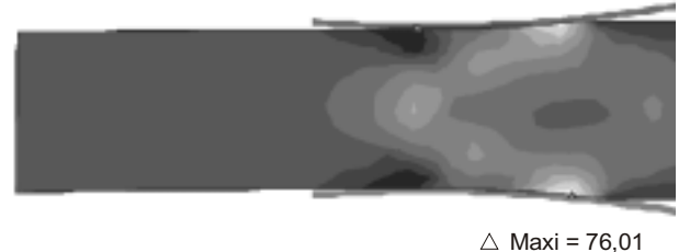
Figure 5. Distribution of stresses \sigma_m within the roll gap, with h_0 = 105,76 mm, \epsilon = 10\% , \theta = 2^\circ , positive values mean compression
