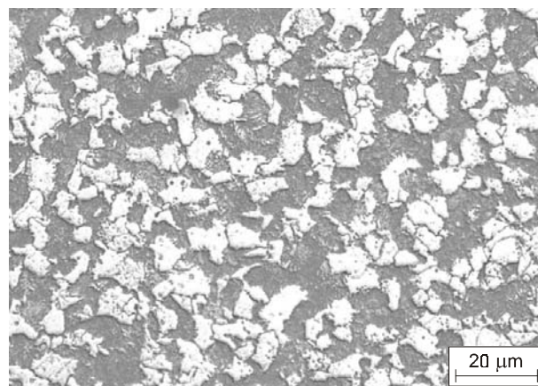
Figure 2. Initial microstructures of applied tool steel (ferrite grains and lamellar pearlite grains)
