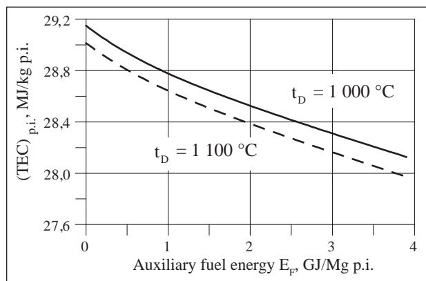
Figure 5 TEC of pig iron
