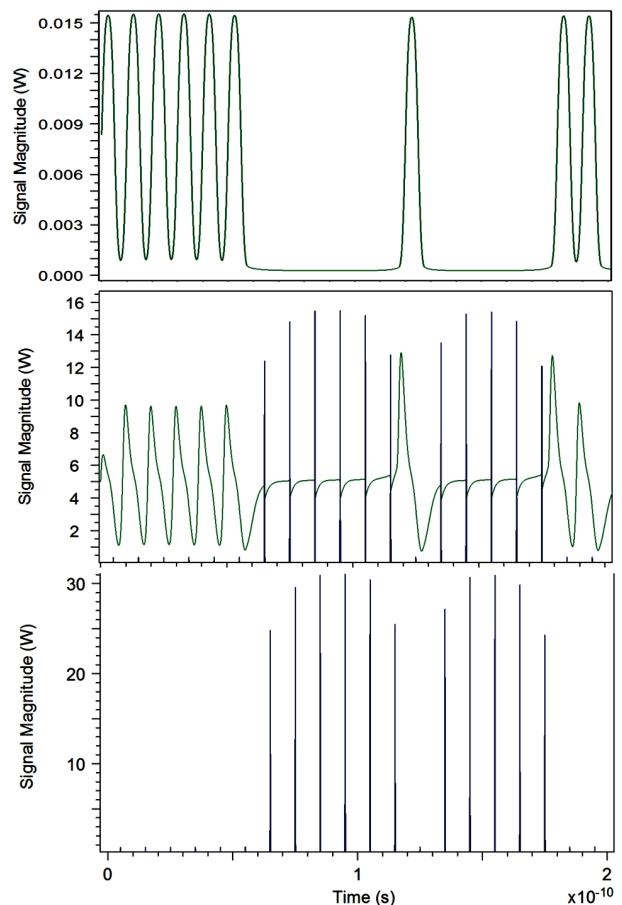
Figure 3 Data produced through CW laser, RZ saturated pulse after passing through SOA and resultant inverted pulse at T-port
