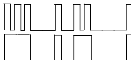
Figure 1 RZ and NRZ Modulation formats
