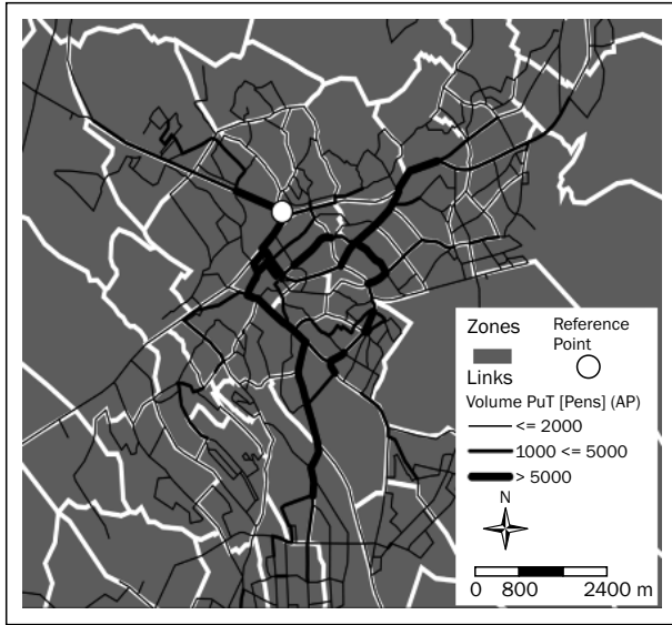
Figure 3 - Link volumes resulting from the UPT timetable-based assignment for the morning peak period
