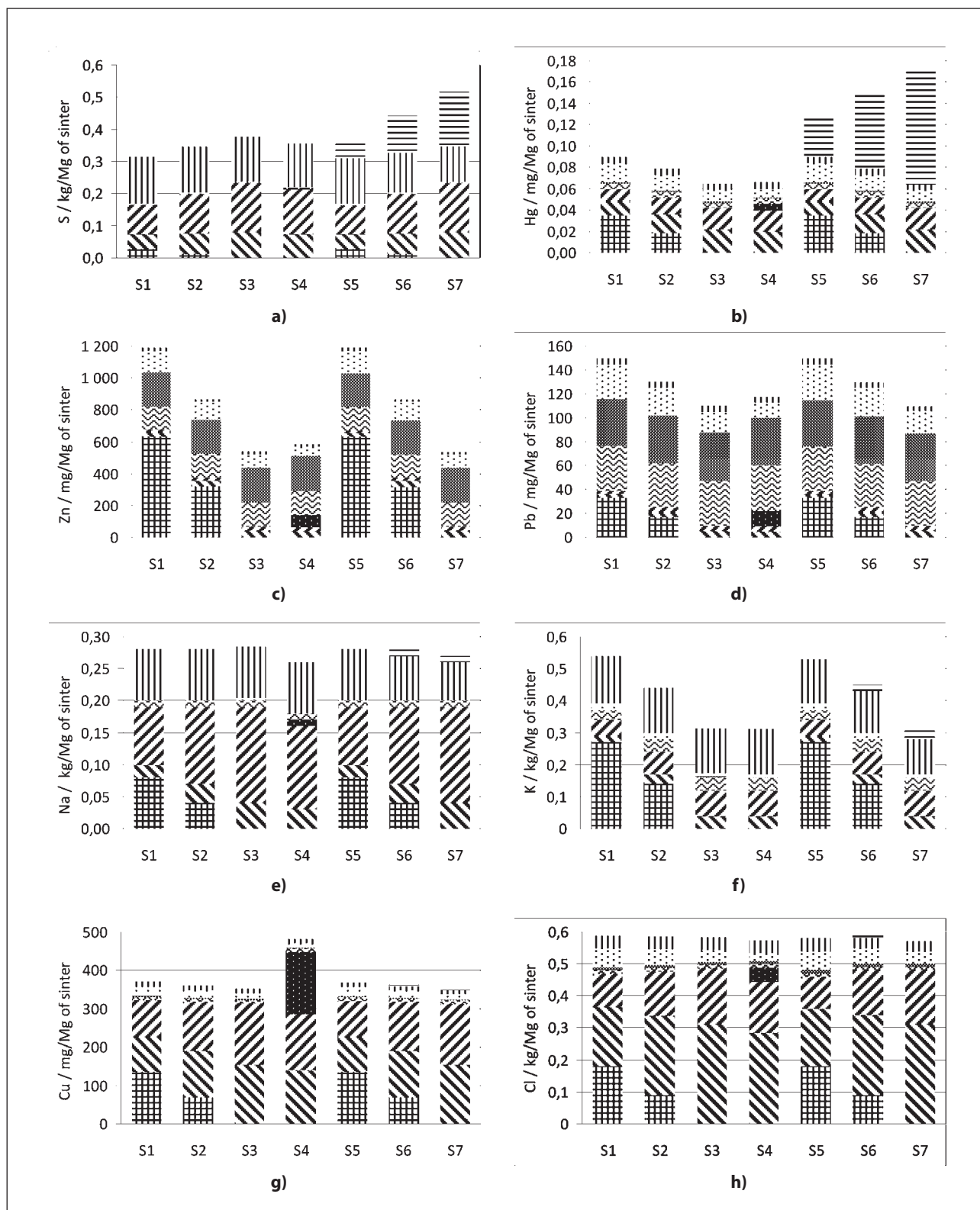
Figure 2 Content of main harmful admixtures in the studied sinter mixtures (a) S, (b) Hg, (c) Zn (d) Pb, (e) Na, (f) K, (g) Cu, (h) Cl
