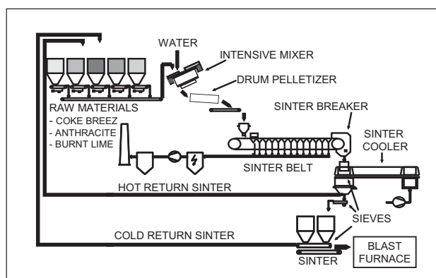
Figure 1 Sinter mixture preparation concept
