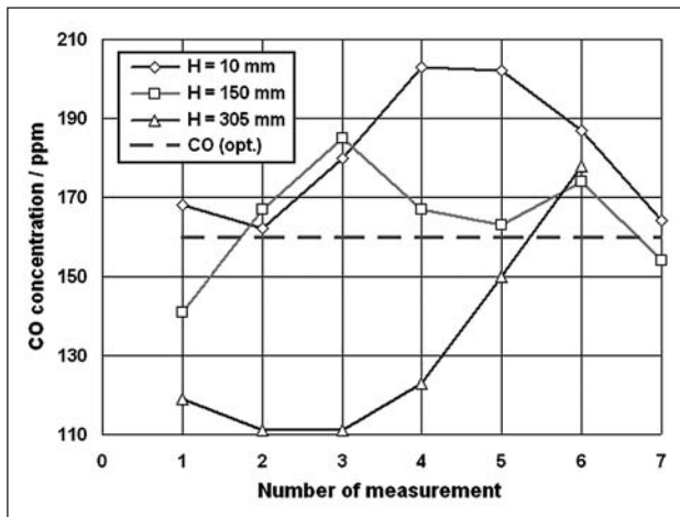
Figure 4 Distribution of CO concentration in the hood with all technological windows opened
