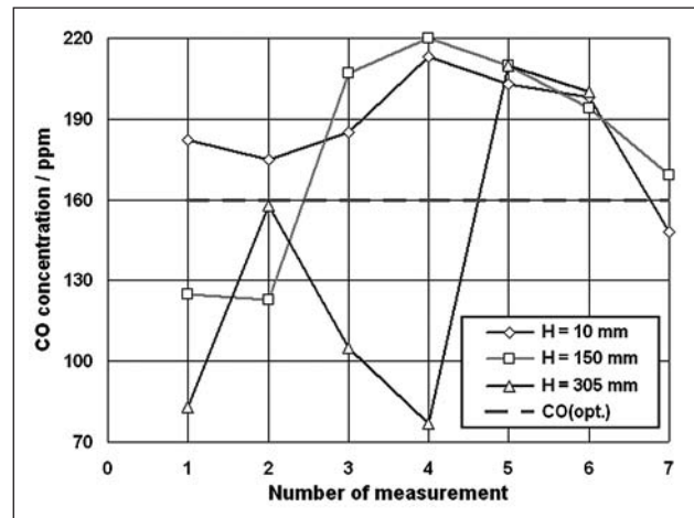
Figure 6 Distribution of CO concentration in the hood with the II and III windows opened and the I and IV windows closed
