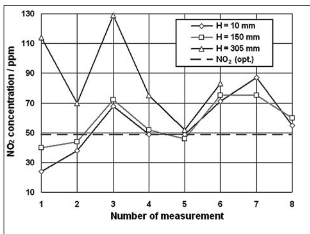
Figure 7 Distribution of NO 2 concentration in the hood for the two-outlet channel variant
