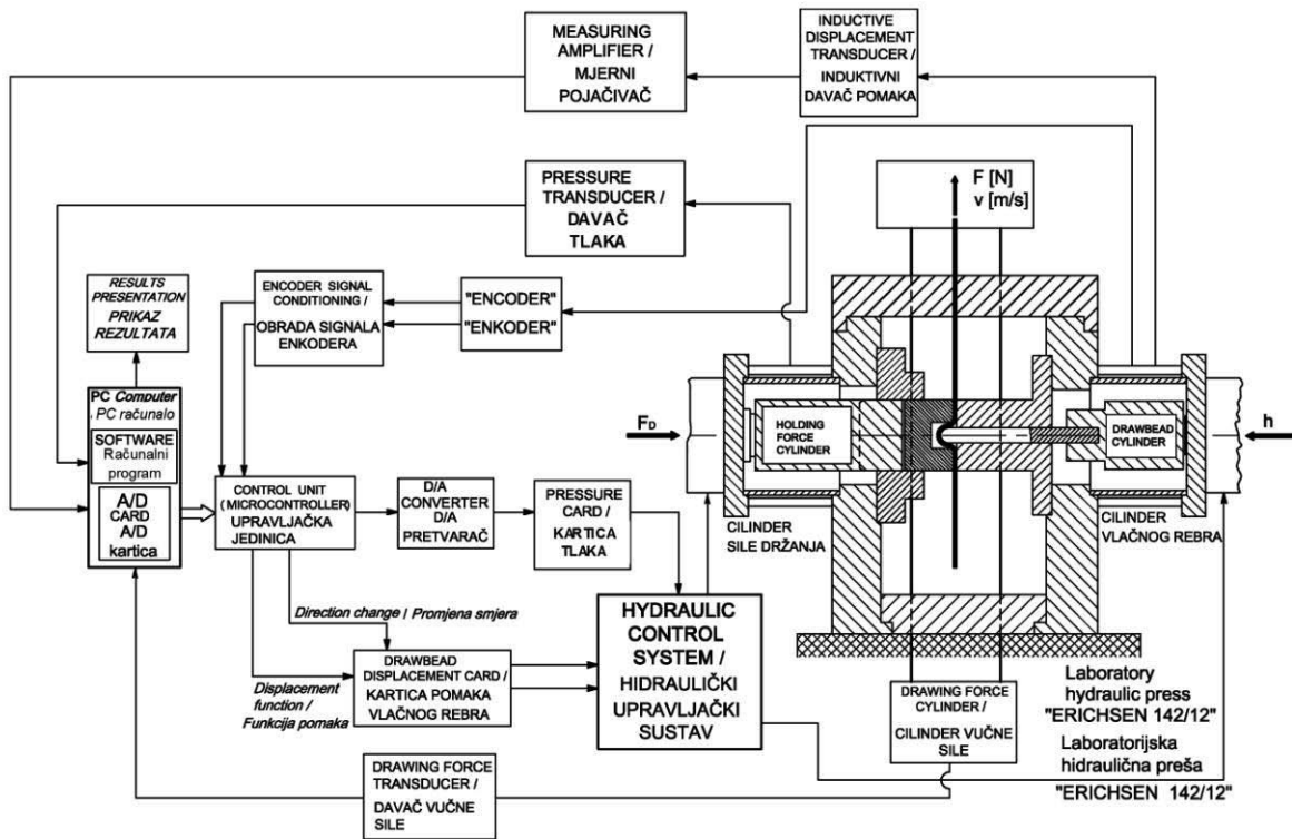
Figure 2. Block scheme of experimental apparatus
