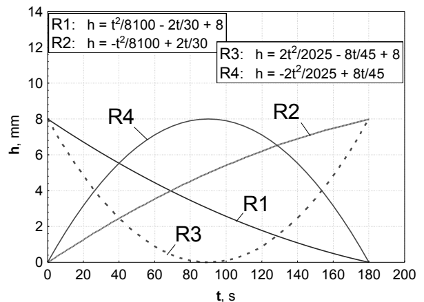
Figure 9. Drawbead height dependencies on time
