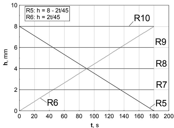
Figure 10. Drawbead height dependencies on time
