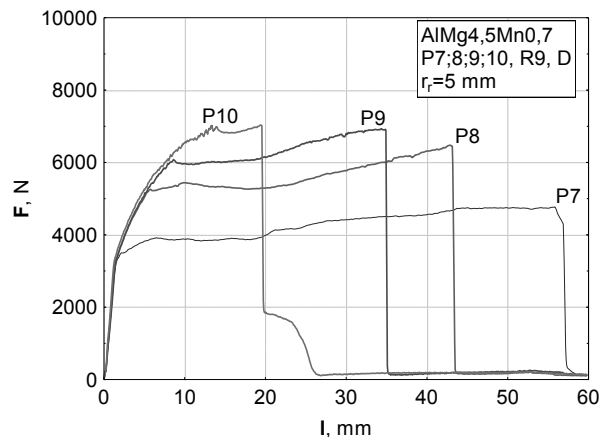
Figure 13. Drawing force dependencies on stripe travel
