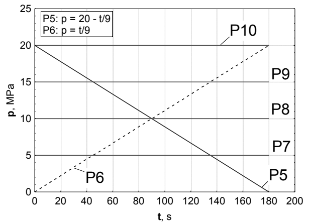
Figure 8. Contact pressure dependencies on time
