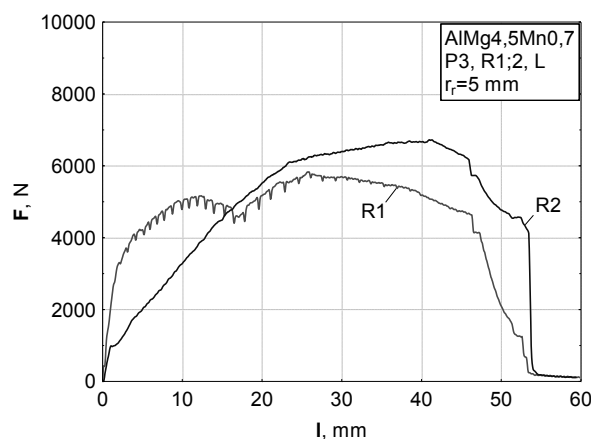
Figure 16. Drawing force dependencies on stripe travel
