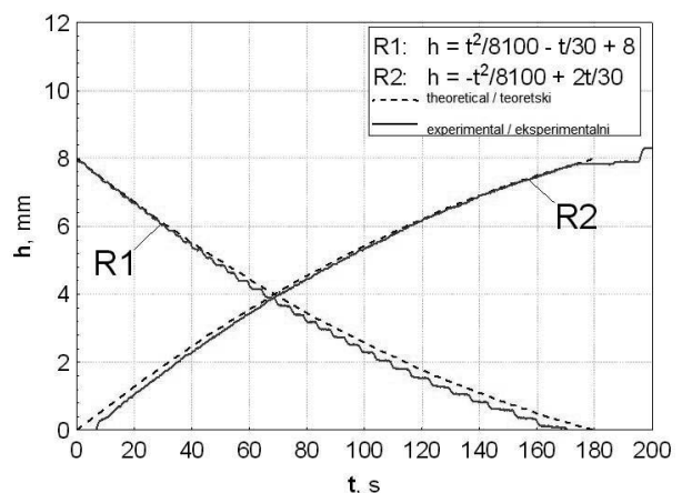
Figure 12. Given and real drawbead height dependencies on time
