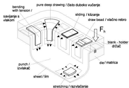
Figure 1. Scheme of physical models at deep drawing of complex geometry parts
