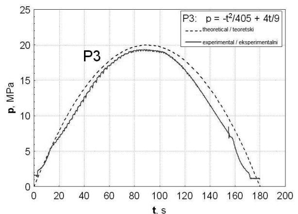
Figure 11. Given and real pressure dependence on time
