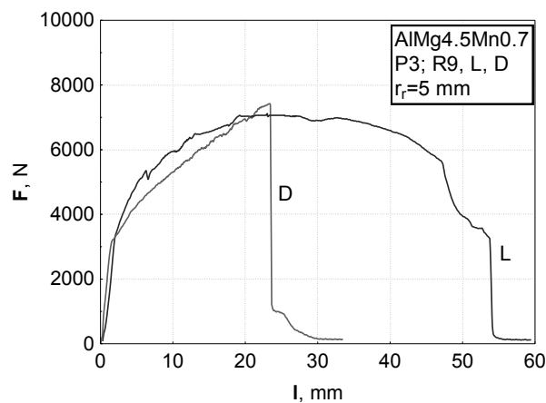
Figure 14. Drawing force dependencies on stripe travel
