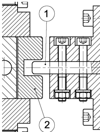
Figure 3. Scheme of drawbead
