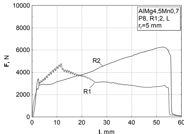
Figure 15. Drawing force dependencies on stripe travel
