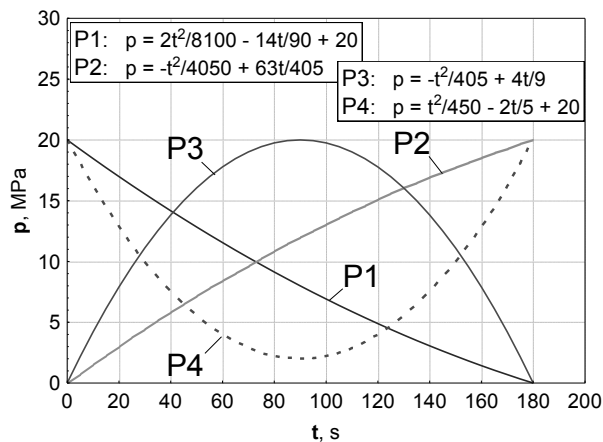
Figure 7. Contact pressure dependencies on time
