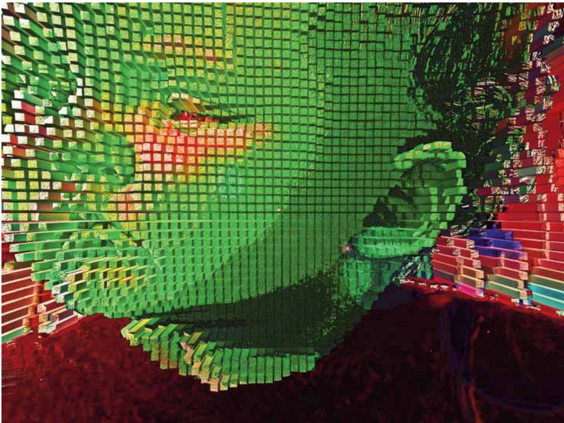
Setter: Levels
