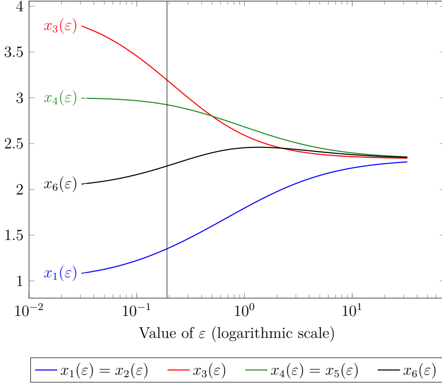
Figure 3: Generalized degrees of Example 3
