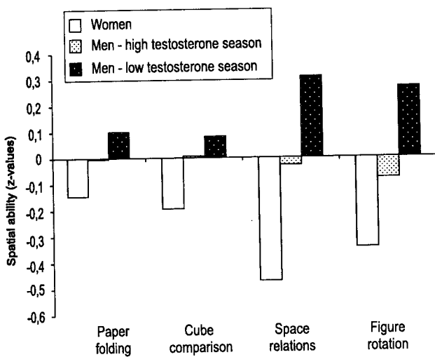
Figure 1. Average scores on four different spatial ability tests in groups with different presumed testosterone levels
