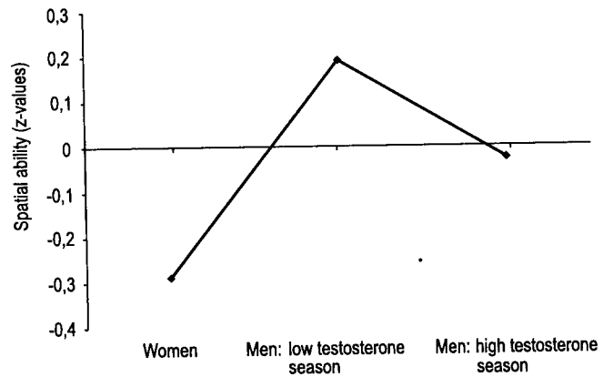
Figure 2. Composite measure of spatial ability in groups with different presumed testosterone levels
