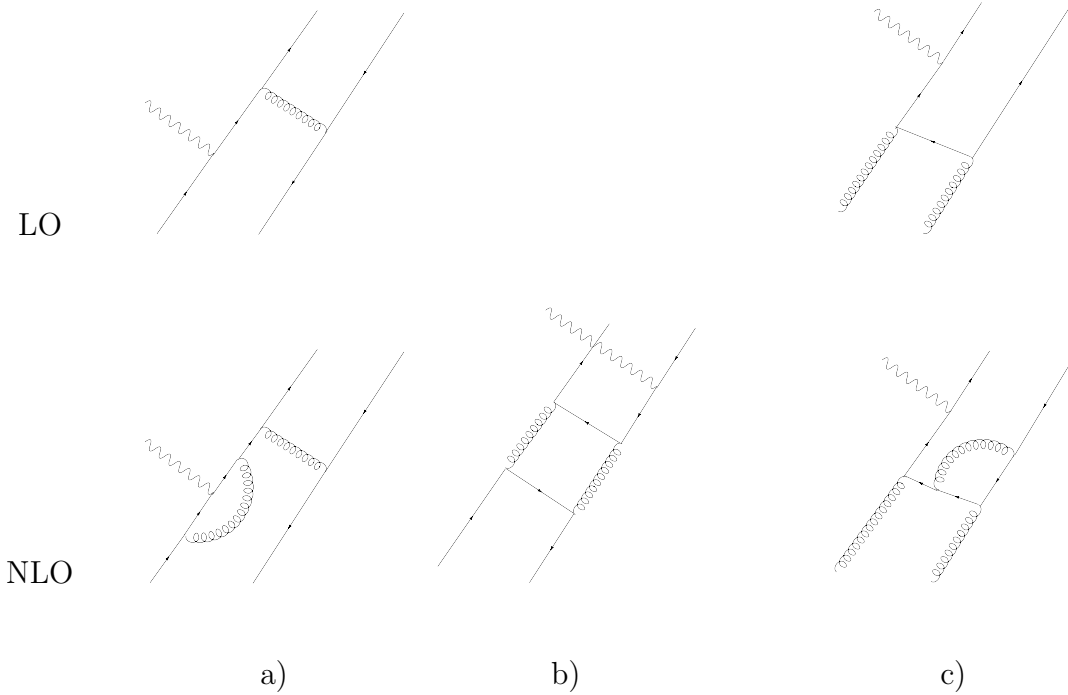
Figure 2: Representative partonic subdiagrams that contribute to DVMP of neutral vector mesons. In context of the GPD part, i.e., partons coming from the proton, (lower "legs", while the upper ones denote the meson) the contributions are organized as: a) quark contribution b) pure singlet quark contribution c) gluon contribution.
