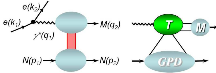
Figure 1: DVMP process from the t -channel view (left) and partonic view (right).
