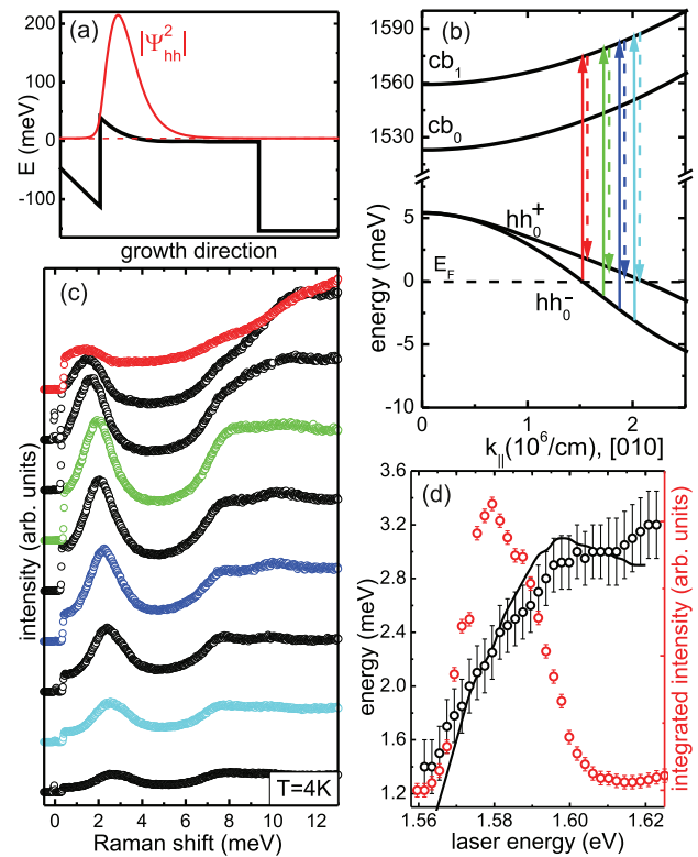
Figure 9 (a) Valence-band potential profile calculated for sample hA. (b) Spin-split dispersion of the hh_0 subband and the lowest conduction band subbands. (c) Series of depolarized \tilde{z}([010], [100])\tilde{z} RILS spectra for different laser energies from 1.567 to 1.600 eV (top to bottom spectra). Spectra are taken at nominally T = 4 K, at resonance with the cb_1 conduction-band subband. (d) Experimental mode positions and integrated intensities of the low-energy SDE. Reprinted with permission from Ref. [37].
