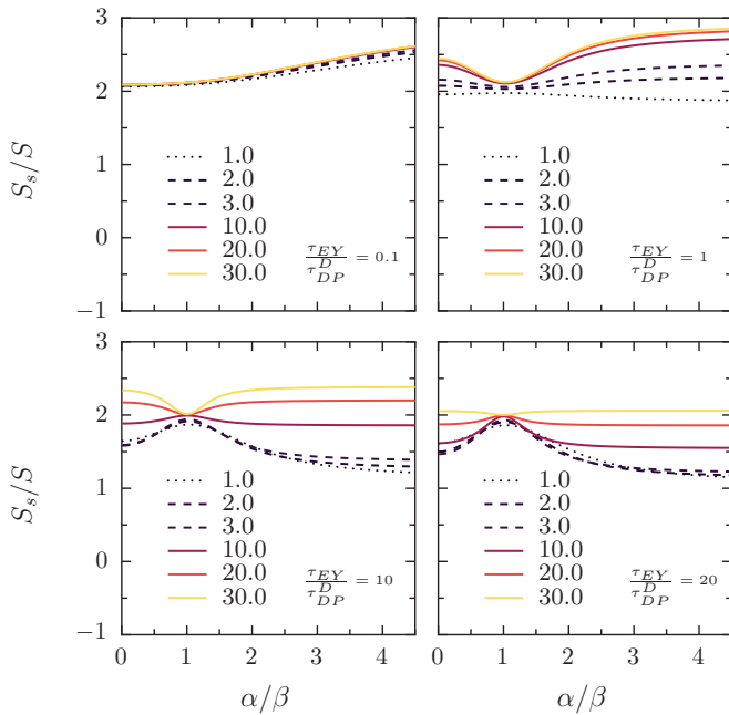
FIG. 1. (Color online) The spin thermopower S_s of a disordered 2D-electron gas with numerous competing SO mechanisms. Typical values for GaAs quantum wells are mobility \mu = 10^4 \text{ cm}^2/\text{Vs} , density n = 10^{12} \text{ cm}^{-2} , effective extrinsic wavelength \lambda_0 = 4.7 \times 10^{-8} \text{ cm} , and Dresselhaus coupling constant \hbar\beta = 10^{-12} \text{ eV}\cdot\text{m} . There follows \gamma_{\text{ss}} \gg \gamma_{\text{intr}}, \gamma_{sj} , \tau_{\text{EY}} \gg \tau_{\text{DP}}^D . The Rashba coupling constant can be modulated by the gate potential. 40,41 Each panel shows the ratio S_s/S as a function of the ratio \alpha/\beta for a given Elliot-Yafet scattering strength, strong to weak from top left to bottom right—panel 3 corresponds to standard GaAs. Magnetic scattering is strongest for the dotted curve, \tau_{sf}/\tau_{\text{DP}}^D = 1 , and strong (weak) for the dashed (solid) curves, \tau_{sf}/\tau_{\text{DP}}^D = 2, 3 (10, 20, 30).
