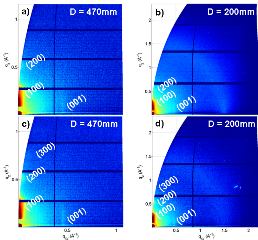
Figure 4.3: a-b) 2D-GIXRD images of \sim 1 ML of N2200 at sample-detector distance D = 470 mm and D = 200 mm respectively; c-d) 2D-GIXRD images of \sim 1 ML of N2200 after annealing at 150^\circ\text{C} overnight in vacuum oven at sample-detector distance D = 470 mm and D = 200 mm respectively. The logarithmic scale of colours is the same for all the images as well as the incident angle \alpha_i = 0.18^\circ .
