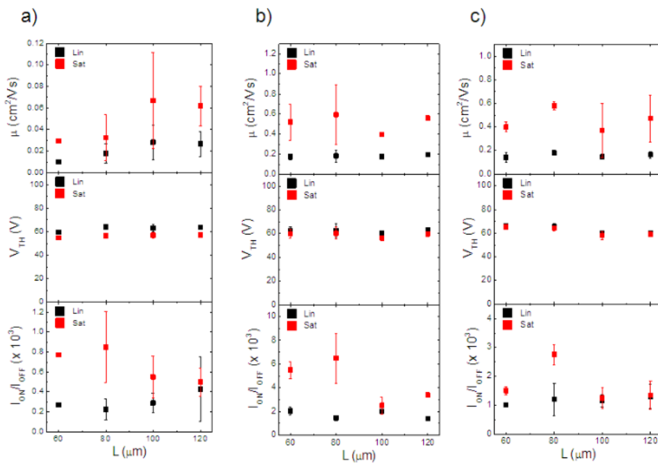
Figure 4.9: Electrical results of a) \sim 1 ML, b) \sim 2 MLs and c) \sim 3 MLs of N2200 thin-films deposited by LS technique on OTS-treated substrate and annealed at 150 °C overnight in vacuum oven.
