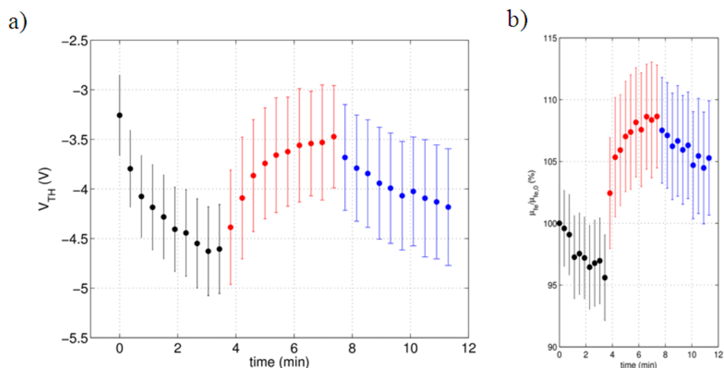
Figure 5.4: a) V_{TH} and b) \mu values vs time. Color legend: black before, red during, blue after X-ray exposure.
