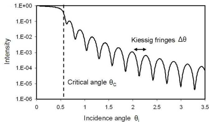
Figure 2.7: Example of Kiessig fringes in XRR measurements
