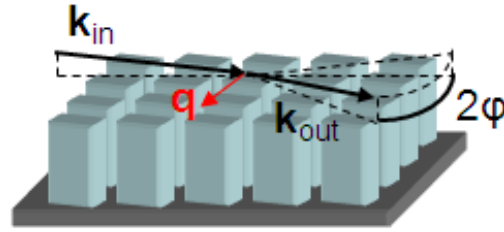
Figure 2.14: Sketch of GIXRD measurement: the scattering vector probes the distance between lattice planes almost parallel to the surface normal.
