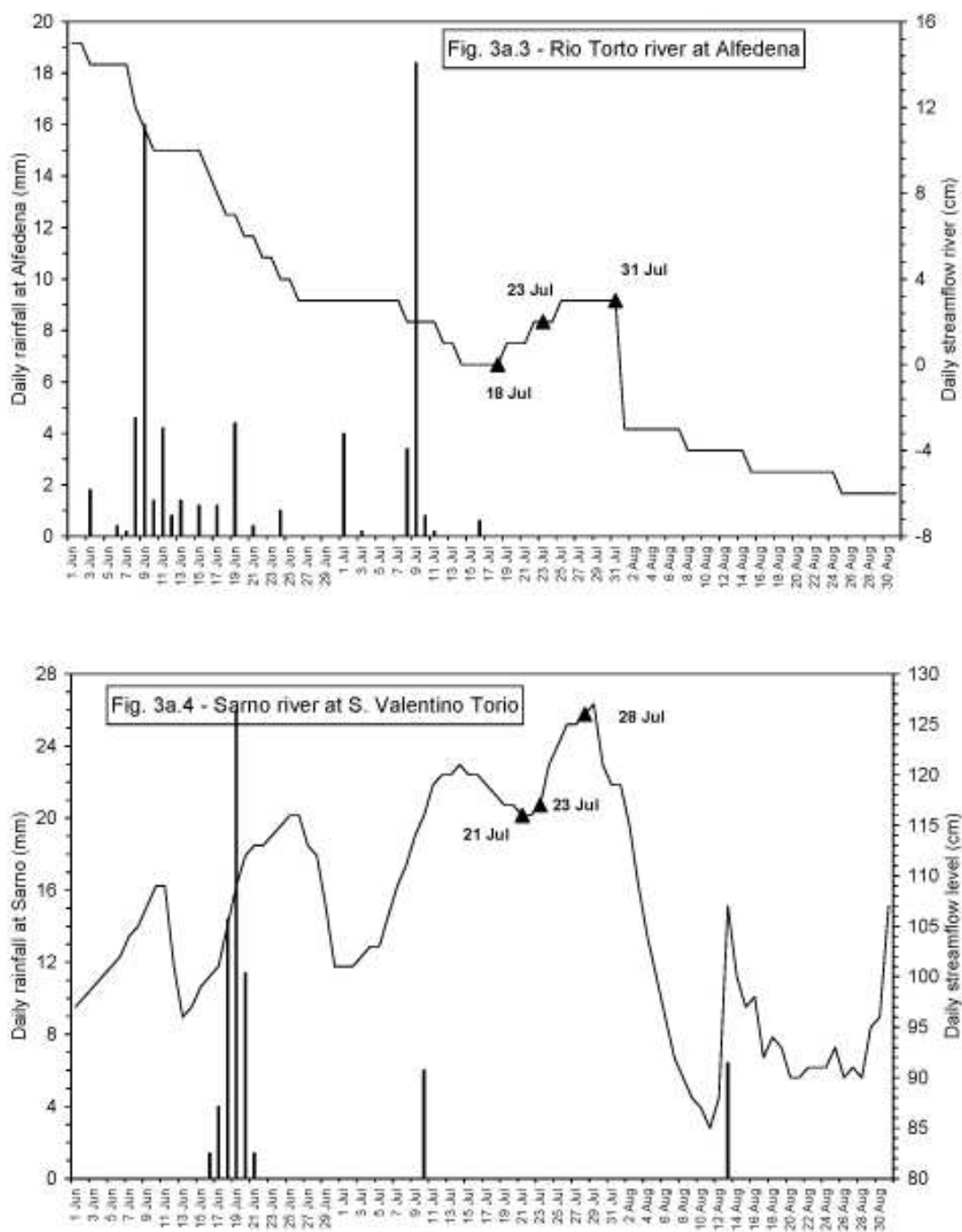
Fig. 3a – Hydrological changes in rivers correlated to the 23 July 1930 earthquake. Black bars indicate rainfalls (left scale).
