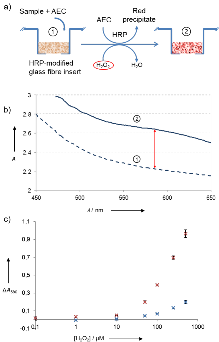
Figure 4. a) Biosensor configuration for H 2 O 2 detection based on the enhanced absorbance measurement of the catalytic conversion of HRP co-substrate, AEC, into an insoluble reddish product. Clean glass fibre inserts are modified with HRP and washed several times prior to experiments. b) The production of red precipitate in the presence of H 2 O 2 induces an increase in the measured absorbance ( A_{\max} = 580 \text{ nm} ). c) Calibration curves were performed using 0.6 nmol of HRP (25 \mu\text{L} of 1 \text{mg}\cdot\text{mL}^{-1} solution) either (blue) directly in acetate buffer solution (no insert) or (red) crosslinked into a glass fibre enhancer insert, and exposed to varying concentrations of H 2 O 2 (1 to 500 \mu\text{M} contained in 100 \mu\text{L} sample) in the presence of AEC (142 nmol). The graphs indicate a significant improvement of the biosensor analytical performances in the case of HRP-modified enhancer insert. Response times: 15 and 5 minutes for solution assay and insert-based biosensor, respectively. Error bars indicate the calculated standard deviation ( n=3 ).
