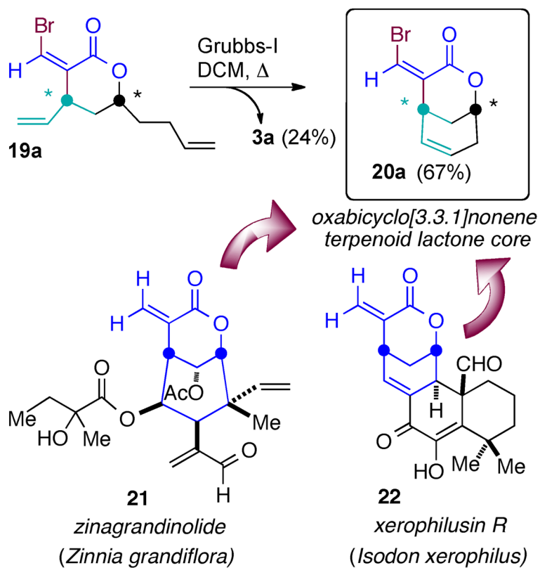
Scheme 5. Isomerization-RCM: Oxabicyclo[3.3.1]nonyl Cores of Zinagrandinolide/Xerophilusin R
