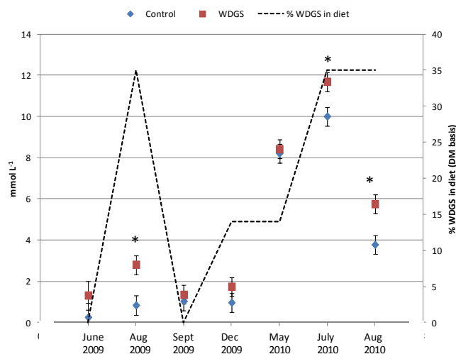
Figure 1. \text{NH}_3 concentration in air samples collected from surface of feedlot pens with cattle fed diets containing corn wet distillers grains with solubles (WDGS) or a dry-rolled corn diet with no WDGS (Control). Asterisks represent a significant difference in ammonia concentration due to dietary treatment, on a given date. The line represents dietary inclusion rate of WDGS. Each sampling period consists of 60 samples collected from pens with cattle fed WDGS and 60 samples from pens with cattle fed Control diets ( N = 840 ).
