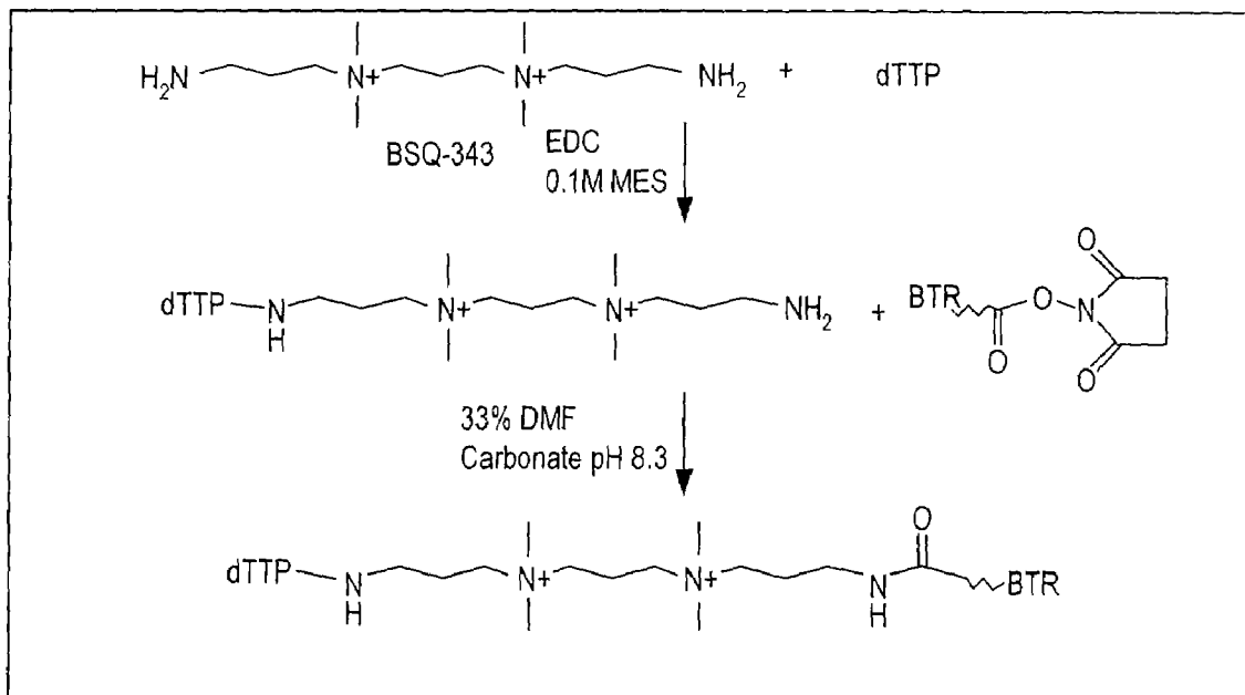
Scheme 6
