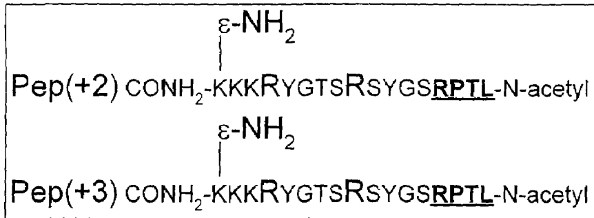
Scheme 7 - Peptide linkers (shown in C-to-N direction)
