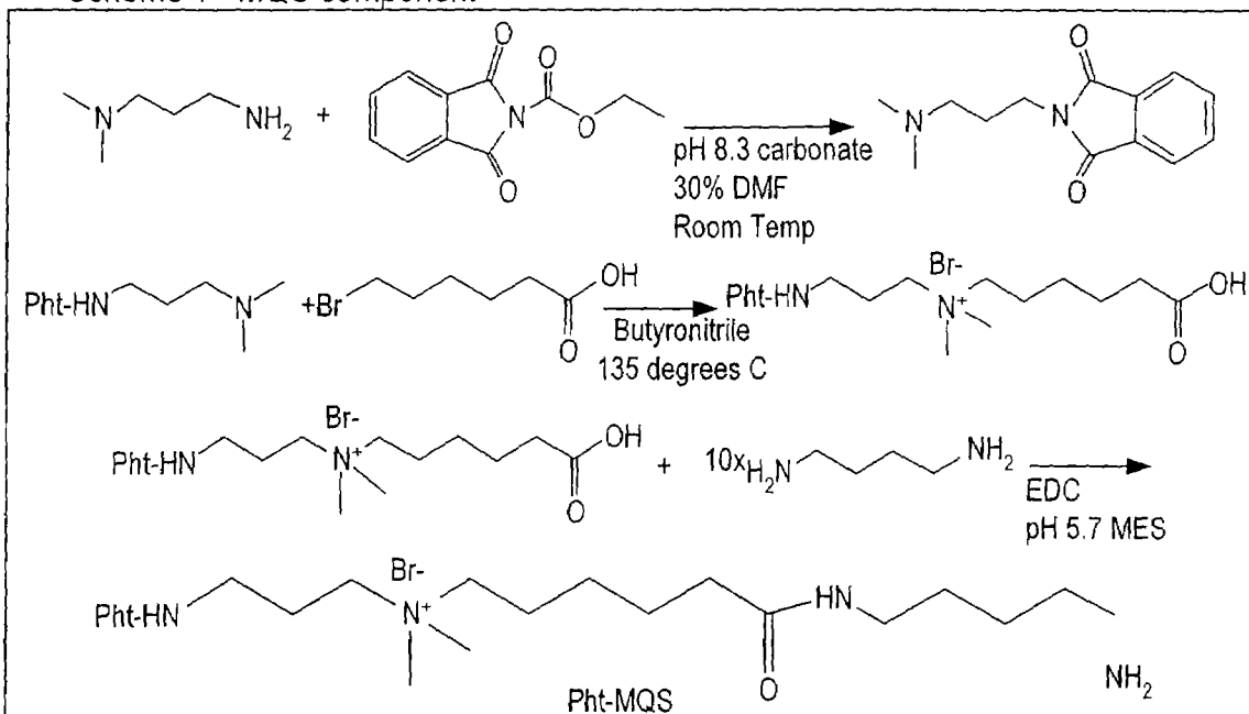
Scheme 2 - BQS linker
