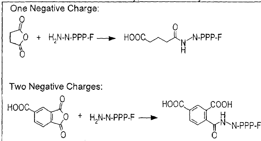
Scheme 10 - g-dNTP With Carboxylated Base
