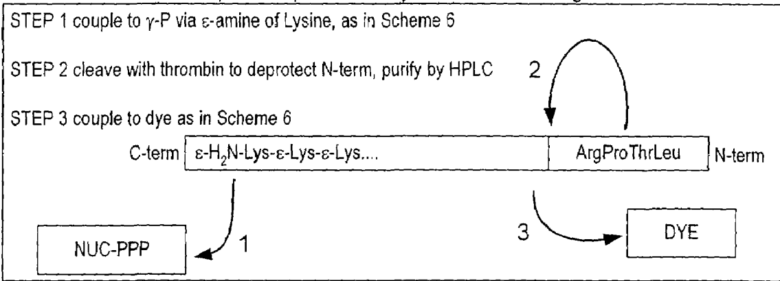
Scheme 8 - Peptide Deprotection By Thrombin Cleavage
