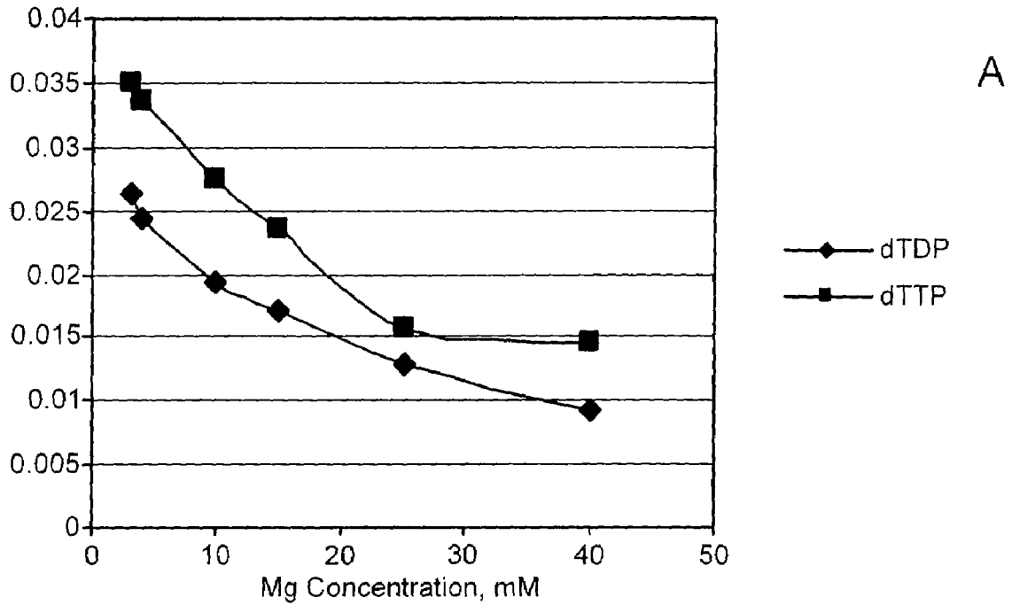
Mg ++ Controls Electrophoretic Mobility of Nucleotides
