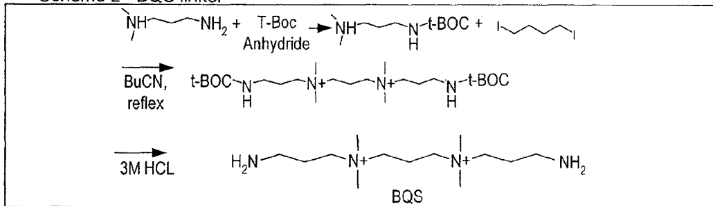
Scheme 3 - TQS linker
