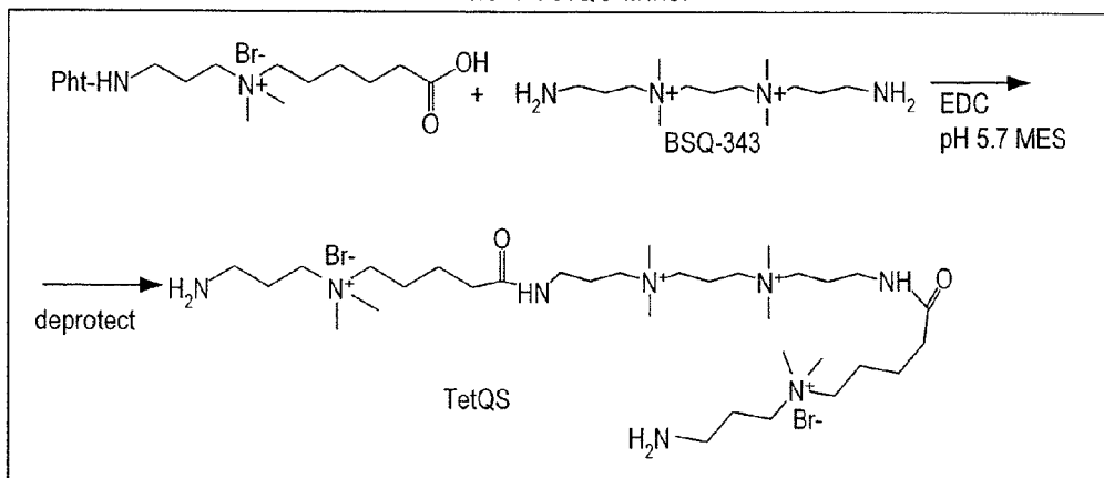
Scheme 4 TetQS linker
