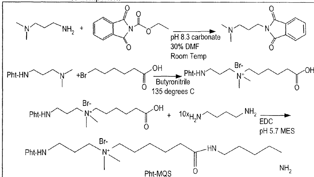
Scheme 2 - BQS linker
