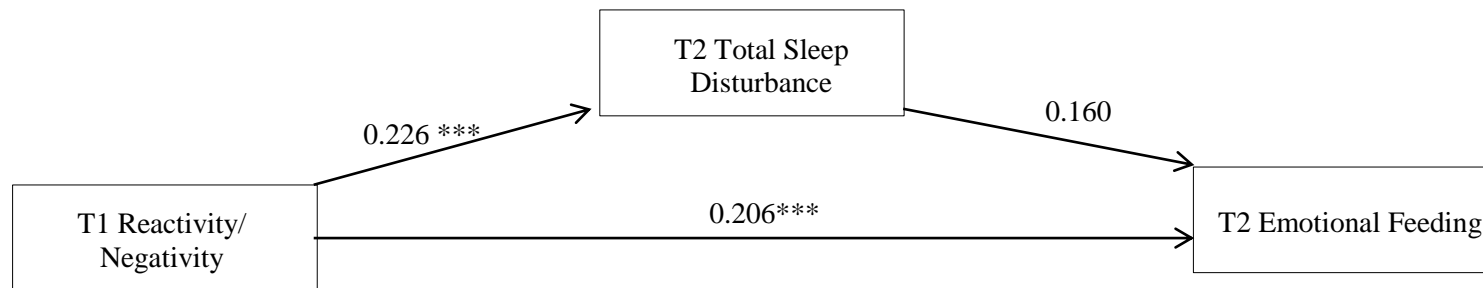
Figure 4. Exploratory Model 2: Direct and indirect relationship among T1 Reactivity/Negativity, T2 Total Sleep Disturbance, and T2 Emotional Feeding
