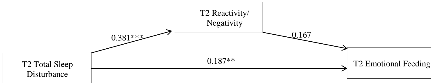
Figure 5. Exploratory Model 3: Direct and indirect relationship among T2 Total Sleep Disturbance, T2 Reactivity/Negativity, and T2 Emotional Feeding
