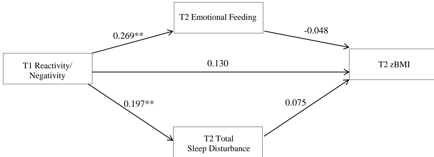
Figure 2. Final longitudinal analysis model
