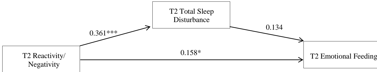
Figure 3. Exploratory Model 1: Direct and indirect relationship among T2 Reactivity/Negativity, T2 Total Sleep Disturbance, and T2 Emotional Feeding
