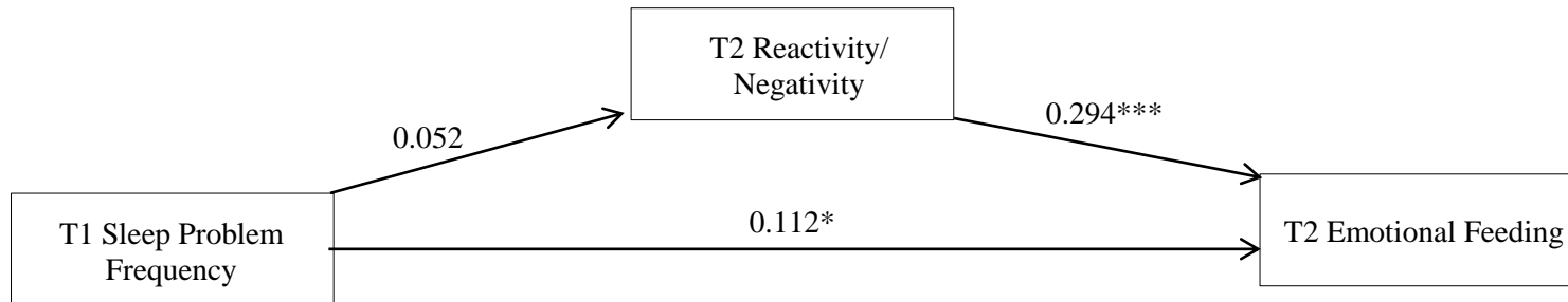
Figure 6. Exploratory Model 4: Direct and indirect relationship among T1 Sleep Problem Frequency, T2 Reactivity/Negativity, and T2 Emotional Feeding
