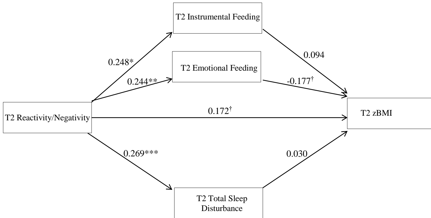
Figure 1. Final concurrent analysis model
