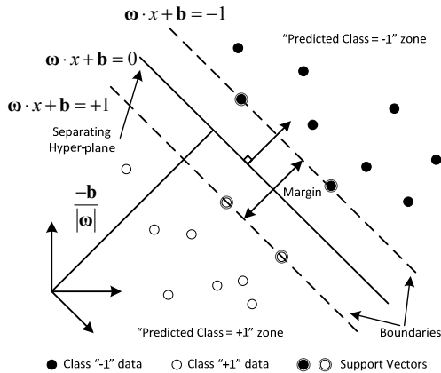
Fig. 3. SVM classification.
