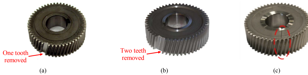
Fig. 10. The test gears with (a) one-tooth-missing, (b) two-tooth-missing, and (c) gear crack.
