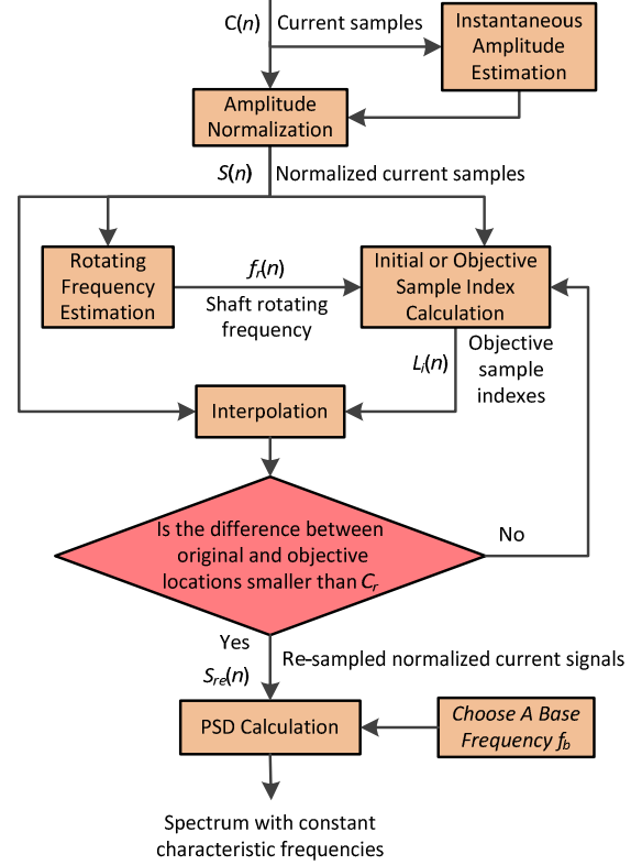
Fig. 2. Schematic of the adaptive signal resampling algorithm.
