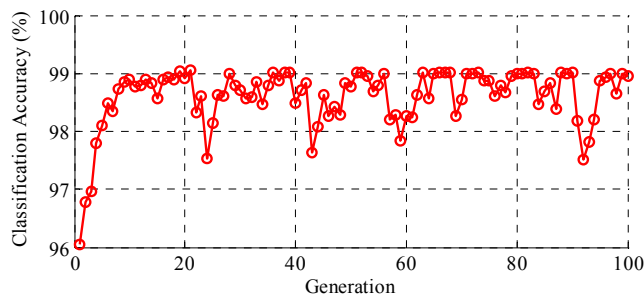
Fig. 11. Classification accuracy of the GA-SVM hybrid classifier over generations.
