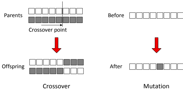
Fig. 6. The crossover and mutation operations.
