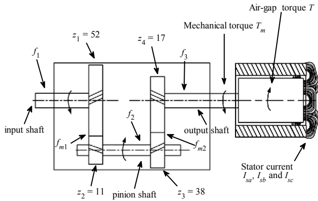
Fig. 9. Structure of the test drivetrain consisting of a two-stage gearbox connected to a PMSG with characteristic vibration frequencies.
