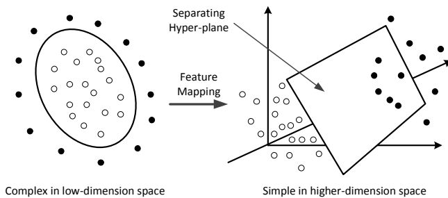
Fig. 4. Feature mapping by using the kernel function.
