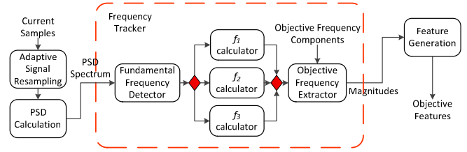
Fig. 1. Schematic diagram of the feature extraction scheme.
