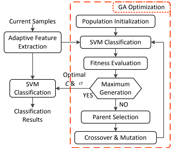
Fig. 7. The proposed GA-SVM hybrid classifier.
