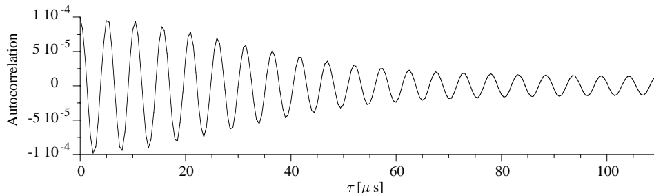
FIG. 2. Autocorrelation of the Doppler signal.
