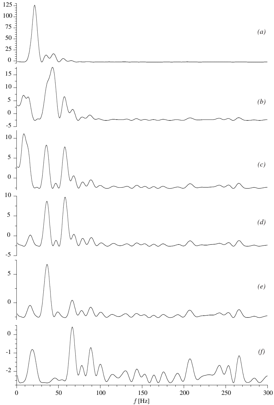
FIG. 4. Plot of \log_{10} P(\omega|\mathbf{e}, \mathcal{J}) as given by (19) for the Doppler signal obtained from the 128 \mu\text{s} window vs. f ( \omega = 2\pi f ): (a) for the original signal; (b) for the residual after the removal of the dominant frequency in (a). Each of the remaining panels shows probability after removing the dominant frequency of the previous panel.
