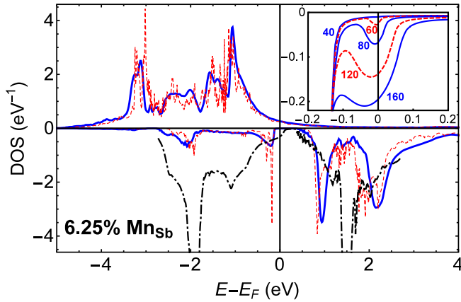
FIG. 4. (Color online) Partial DOS for \text{Mn}_{\text{Sb}} in NiMnSb with a 6.25% occupation of the Sb site by Mn, parallel spin alignment. Solid (blue) lines: CPA; dashed (red) lines: VASP. Black dotted-dashed line: Total minority-spin DOS per formula unit ( N_{\downarrow} ), disordered spin of \text{Mn}_{\text{Sb}} . Inset: N_{\downarrow} at 40, 60, 80, 120, and 160 K as labeled (same units on axes).
