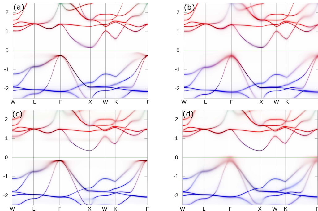
FIG. 5. (Color online) Minority-spin spectral function in NiMnSb with 6.25% of (a), (b) \text{Mn}_{\text{E}} and (c), (d) \text{Mn}_{\text{Sb}} . The spins of \text{Mn}_{\text{E}} are (a) antiparallel to magnetization and (b) randomly oriented. The spins of \text{Mn}_{\text{Sb}} are (c) parallel to magnetization and (d) randomly oriented. Coloring is similar to Fig. 1(a); \text{Mn}_{\text{E}} added to Mn (red), \text{Mn}_{\text{Sb}} to Sb (green). Energy is in eV measured from E_F .
