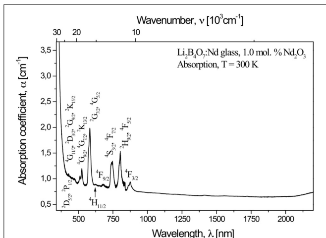
FIGURE 2 | The optical absorption spectrum of \text{Nd}^{3+} centers in \text{Li}_2\text{B}_4\text{O}_7\text{:Nd} glass.
