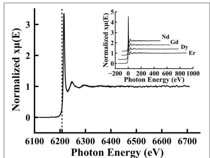
FIGURE 4 | X-ray absorption fine structure spectrum of \text{Li}_2\text{B}_4\text{O}_7\text{:Nd} .
