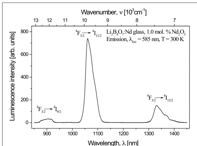
FIGURE 3 | The luminescence emission spectrum of \text{Nd}^{3+} in \text{Li}_2\text{B}_4\text{O}_7\text{:Nd} glass.
