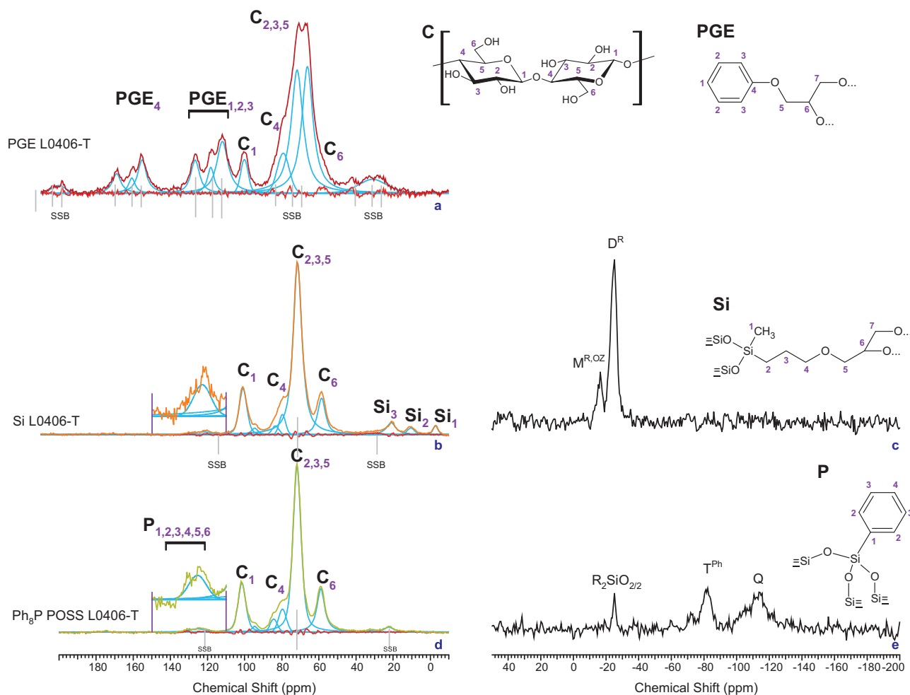
Fig. 10. 13 C and 29 Si NMR using the CPMAS and MAS methods for cellulose control samples, PGEL0406-T, Si-L0406-T, and Ph8P-L0406-T, conducted by our collaborators at Dow Corning.
