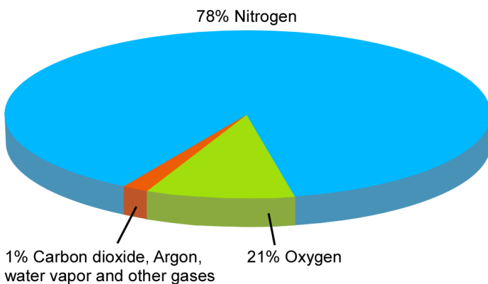
Figure 4.2. Composition of the earth's atmosphere.
