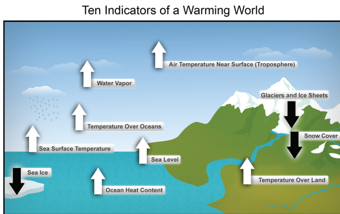
Figure 3.1. These are just some of the indicators measured globally over many decades that show that the earth's climate is warming. White arrows indicate increasing trends, and black arrows indicate decreasing trends. All the indicators expected to increase in a warming world are, in fact, increasing, and all those expected to decrease in a warming world are decreasing. (Source: Walsh et al., 2014)
