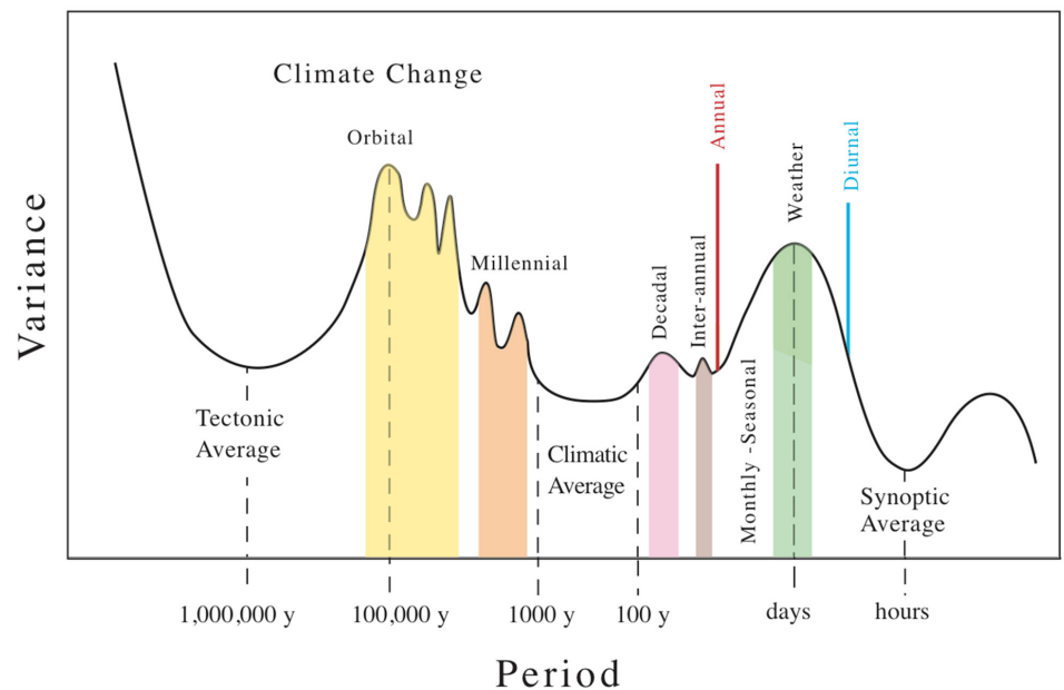
Figure 2.1. The classic spectrum of climate change. Note that variability occurs on all time scales, but to a greater or a lesser degree. (Source: K. Maasch, University of Maine)
