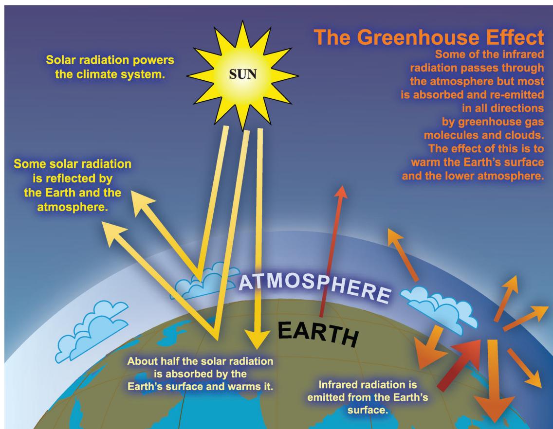
Figure 2.2. The greenhouse effect. (Source: Le Treut et al., 2007)
