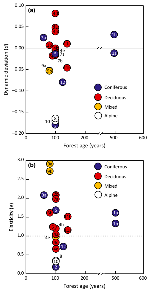
Fig. 8 Catchment properties as a function of forest type (colored circles) and forest age: (a) dynamic deviation d and (b) elasticity e . Key to site IDs (the numbers within the circles) is given in Table 1. (Color in the online version)
