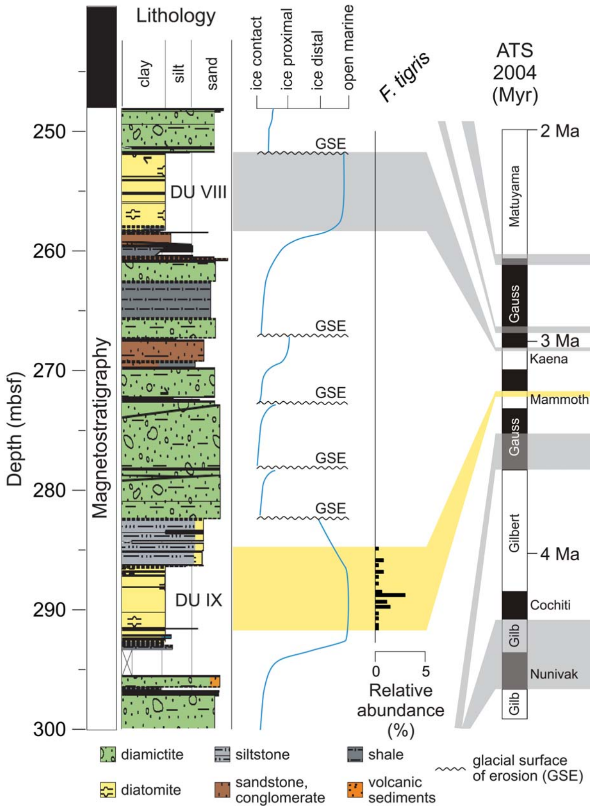
TEXT-FIGURE 2 Summary of the AND-1B core from 248-300 mbsf. Magnetostratigraphy after Wilson et al. (2007). Lithostratigraphy after Krisek et al (2007). Glacial proximity curve after Naish et al. (2009); grounding line advances for five glacial/interglacial cycles are identified by glacial surfaces of erosion. Fragilariopsis tigris is only identified from DU IX. The bold yellow field marks the position of DU IX within the astronomically tuned timescale of (ATS) of Gradstein et al. (2004). Pale grey fields mark the ages of AND-1B diatomites from which F. tigris is absent (Winter et al. 2012). Full color version is available online at micropress.org
