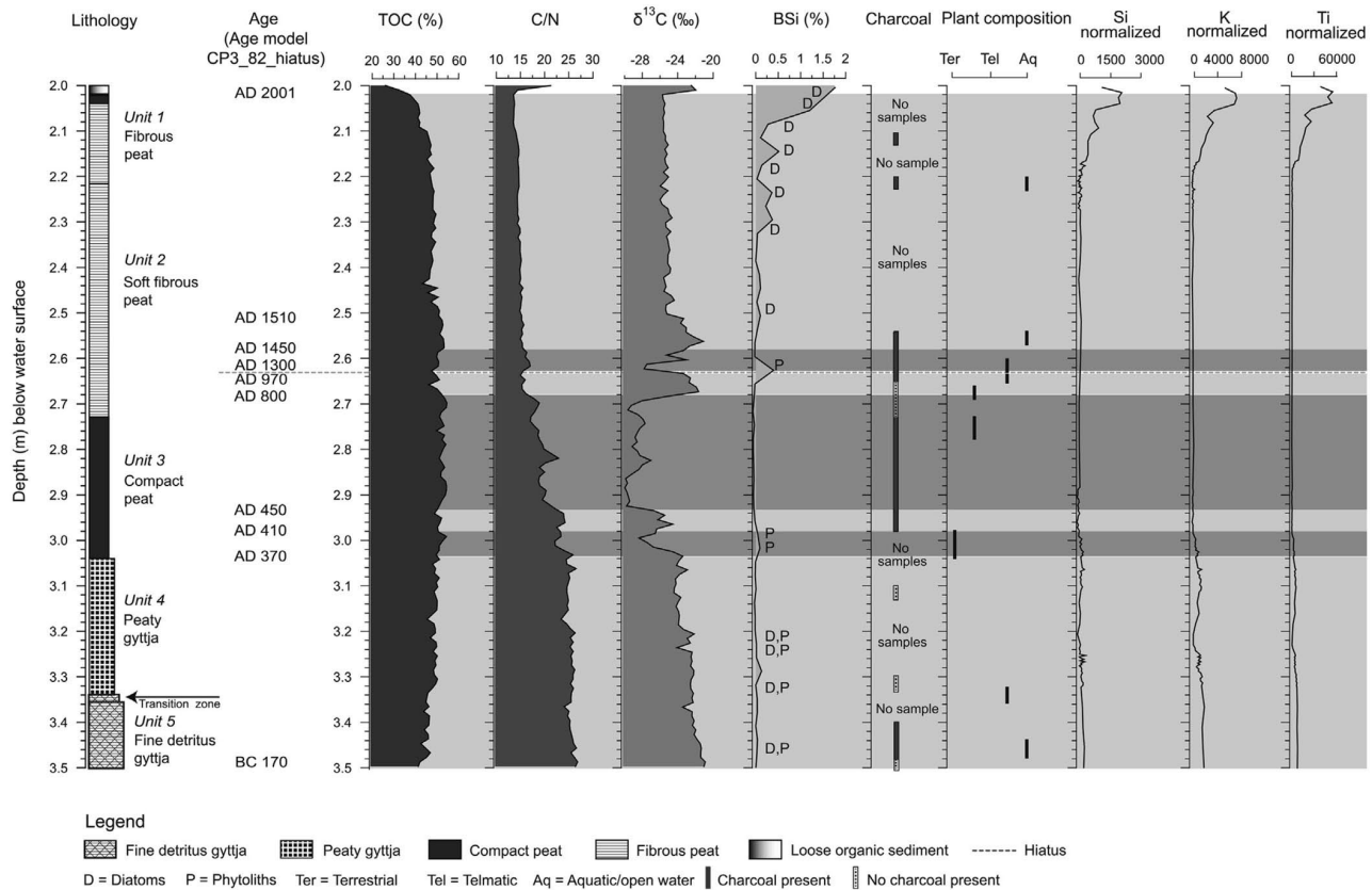
Figure 3. Lithostratigraphy, geochemistry, and selected elemental data for CP3. The samples analyzed for diatoms, phytoliths, charcoal, and plant macrofossil composition are discontinuous (see text for further explanations). Light gray bars represent higher effective moisture, and the dark gray bars represent lower effective moisture.
