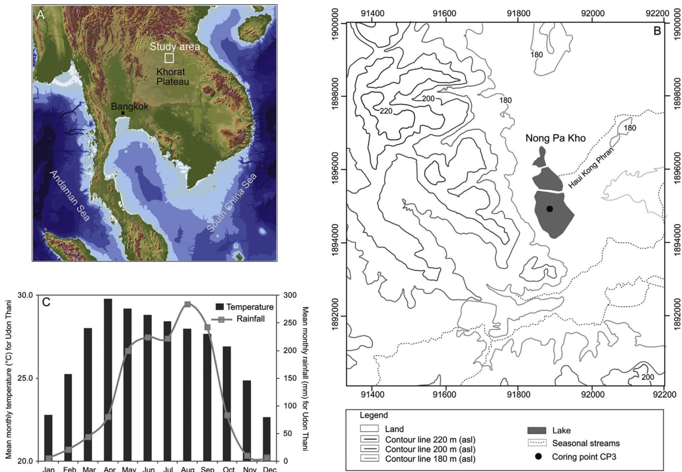
Figure 1. (A) Location of the study area in northeast Thailand. (B) Topography around Nong Pa Kho and the location of coring point CP3. The coordinate system is based on the UTM Grid system (WGS 1984 zone 48; asl = above sea level). (C) Mean monthly rainfall and temperature (1962–2011) for Udon Thani, which is situated 36 km NW of Pa Kho. Map (A) was generated using the generic mapping tools-GMT ( http://gmt.soest.hawaii.edu/ ), and map (B) was redrawn based on aerial photographs before and after 1994 using the data set in Klubseang (2011).
