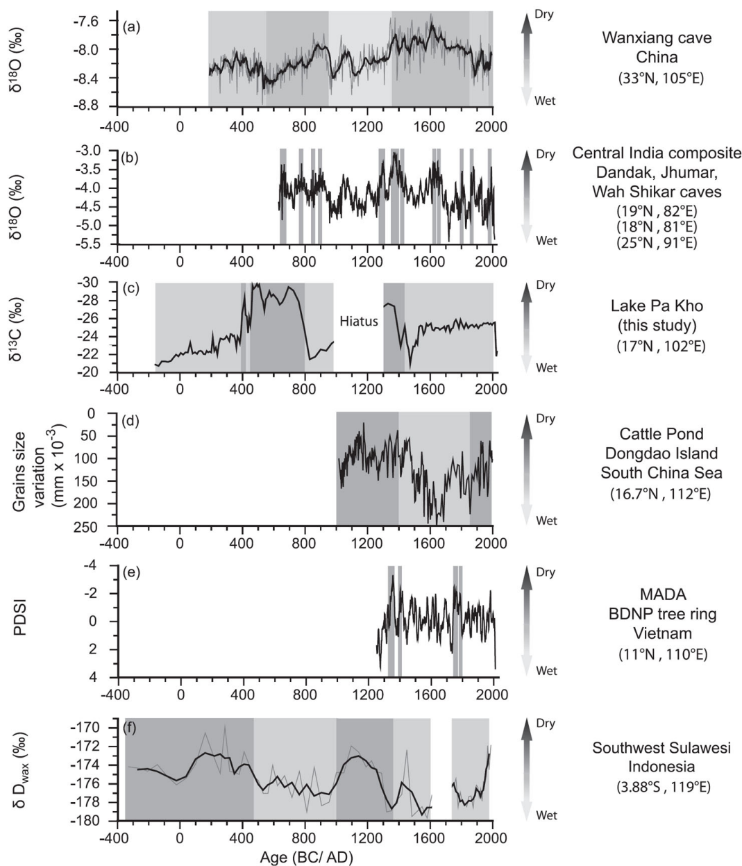
Figure 4. Selected high-resolution records for the Asian monsoon region for the past 2000 years: (a) \delta^{18}\text{O} data of Wanxiang Cave speleothems (Zhang et al., 2008); (b) Composite \delta^{18}\text{O} time series for central India based on speleothems from Dandak, Jhumar, and Wah Shikar Caves (Berkelhammer et al., 2010; Sinha et al., 2011a, 2011b, 2007); (c) \delta^{13}\text{C}_{\text{org}} data from Lake Pa Kho (this study); (d) grain size variations in sediment core DY6-MGS of Cattle Pond, Dongdao Island (Yan et al., 2011); (e) Palmer Drought Severity Index (PDSI) derived from the Monsoon Asia Drought Atlas (MADA) for the region between 10 and 20°N and 95–115°E (Buckley et al., 2007, 2010, 2014; Cook et al., 2010; D'Arrigo et al., 2011; Sano et al., 2009); (f) \delta\text{D}_{\text{wax}} from marine cores 31 MC and 34 GGC from southwest Sulawesi (Tierney et al., 2010). The vertical light gray bars represent higher effective moisture/a strengthened summer monsoon, and the dark gray bars represent lower effective moisture/a weakened summer monsoon. Note that the timing of the shifts in moisture history of the individual records follows that cited by the respective author/s. See Figure 5 for the location of the different records.
