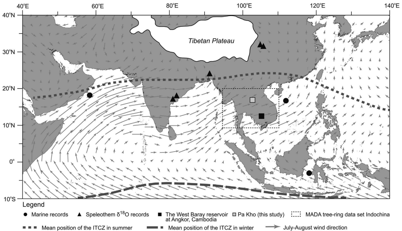
Figure 5. Location of selected high-resolution Asian monsoon paleo-records for the last 2000 years. The mean position of the winter and summer Intertropical Convergence Zone (ITCZ) is according to Wang (2009). The July–August wind directions and wind speeds follow Wang et al. (2003). Long arrows indicate high wind speed and short arrows lower wind speed.
