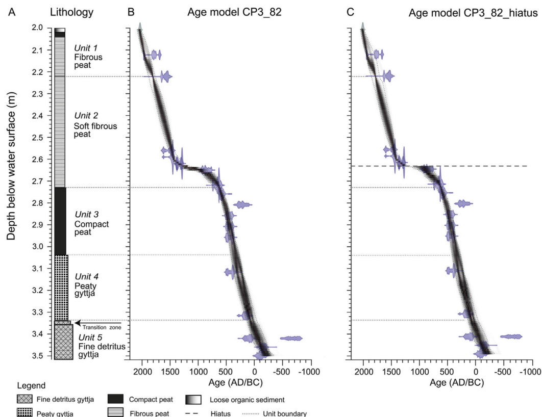
Figure 2. (A) Lithostratigraphy for CP3, (B) age model CP3_82 and (C) age model CP3_82_hiatus. The blue shapes show the calibrated ^{14}\text{C} dates with two standard deviations, the grey shading indicates the likely age model and the dotted lines show the 95% confidence ranges of the age model. See Table 1 for a detailed description of the sequence and Table 2 for the ^{14}\text{C} dates.
