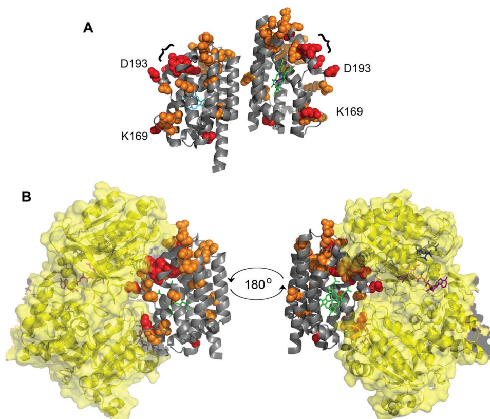
Figure 22. Interface for CPR on HO-2 defined by NMR and mutagenesis. A, residues in red have both significant CSPs and large intensity ratio changes with the addition of 75 \mu\text{M} CPR. Residues of HO-2 that have significant CSPs or large changes in peak intensity ratio with the addition of 75 \mu\text{M} CPR are shown in orange. { identifies a patch of residues strongly affected by CPR (Phe-99, Glu-102, Gln-200, Leu-201, and Tyr-202). Leu-201 and Lys-169 were identified by mutagenesis. Side chains are shown as spheres (PDB 2QPP). B, residues identified for HO-2 mapped onto the analogous residues of HO-1 in the published crystal structure of the complex of rat HO-1 (gray) and rat CPR \Delta TGEE (yellow) (PDB 3WK7). Cofactors are as indicated as follows: heme (green), NADP + (blue), FAD (orange), and FMN (purple).
