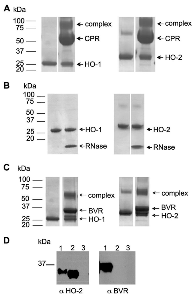
Figure 16. Chemical cross-linking of HO-2 and CPR. A, heterobifunctional cross-linker LC-SPDP stabilizes a complex between HO-1 or HO-2 and CPR. B, no complex is trapped for HO-1 or HO-2 with RNase. C, chemical cross-linking also stabilizes a complex between HO-1 or HO-2 and BVR. Cross-linking reactions contained 10 \mu m of the indicated protein. D, reducing SDS-PAGE and Western blot of HO-2 pulldown and associated BVR. Lane 1, cross-linking reaction; lane 2, HO-2 only; lane 3, BVR only.
