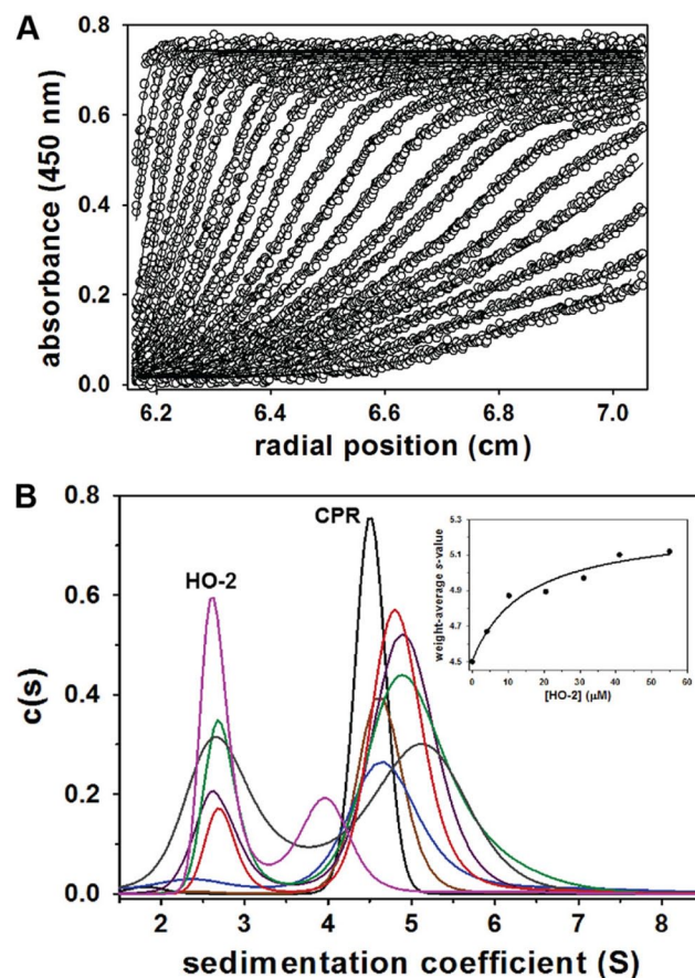
Figure 15. Sedimentation velocity analysis of HO-2 and CPR interactions. A, velocity scans selected from analysis of a 2:1 ratio of hHO-2 (41 \mu\text{M} ) to CPR (20.5 \mu\text{M} ). Shown are the absorbance data (open circles) fitted (solid lines) to the continuous c(s) distribution model. B, sedimentation coefficient distributions of CPR (20.5 \mu\text{M} ) alone (black trace) and in the presence of 4.1 \mu\text{M} (brown trace), 10.25 \mu\text{M} (blue trace), 20.5 \mu\text{M} (red trace), 30.75 \mu\text{M} (purple trace), 41 \mu\text{M} (green trace), and 55 \mu\text{M} HO-2 (gray trace). hHO-2 alone (41 \mu\text{M} ) is shown in magenta. The inset shows the weight-average s value plotted versus HO-2 concentration. The data were fit to a single-site binding isotherm to yield a K_d value of 15.1 \pm 6.5 \mu\text{M} .
