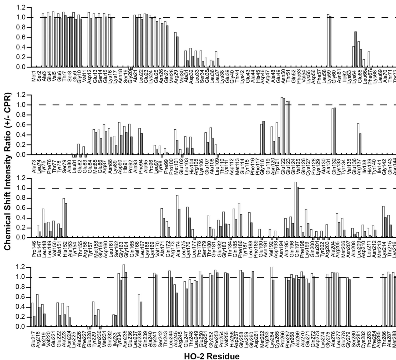
Figure 6. Effect of CPR on perdeuterated hHO-2 chemical shift intensities. Histogram bars represent the ratio of peak height in the absence or presence of CPR (+CPR/−CPR). Ratios with 75 and 150 \mu M CPR are shown (white and gray, respectively). A ratio of 1 (dotted line) indicates no change for that residue. Negative bars represent cross-peaks that are broadened beyond detection with the addition of CPR. Bars that are absent represent residues that are unassigned in the spectrum.
