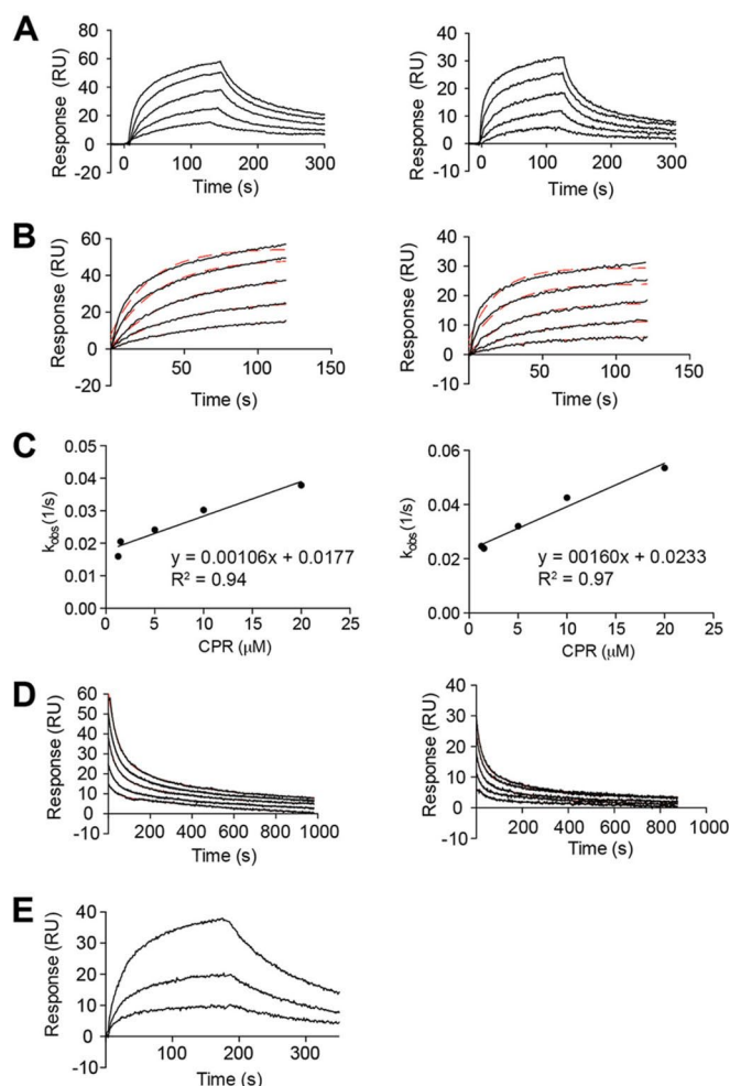
Figure 14. SPR analysis of CPR binding HO-1 (left panels) and HO-2 (right panels). A, various concentrations of CPR (1.25, 2.5, 5.0, 10.0, and 20.0 \mu\text{M} ) were injected against immobilized HO-1 or HO-2. B, single exponential fits for the association phase of CPR binding HO-1 or HO-2 are shown in red. C, single exponential fits were used to determine k_{\text{obs}} for the association phase of CPR binding HO-1 or HO-2. k_{\text{on}} and k_{\text{off}} values are derived from the linear regression of k_{\text{obs}} ( k_{\text{on}} = slope; k_{\text{off}} = y intercept). D, bi-exponential fits for the dissociation phase of CPR binding HO-1 or HO-2 are shown in red. E, various concentrations of heme (0.125, 0.25, and 0.5 \mu\text{M} ) were injected against immobilized CPR. Data are representative of three independent experiments.
