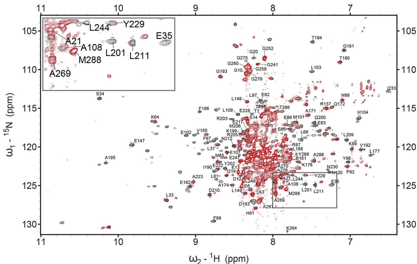
Figure 2. NMR analysis of CPR binding hHO-2. ^1\text{H} - ^{15}\text{N} TROSY spectra of 150 \mu\text{m} perdeuterated ^{15}\text{N} -hHO-2 collected in the absence (black) or presence (red) of equimolar CPR.
