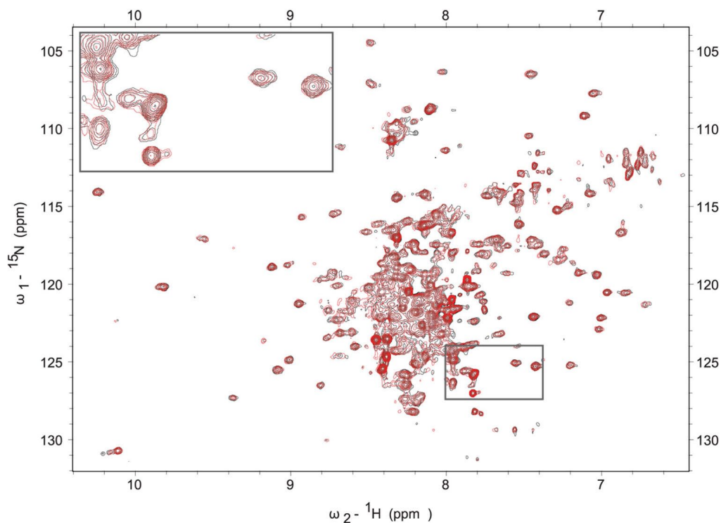
Figure 17. NMR analysis of BVR binding HO-2. ^1\text{H} - ^{15}\text{N} TROSY spectra of 150 \mu\text{m} non-perdeuterated ^{15}\text{N} -hHO-2 collected in the absence (black) or presence (red) of equimolar BVR.
