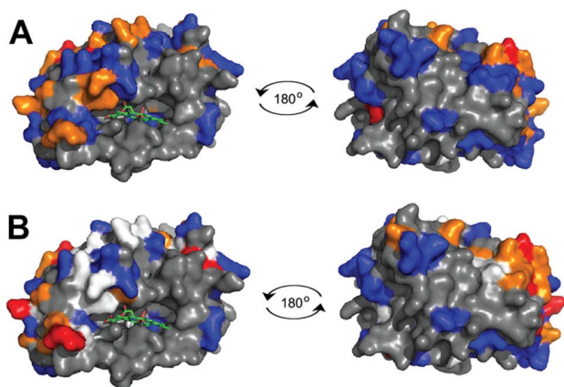
Figure 5. CPR-induced CSPs on the hHO-2 spectrum mapped onto the crystal structure. The effect of 75 or 150 \mu\text{m} CPR (A and B, respectively) on hHO-2 CSPs as determined in Figure 4 was mapped onto the crystal structure of hHO-2 (PDB 2QPP). The color of the residue reflects the degree of CSP effect by CPR. Red indicates residues with highly significant CSPs (more than two standard deviations from the mean); orange indicates residues with significant CSPs (at least one standard deviation from the mean); blue indicates residues with no significant CSP; white indicates residues that are broadened beyond detection; gray indicates residues that are unassigned.
