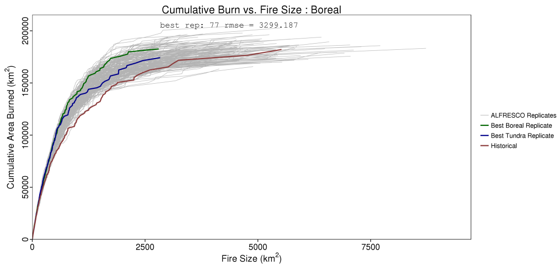
Figure 9: Cumulative area burned versus individual fire size (km 2 ) for the historical observation period 1950-2010. Red line indicates observed distribution. Green and blue lines indicate best performing simulation replicates. Gray lines indicate individual replicates (n = 200).
