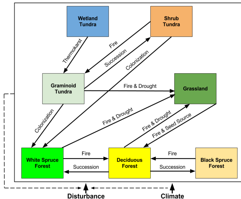
Figure 5: Conceptual diagram of the processes affecting state transitions in ALFRESCO. Arrows indicate causal relationships.
