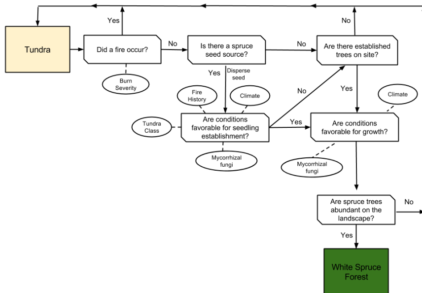
Figure 6: Conceptual diagram of the processes affecting state transitions from tundra to spruce in ALFRESCO. Arrows indicate the progression from one step in the transition process to the next step in the process.
