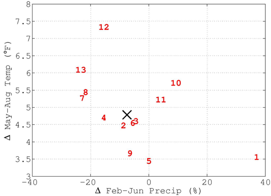
Figure 4. Distribution of model projections for mid-21 st century departures in May-August temperature and February-June precipitation from historical normals for 13 GCMs (red numbers) and the multi-model ensemble mean (black 'X').
