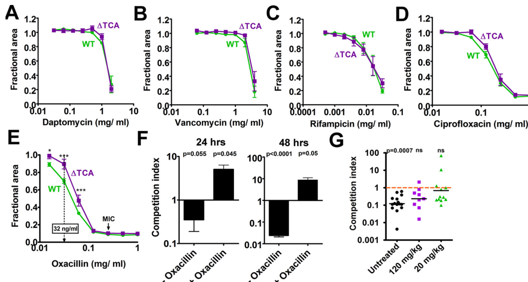
FIG 1 TCA cycle activity imposes a fitness cost during antibiotic stress. The ability of strains to tolerate various concentrations of daptomycin (A), vancomycin (B), rifampin (C), ciprofloxacin (D), and oxacillin (E) was determined by monitoring growth ( OD_{600} ) according to a previously published method (10). Experiments were performed 4 times. The dotted line denotes sub-MIC concentration utilized in experiments (oxacillin, 32 ng/ml). (F) Competitive fitness of the WT relative to the \Delta TCA mutant was determined following coculture of equal concentrations of both strains in TSB. Competitive indices were calculated as the ratio of the \Delta TCA mutant and WT in the output normalized to the same ratio in the initial inoculum. Competitive outcomes were determined at 24 h and 48 h of growth. Horizontal lines indicate the arithmetic mean; experiments were performed three times. (G) In vivo experiments were conducted in male Sprague Dawley rats that underwent B cell ablation by two intraperitoneal cyclophosphamide injections spaced 3 days apart. Rats were infected with bacteria (both WT and \Delta TCA mutant = 10^9 CFU/ml) 24 h after the last cyclophosphamide treatment. Three and four days postinfection, rats were challenged with various doses of oxacillin, and on the fifth day they were sacrificed. Viable bacterial counts from the liver were determined by plating on TSA and TSA containing erythromycin selection. Competitive indices were calculated as the ratio of the \Delta TCA mutant and the WT in the output normalized to the same ratio in the initial inoculum. Horizontal lines indicating medians were compared to a hypothetical value of 1 (i.e., equal growth; dashed lines) to determine statistical significance. P values were determined by the Wilcoxon signed-rank test. Unless otherwise indicated, data were analyzed using the unpaired Student t test ( n \geq 3 ; *, P < 0.05 ; **, P < 0.005 ; ***, P < 0.0005 ; ns, not significant).
