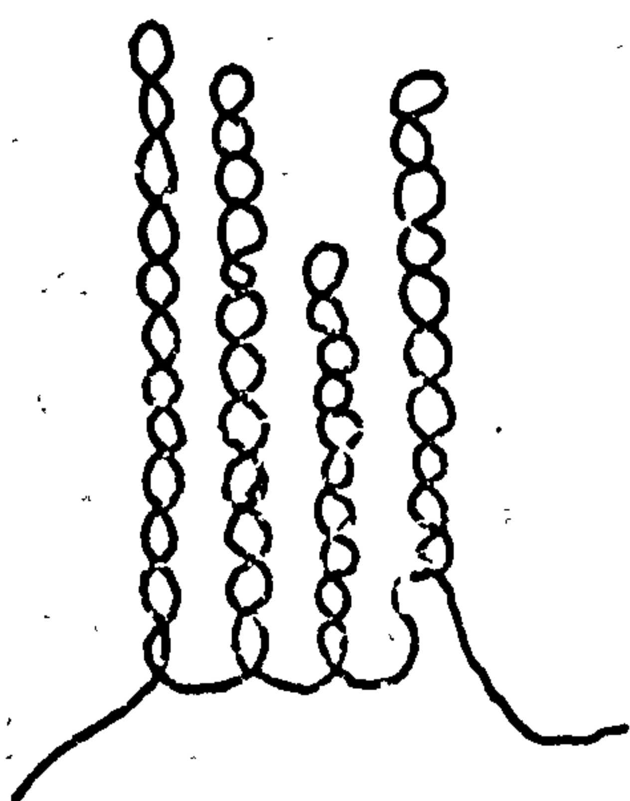
b. Antiparallel Double Helix Gel formation (taking up slack)
