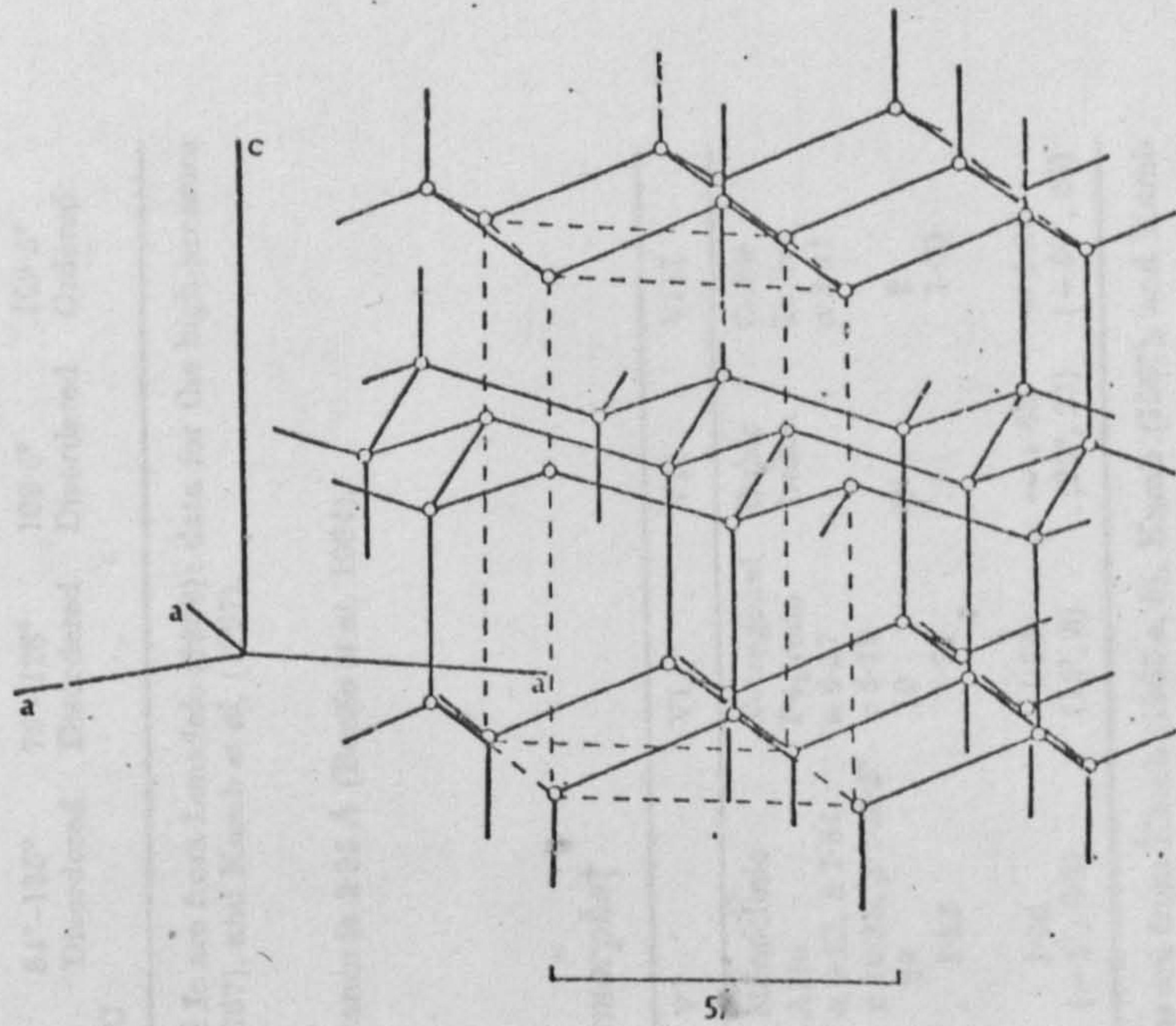
a) . The arrangement of the oxygen atoms in ice I. There are four molecules per unit cell, which is outlined in the figure by dashes. Redrawn from Owston (1958).
