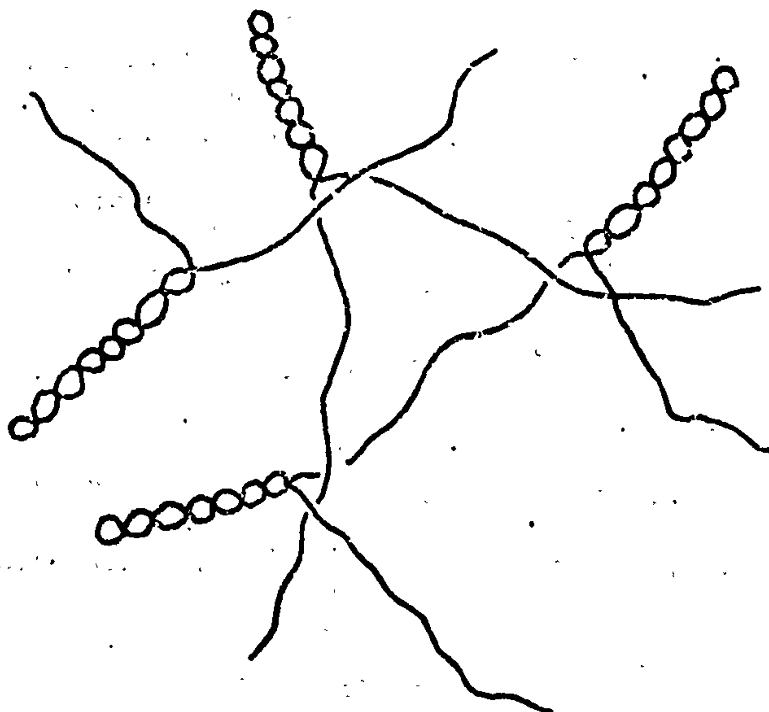
b. Antiparallel Double Helix Gel formation (taking up slack)
