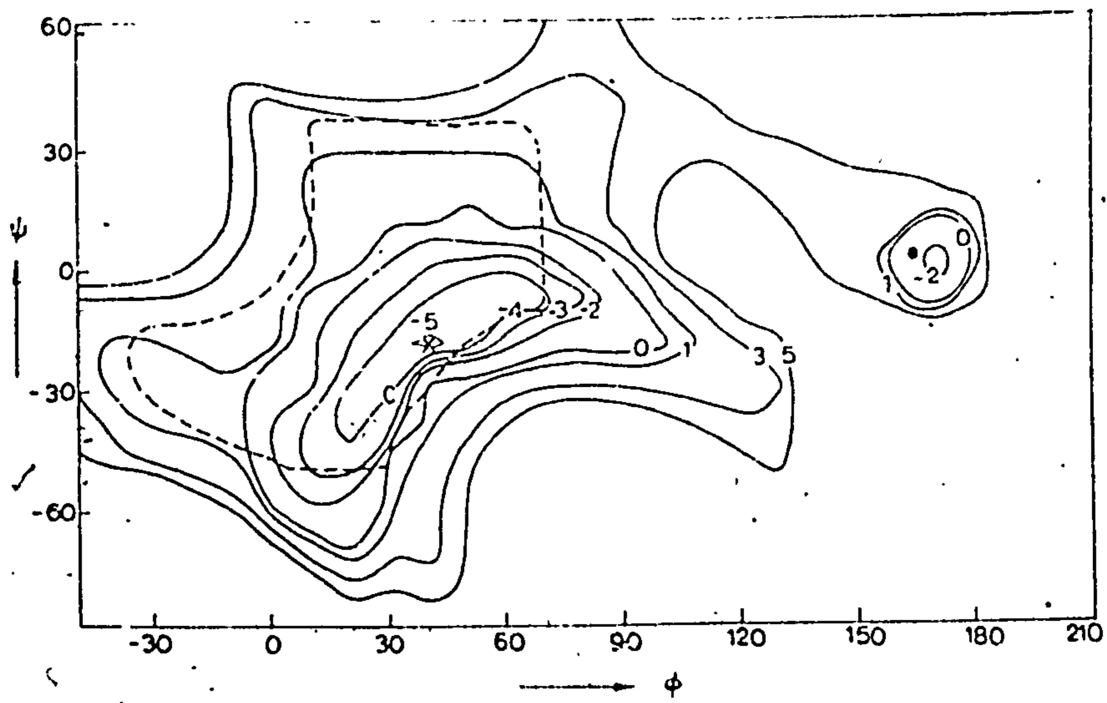
Energy contour diagram (in kcal/mole) obtained using the expression (1) for a pair of \beta -D-glucose residues joined through (1 \rightarrow 4) linkage. The steric map is indicated (- - -). \odot The position of occurrence of cellulose. \otimes Position of occurrence of minimum energy
