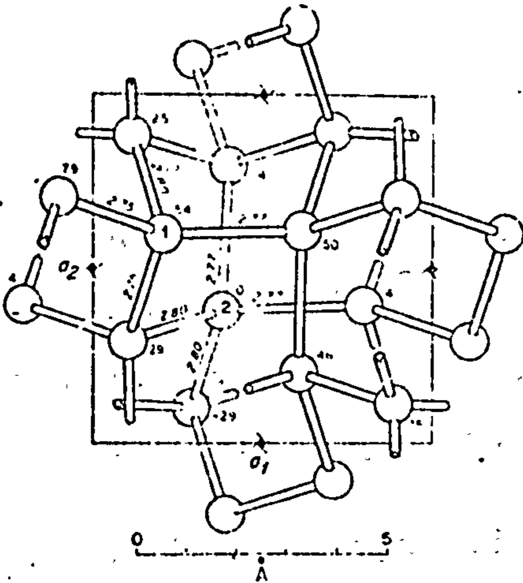
c) Ice III (along c axis)
