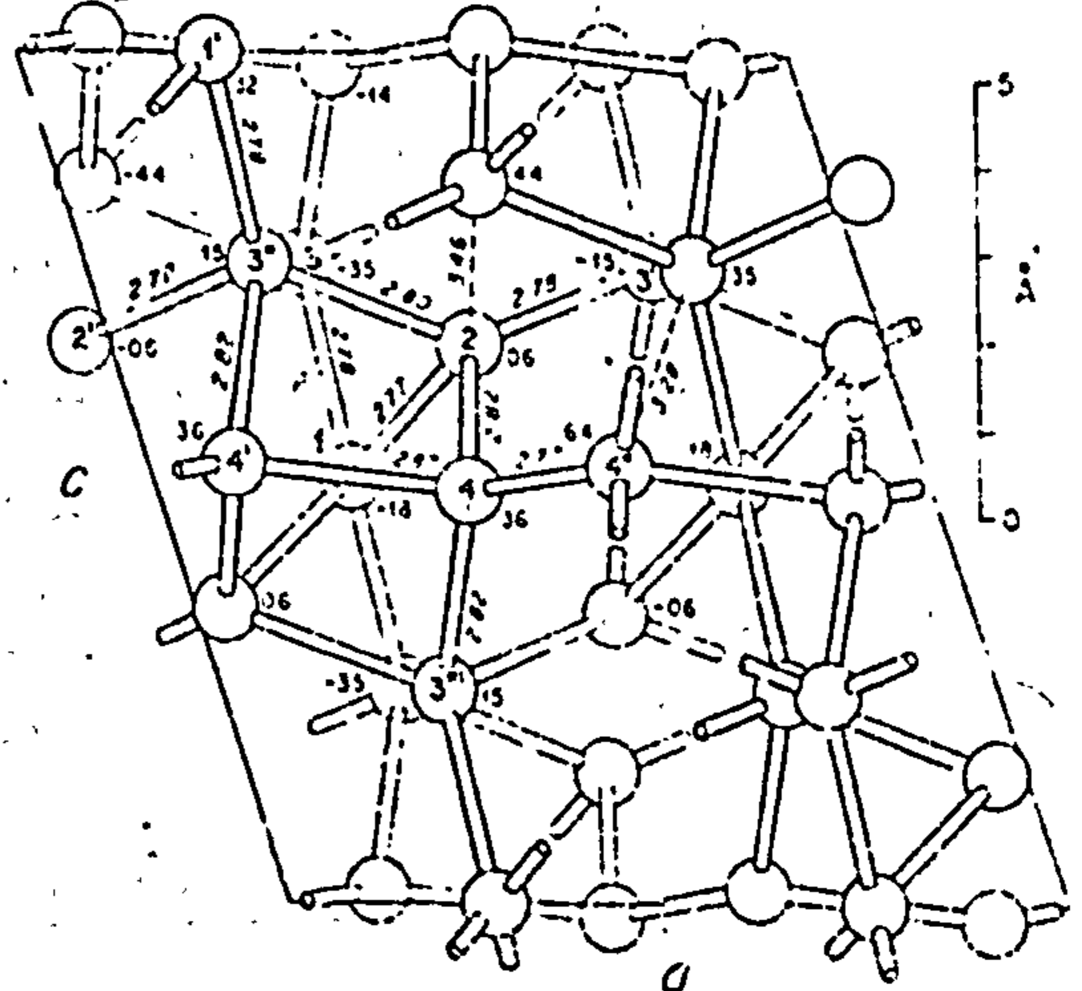
d) Ice V
