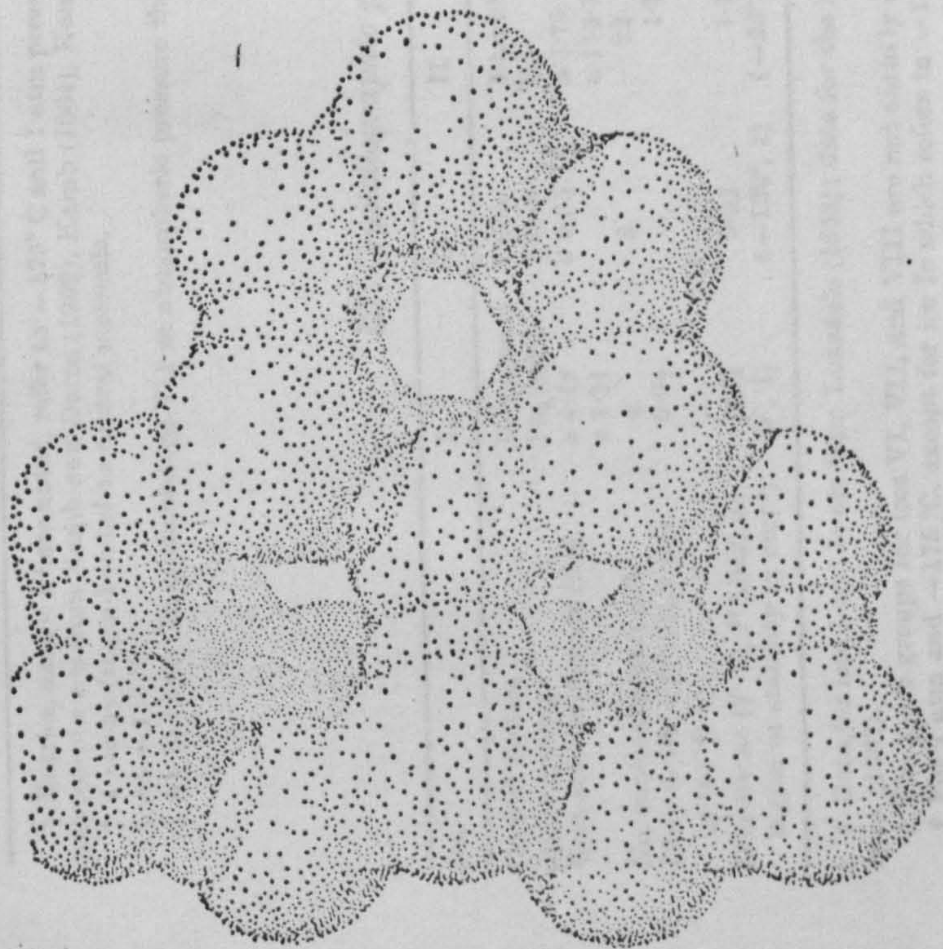
b) . A representation of an ice I crystal showing the van der Waals radii of the atoms. The view is down the c-axis, illustrating the open 'shafts'. Reproduced from Pimentel and McClellan (1960).
