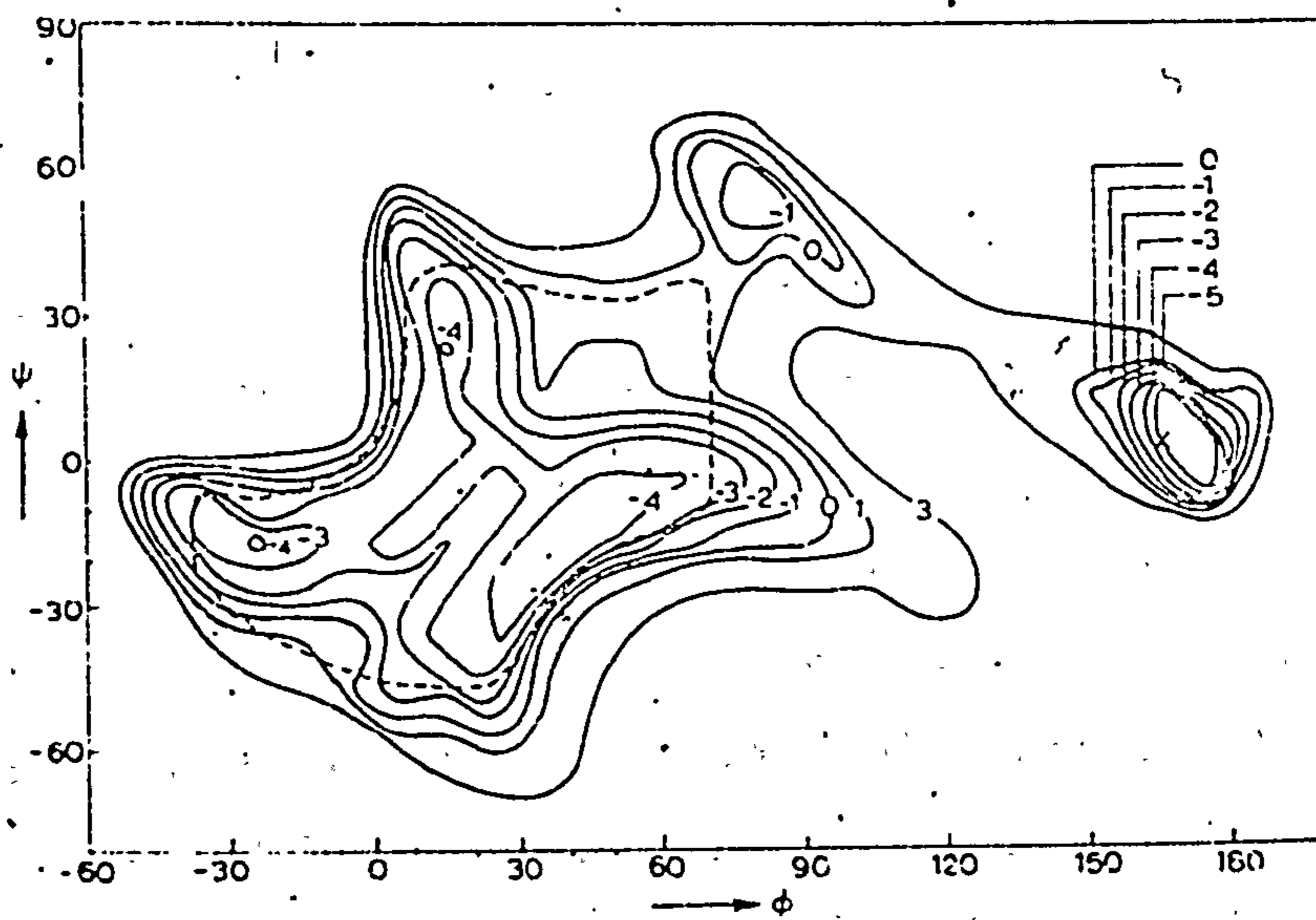
Energy contour diagram (in kcal/mole) obtained using the expression (1) for a pair of \beta -D-glucose residues joined through (1 \rightarrow 3) linkage. The steric map is indicated (- - -). \odot The position of occurrence of minimum energy.
