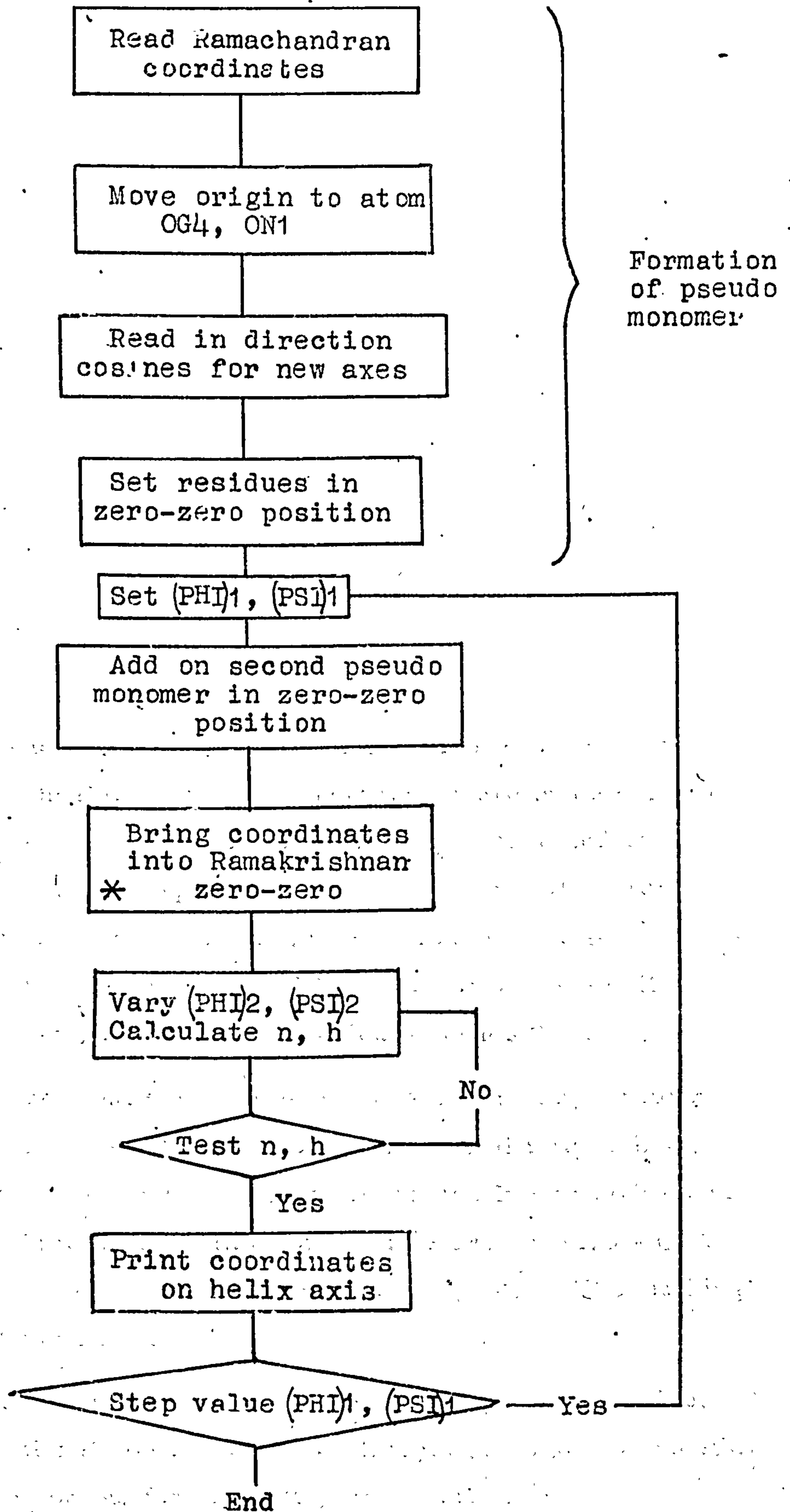
Fig. 2.14 Flow chart for computing trial conformations
