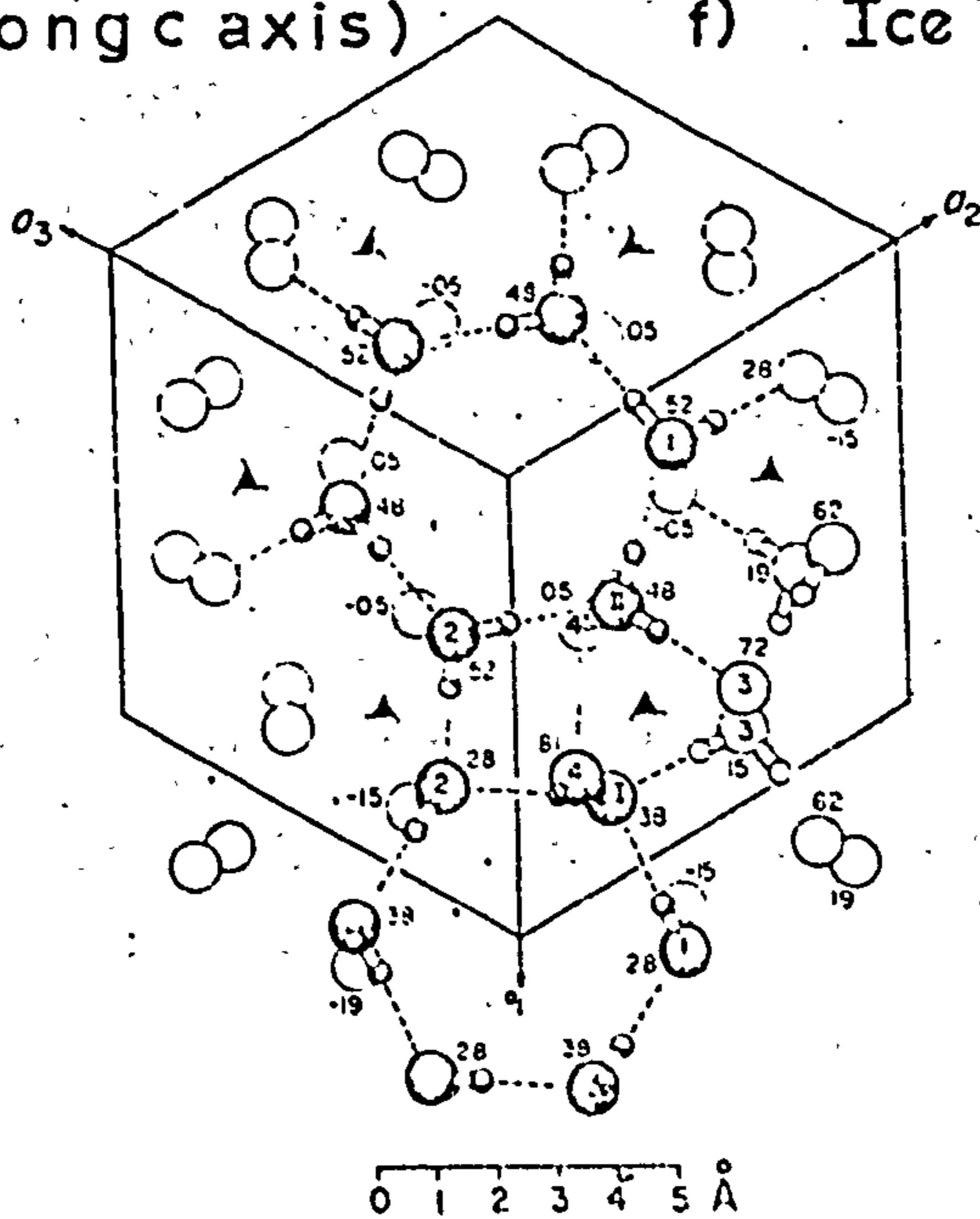
g) Ice III (along c axis)
