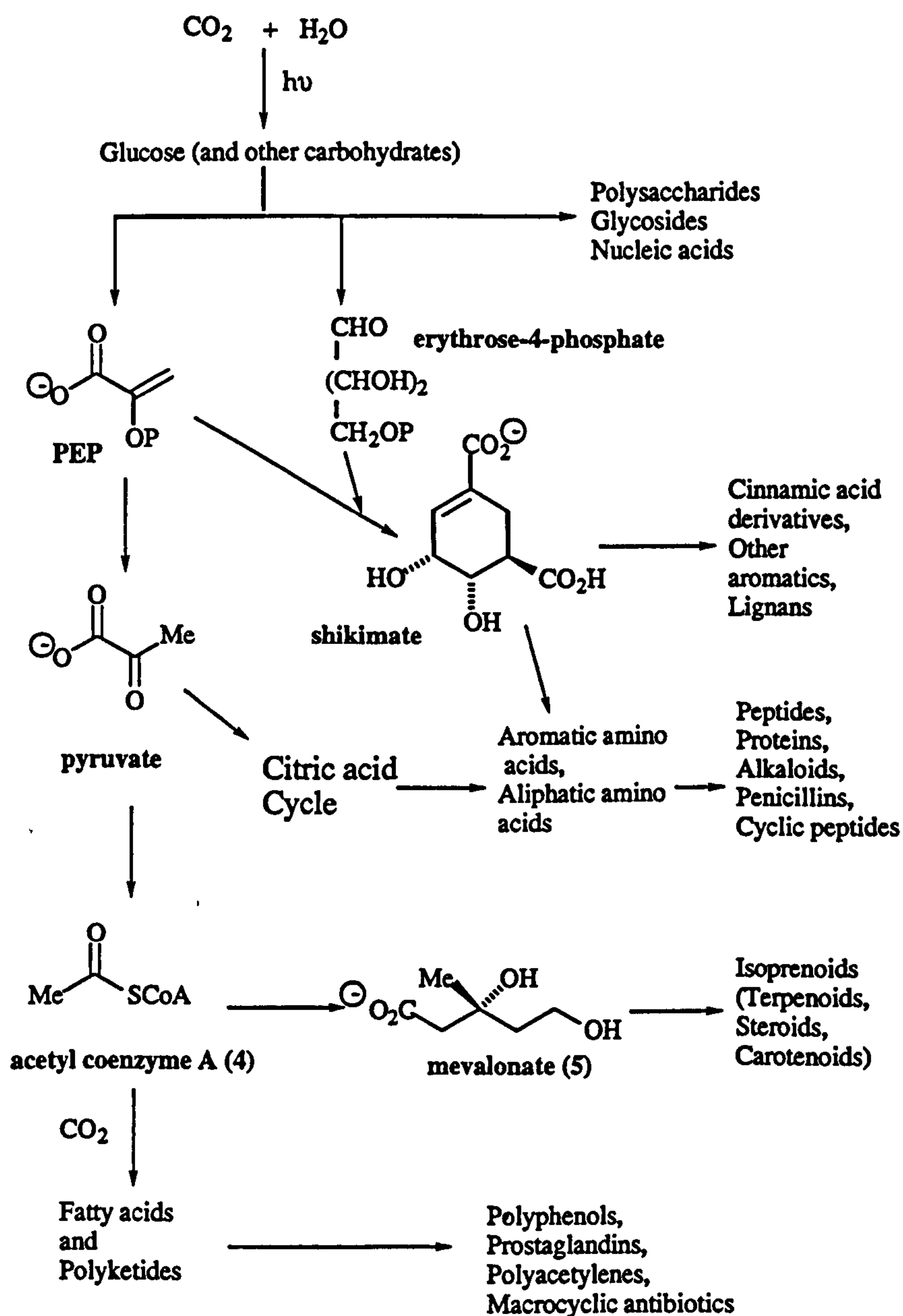
Scheme 1.1: Links between primary and secondary metabolism.
