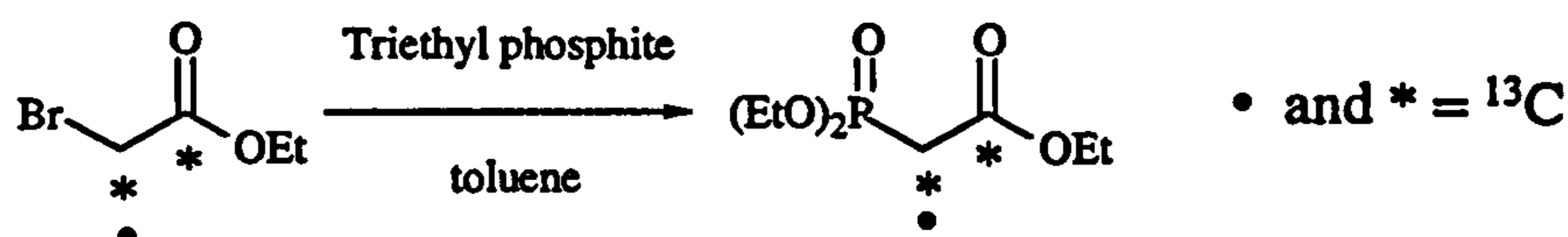
Scheme 2.38: Synthesis of ethyl phosphonoacetate, enabling incorporation of a single or double ^{13}\text{C} label.
