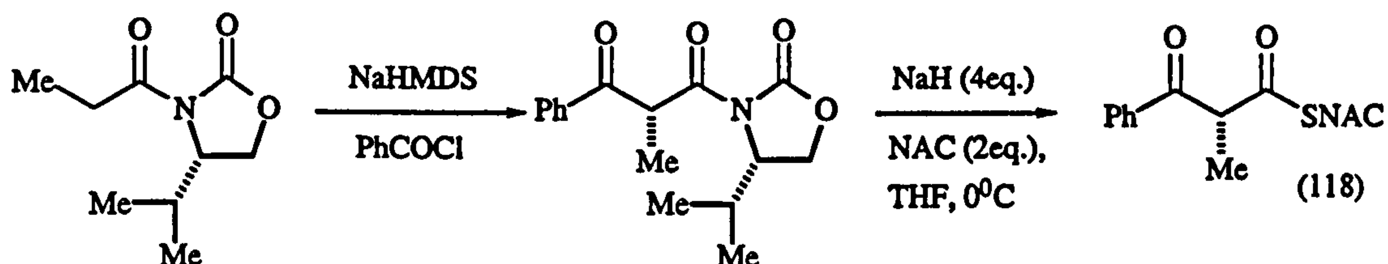
Scheme 2.15: Synthesis of the \beta -keto NAC thioester via direct displacement of the chiral auxiliary.
