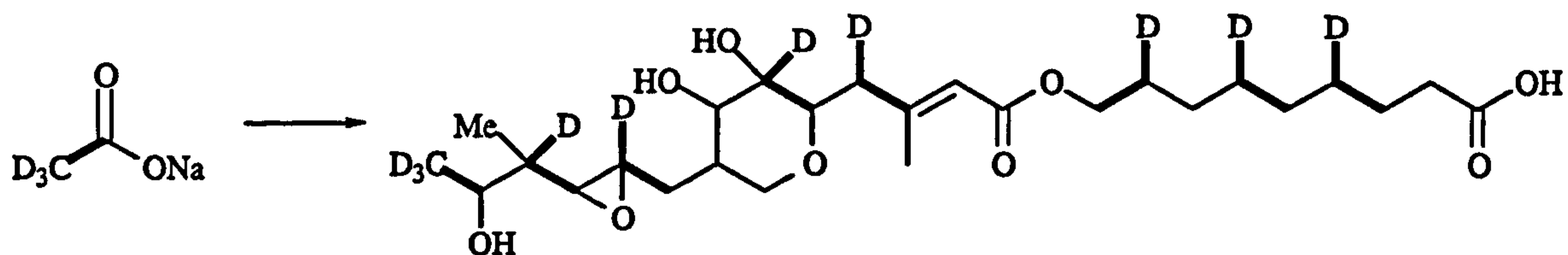
Scheme 1.23: Results of feeding [1-^{13}\text{C}, 2\text{H}_3] acetate to Pseudomonas fluorescens .
