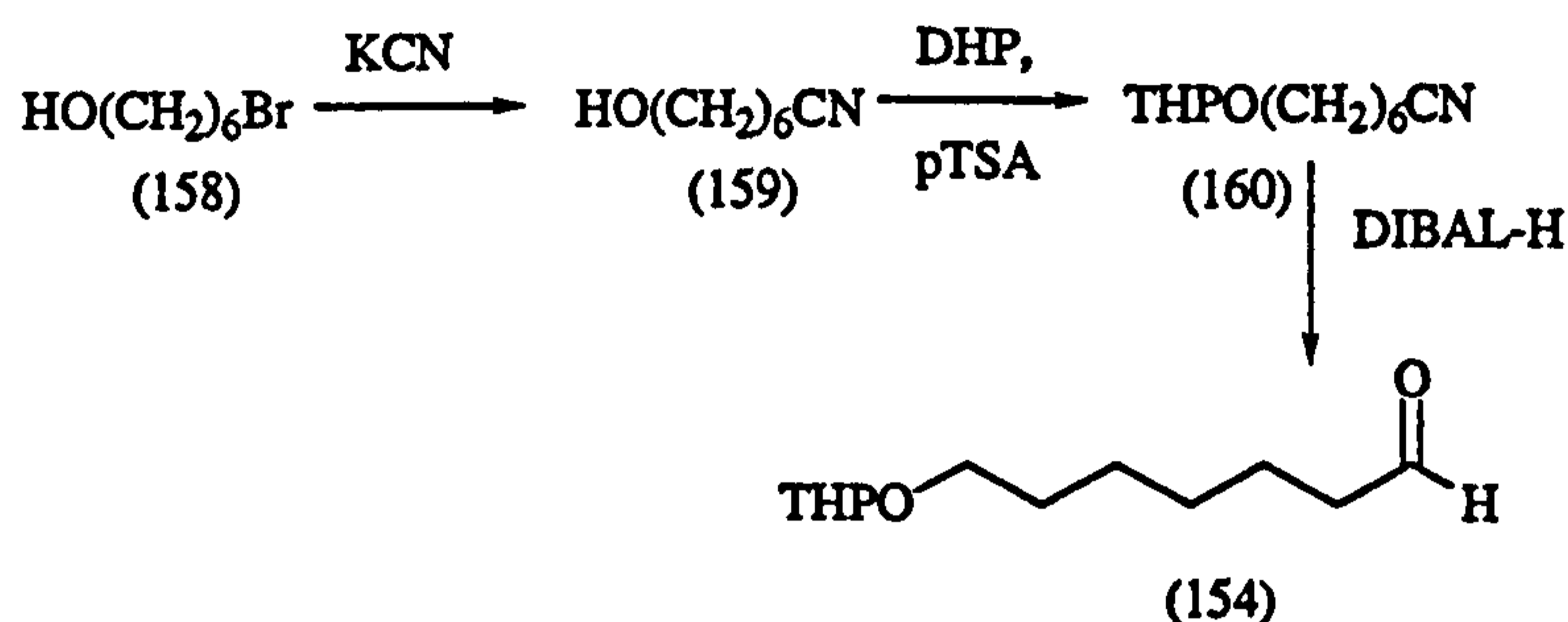
Scheme 2.36: Synthesis of 7-(1'-tetrahydropyran-2-yl)oxyheptanal, via DIBAL reduction of 7-(1'-tetrahydropyran-2-yl)oxyheptanenitrile (160).
