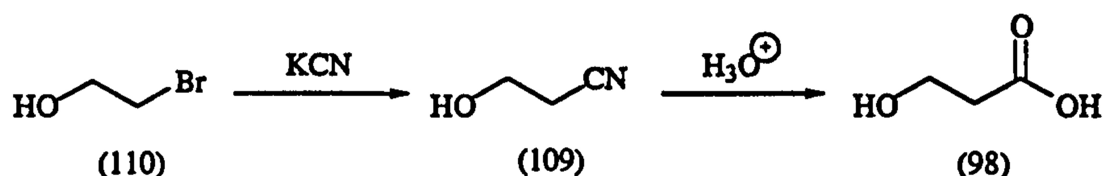
Scheme 2.9: Proposed synthesis of 3-hydroxypropionic acid (98).
