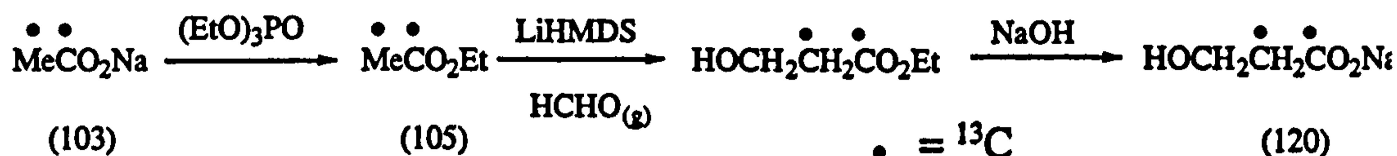
Scheme 2.16: Synthesis of sodium [1,2- 13 C 2 ]-3-hydroxypropionate
