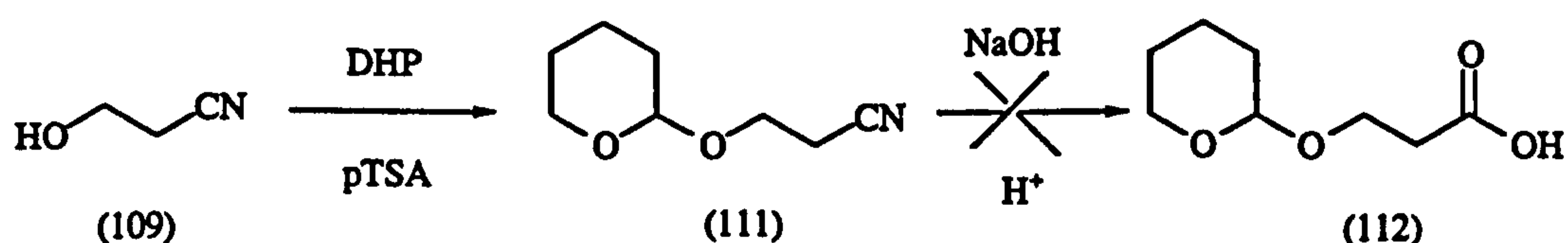
Scheme 2.10: Attempted synthesis of the THP protected 3-hydroxypropionic acid.
