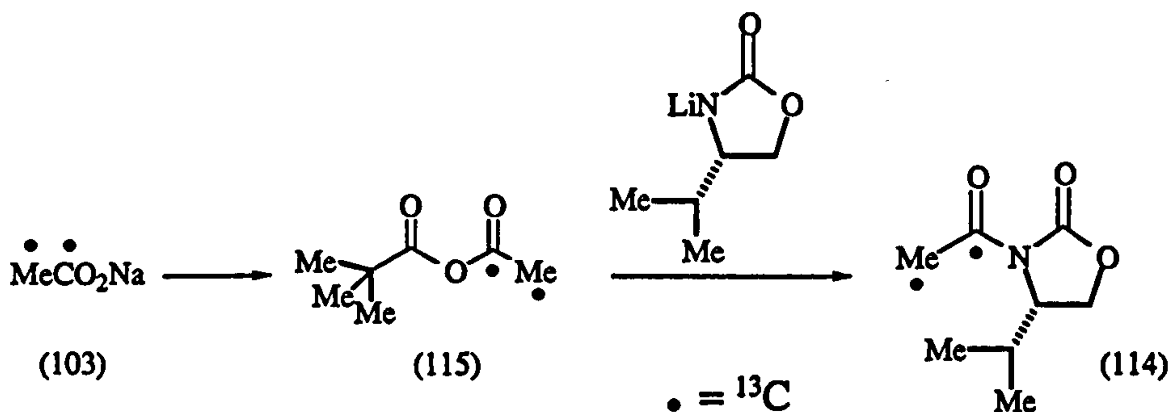
Scheme 2.13: Synthesis of (4 S )-[1,2- ^{13}\text{C}_2 ]-3-acetyl-4-(1-methylethyl)-2-oxazolidinone.
