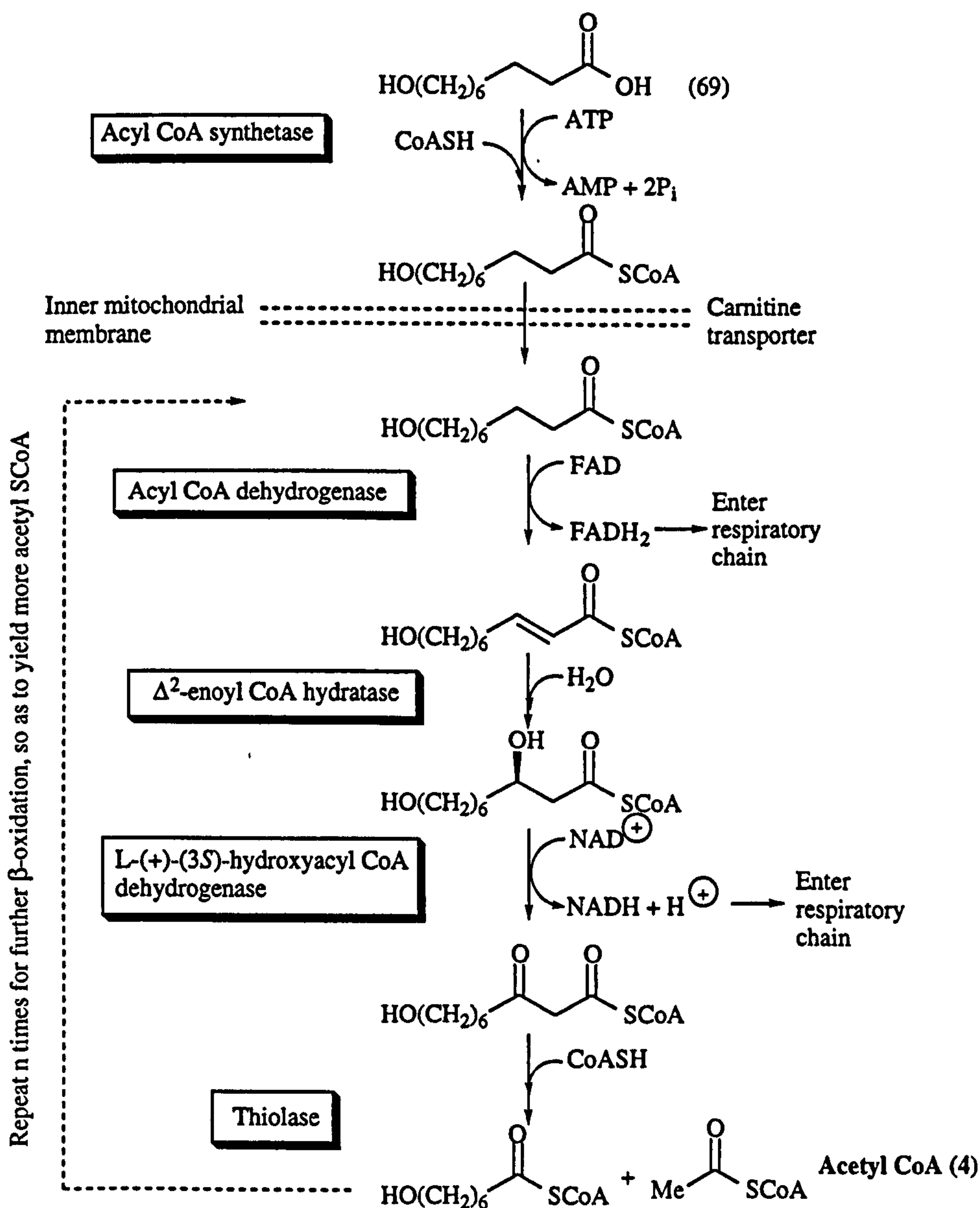
Scheme 2.23: \beta -Oxidation of 9-hydroxynonanoic acid.
