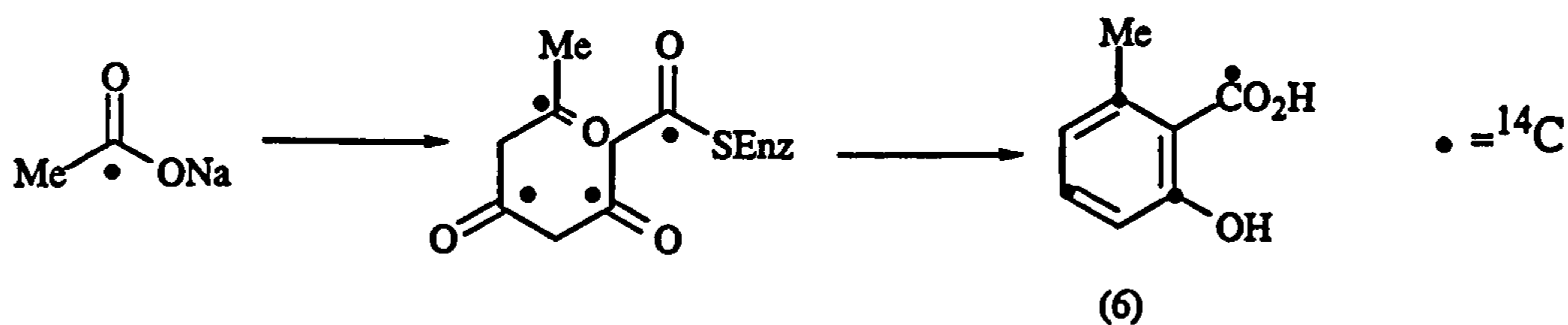
Scheme 1.4: The biosynthesis of 6-MSA.
