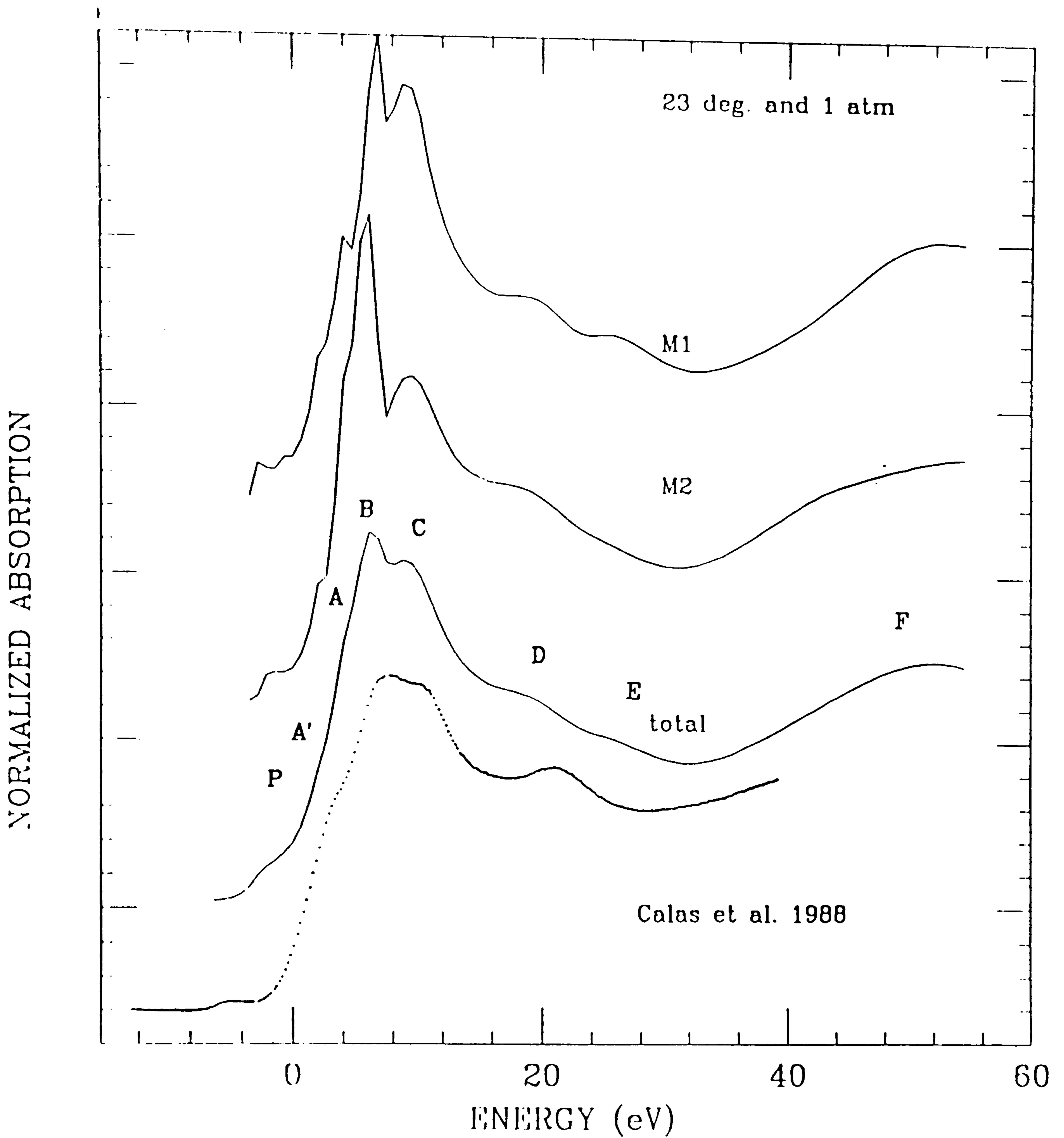
Fig. 6.2.1 Fe K-edge in Fe 2 sio 4 at ambient conditions. The top and middle curves are M1- and M2-cluster contributions with Fe in high spin final state; the third curve gives the sum of M1 and M2. The last curve is the experimental data of Calas et al. (1988)
