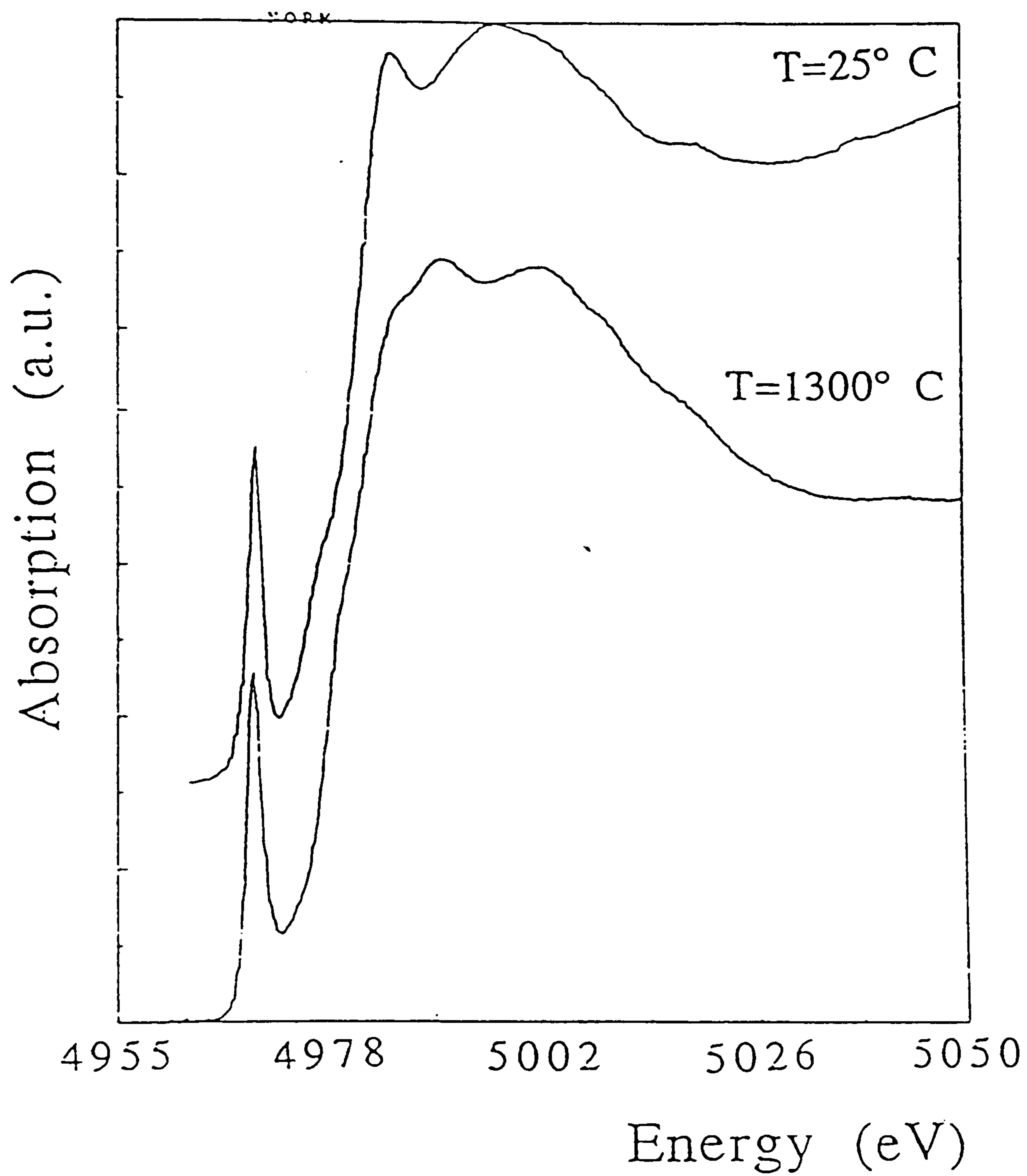
Fig. 8.1.4 XANES spectra of K_2Si_4TiO_{11} composition as quenched glass at room temperature (top) and as liquid at 1300^\circ C (bottom).
