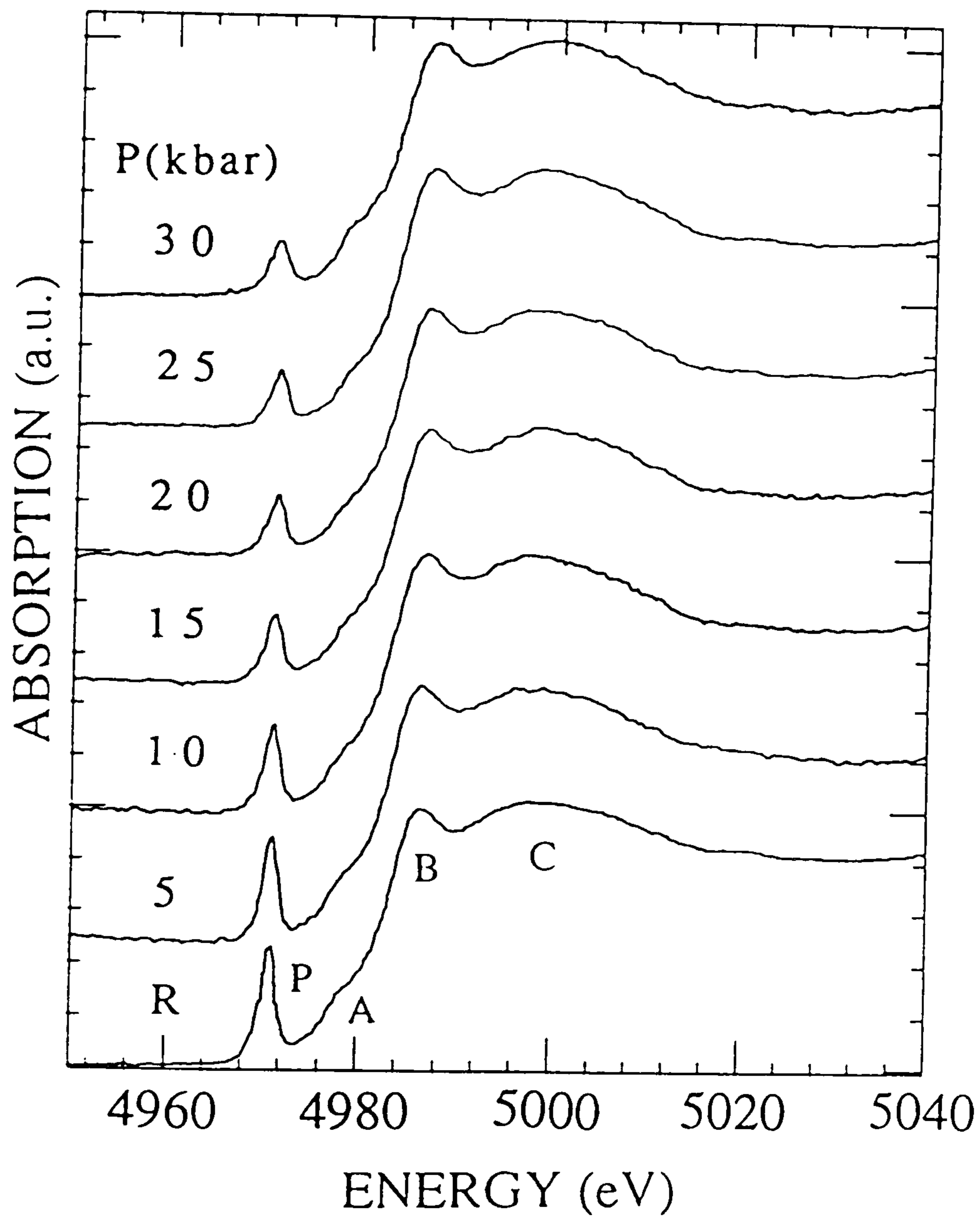
Fig. 3.3.1 Ti K-XANES spectra of K_2TiSi_4O_{11} glasses quenched from different pressures. The main resonances are shown and labelled according to the text (P pre-edge peak, A, B, C). The intensity of peak P decreases strongly with the increasing pressures, suggesting an increase of the Ti average coordination number with pressure.
