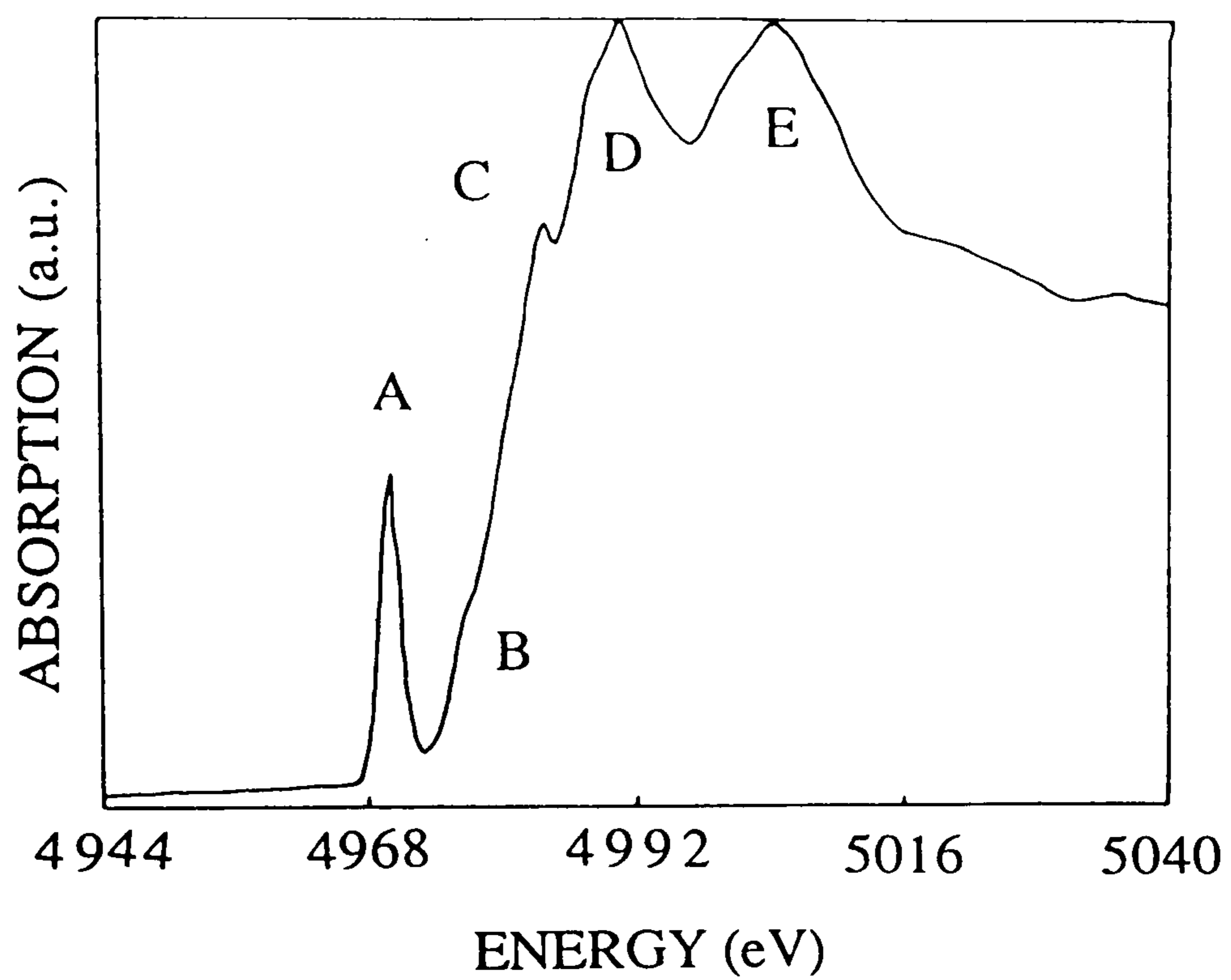
Fig. 3.1.1 XANES spectrum of Ti-richerite RI 40 TiRI 60 taken at the Ti K-edge. The spectrum is normalized at the high energy side (5027 eV). The letters correspond to different parts of the spectrum (pre-edge, edge, above-edge regions).
