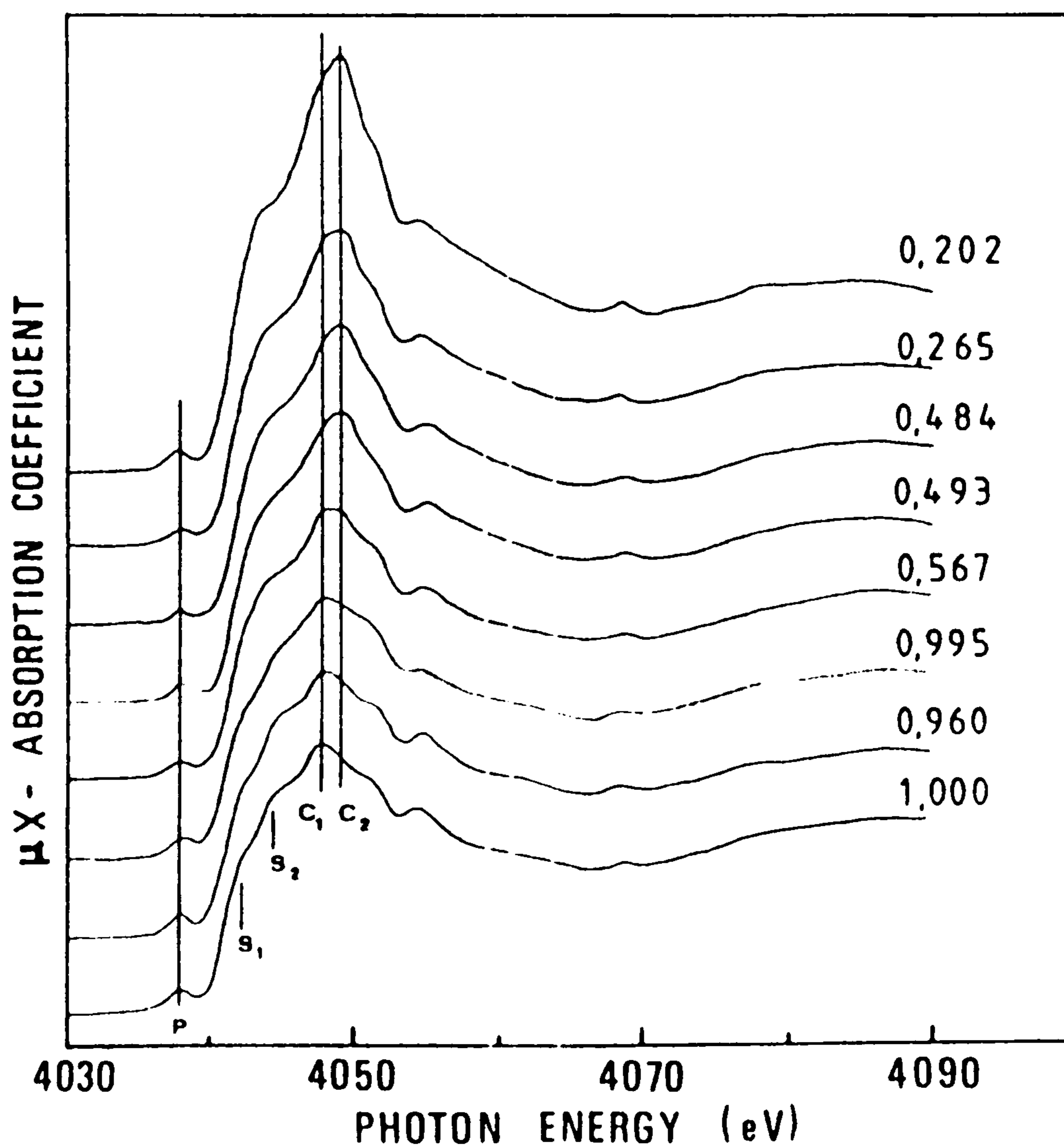
Fig. 1.2.8 XANES spectra at the Ca K-edge. Numbers next to each curve indicate the Ca content of the M2 site (Davoli & Paris, 1990).
