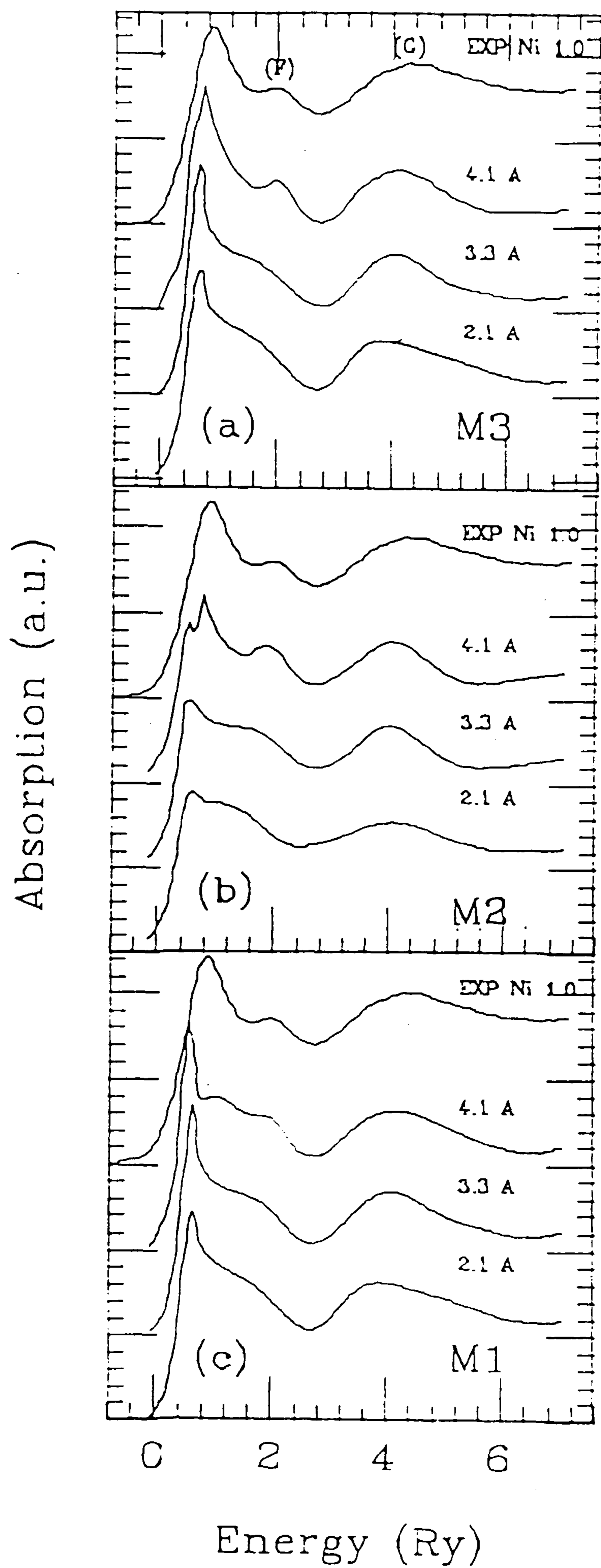
Fig. 7.1.3 Theoretical XANES spectra calculated for Ni 100 richterite, with the photoabsorber located at (a) M3, (b) M2, or (c) M1. The experimental spectrum for Ni richterite is shown at the top of each panel for comparison.
