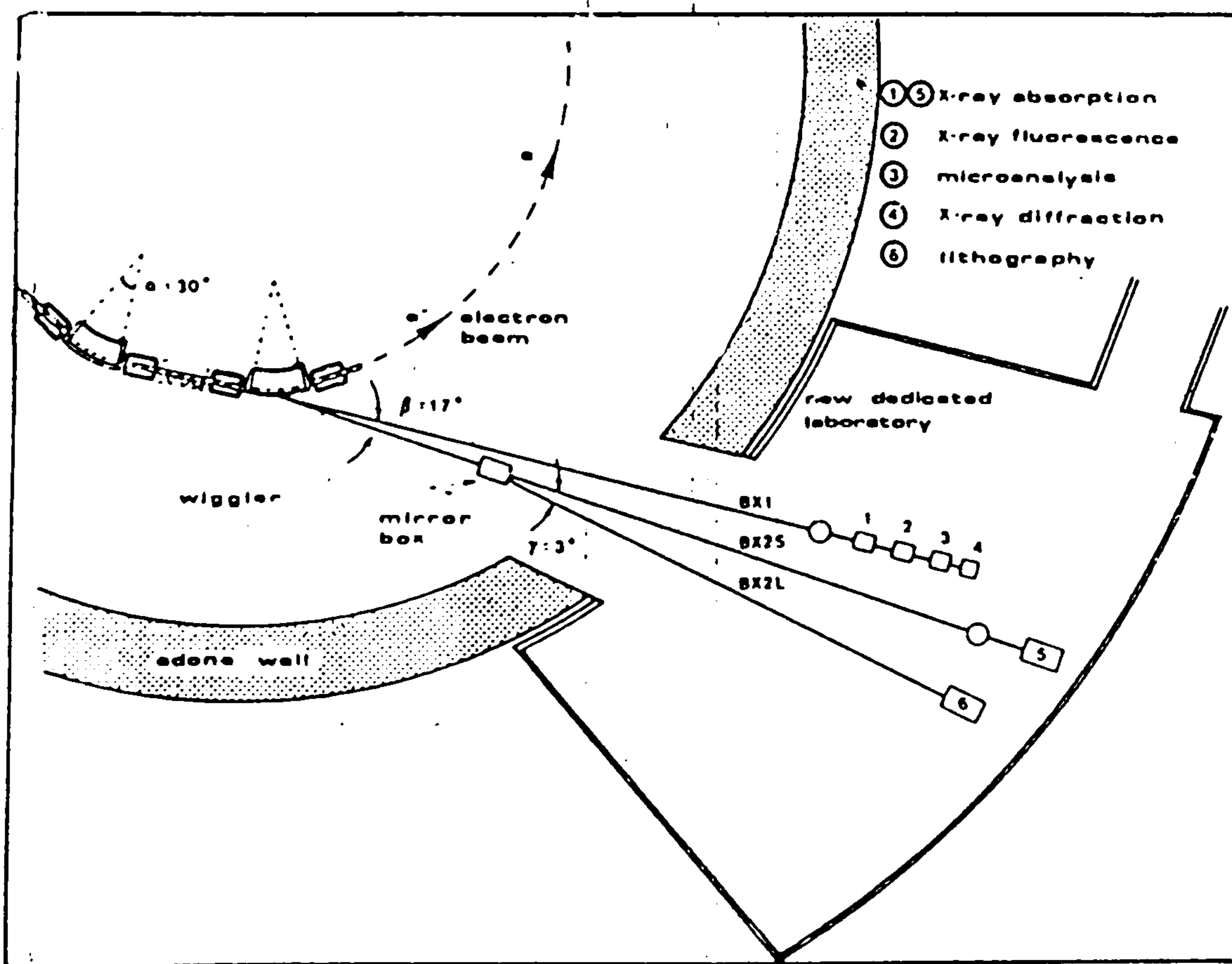
Fig. 1.1.6 Synchrotron Radiation PWA Laboratory (Frascati) using a wiggler magnet as source (Davoli et al., 1988).
