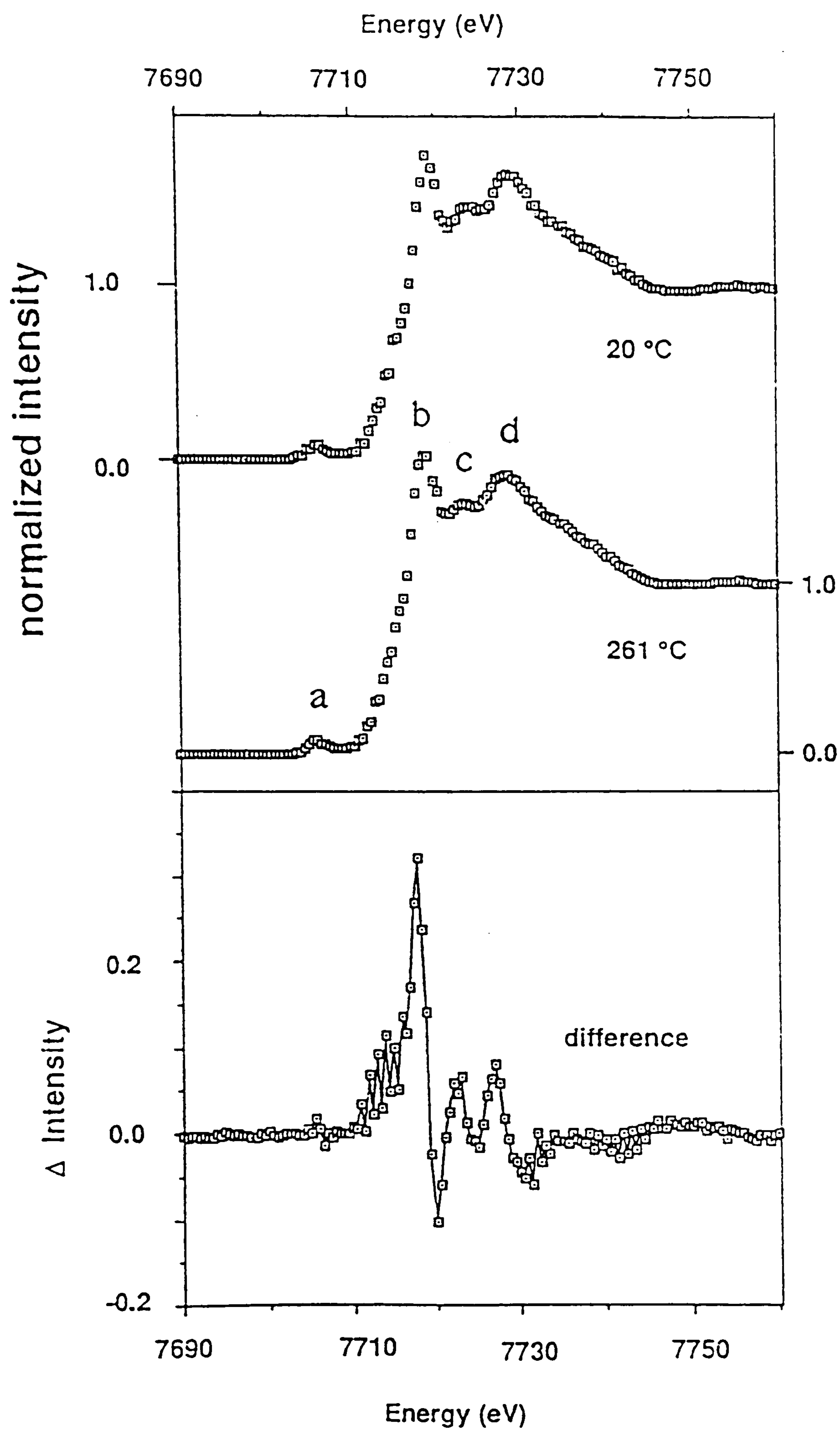
Fig. 8.1.2 Normalized Co K-edge XANES spectra of \text{Ca}_2\text{Co}[\text{Si}_2\text{O}_7] melilite taken at room temperature (top) and at 261^\circ\text{C} (middle), and their difference spectrum (bottom).
