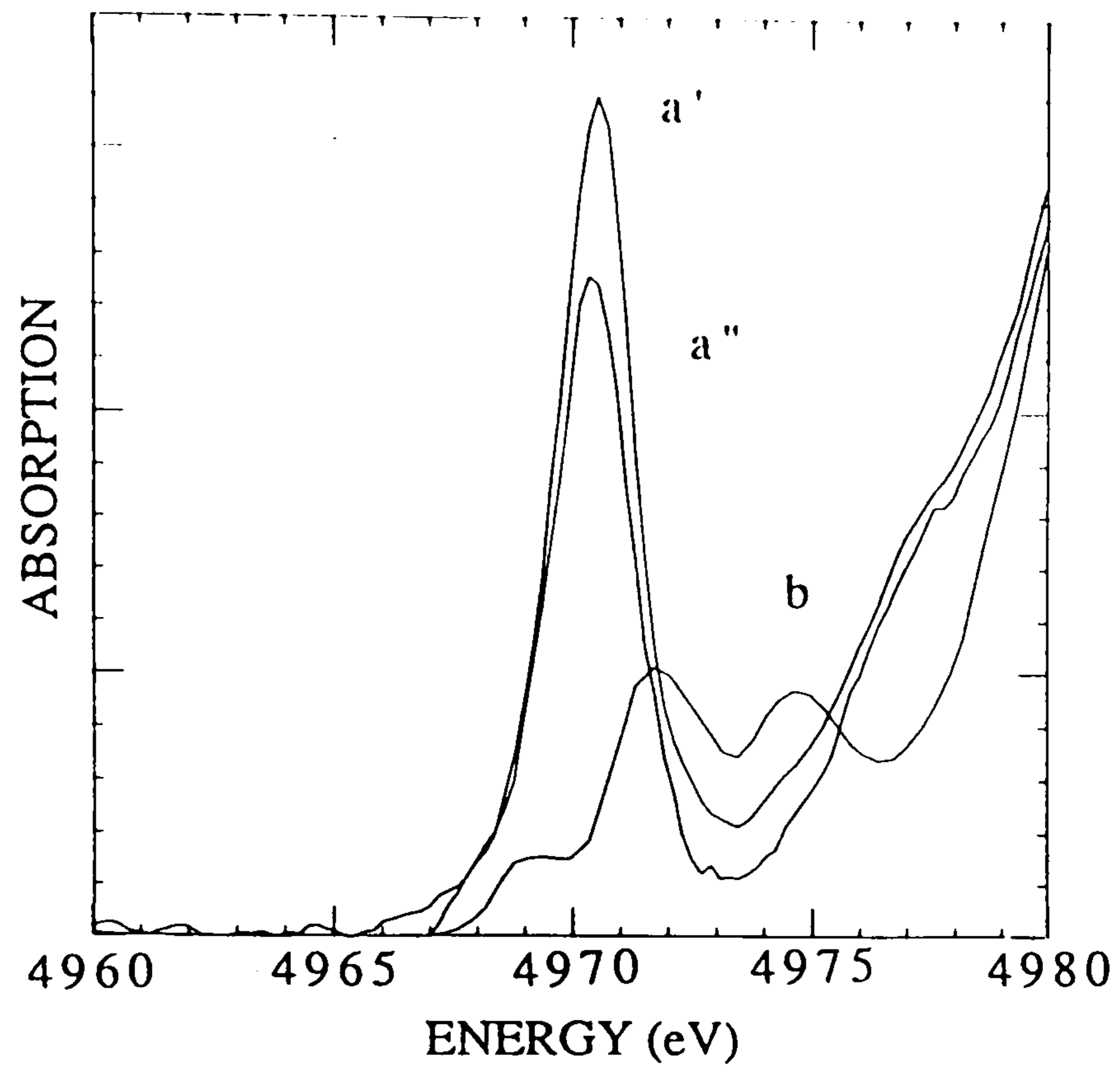
Fig. 3.1.2 The pre-edge region of single phase Ti-rich richterite \text{RI}_{80}\text{TiRI}_{20} (a'') and of nominal end-member \text{RI}_0\text{TiRI}_{100} (a') compared to that of \text{TiO}_2 (rutile) standard (b).
