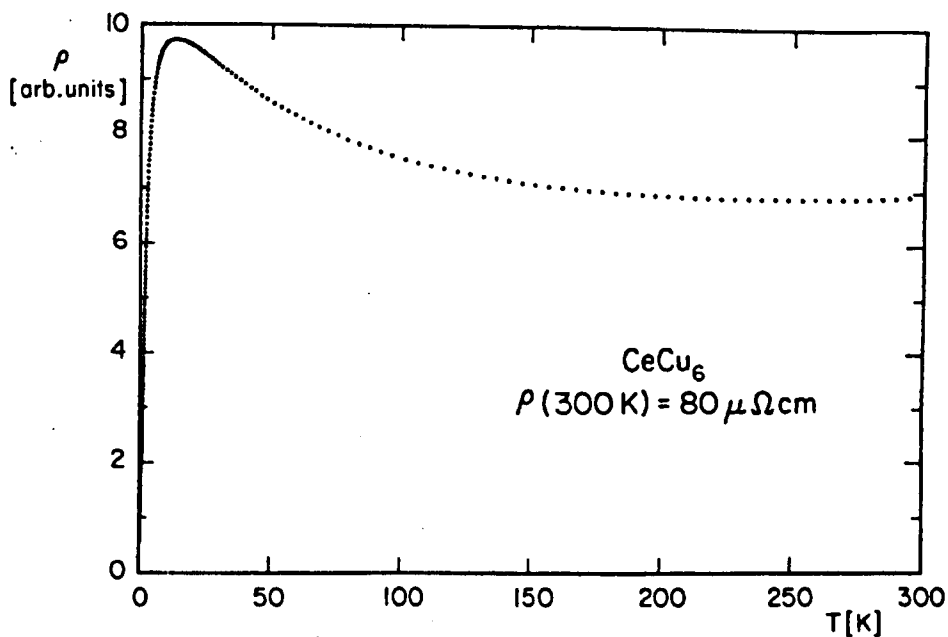
Figure 2.3: The resistivity of CeCu 6 . After Ott et al. [6].
