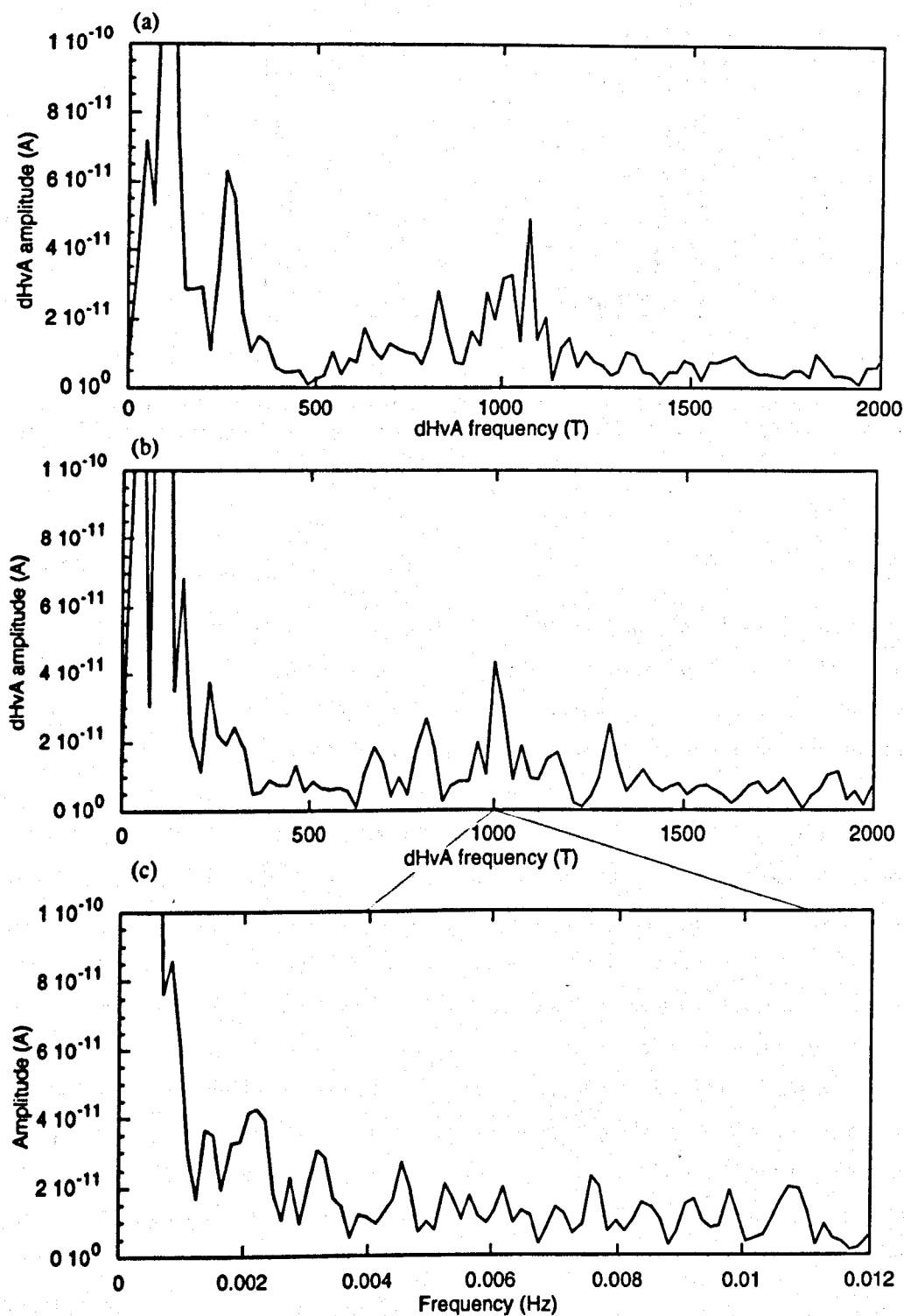
Figure 7.20: Comparison of the oscillations measured by the main field susceptometer in field sweeps between 14.5 T and 8.7 T. (a.) With the CeCu_2Si_2 crystal present. (b.) Without the CeCu_2Si_2 crystal. (c.) Without the CeCu_2Si_2 crystal, analysed with respect to time. The lines indicate the equivalent real time frequencies at either end of the field sweep.
