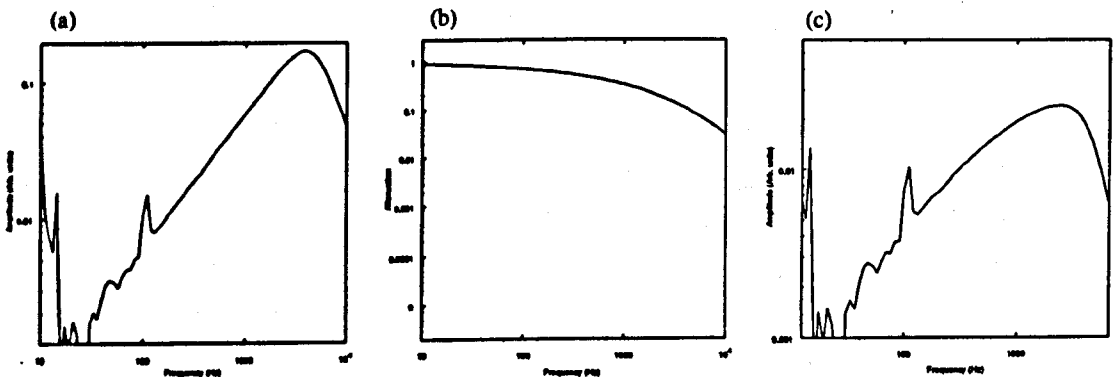
Figure 8.2: Model of the effect of screening due to the silver shield, on the frequency response of the SQUID input. (a) The frequency response measured by the electronic balancing coil. (b) The estimated attenuation due to screening by the silver shield. (c) The product of a. and b.
