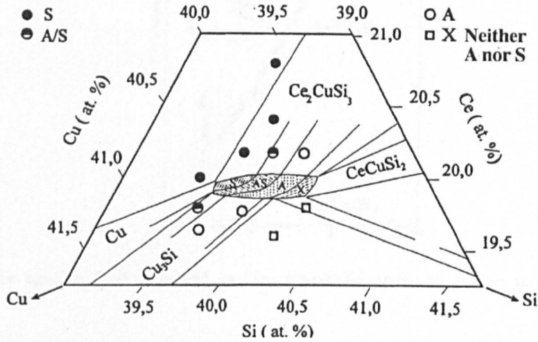
Figure 6.2: The concentration phase diagram of CeCu_2Si_2 [54]. Within a very narrow range superconducting and a separate A phase are possible as well as combinations of both or neither. The exact 1:2:2 ratio produces both phases. To achieve this it is necessary to start off with an excess of Cu.
