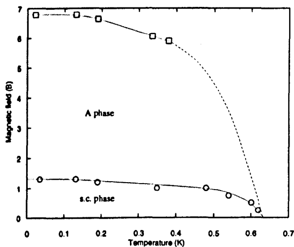
Figure 7.15: The B/T phase diagram of CeCu_2Si_2 measured using the pulsed field technique. The metamagnetic transition becomes indistinct above 400 mK so the dashed line is only drawn from analogy to experiments on other crystals measured by the Darmstadt group using magnetoresistivity.
