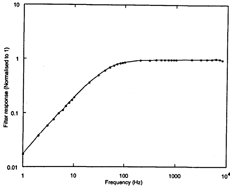
Figure 5.11: The measured input circuit filter response for a series resistor of 8 \text{ m}\Omega , employing the replica susceptometer contained within the transport Dewar probe. The 3 dB point given by R/L is 60 Hz. At higher frequencies slew rate effects are apparent.
