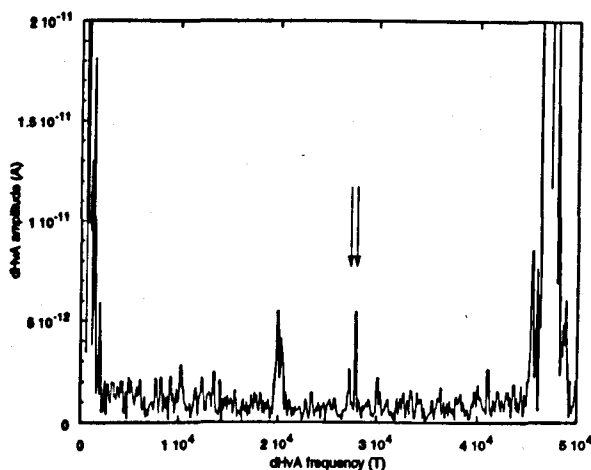
Figure 7.16: Fourier transform of a field sweep between 13 and 15 T at 2.8 mK. The oscillations that were originally attributed to CeCu_2Si_2 are at 27,250 T and 27,850 T. The oscillations at 20,000 T and 47,000 T are explicable in terms of silver.
