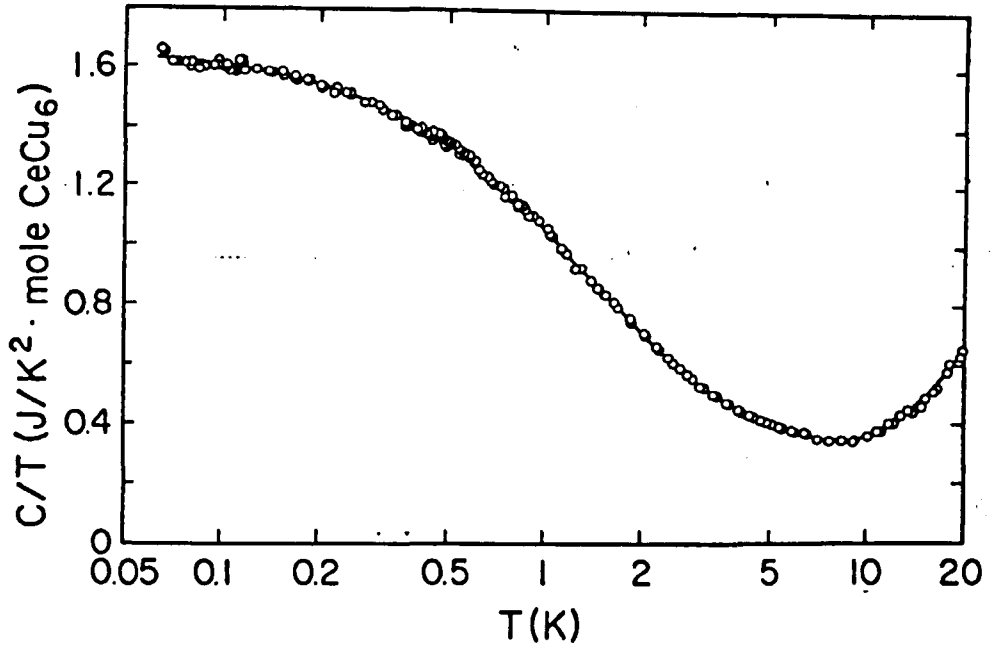
Figure 2.2: The specific heat of \text{CeCu}_6 . After Amato et al. [4].
