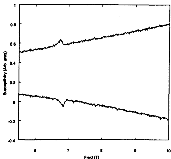
Figure 7.14: Pulsed field experiment with the sweep rate 0.693 T/min, a SQUID gain of 500 and a low pass filter of 1 Hz. The two traces correspond to an up sweep (below) and a down sweep (above). The metamagnetic transition is clearly visible.
