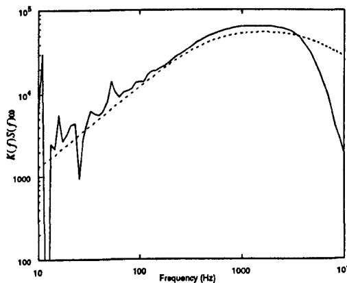
Figure 5.16: The value of K(f)S(f)\omega (for the main susceptometer), based on the first principles calculation (dashed line) and based on the measurement of the superconducting transition in CeCu_2Si_2 (solid line).
