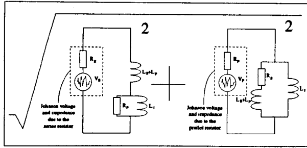
Figure 5.21: A model of the Johnson noise due to two resistors as an incoherent sum of the currents.
