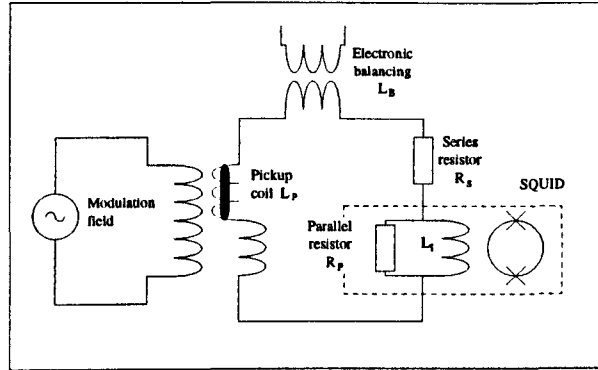
Figure 5.15: A SQUID input circuit possessing both series and parallel resistors.
