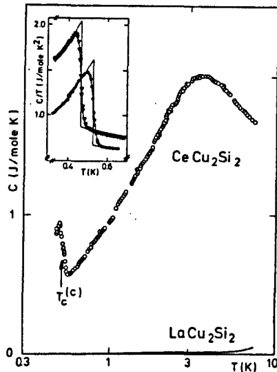
Figure 6.4: The specific heat observed at the superconducting transition in CeCu_2Si_2 . From Steglich [55].
