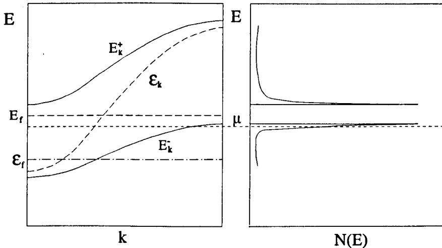
Figure 3.4: Sketch showing the renormalised band structure and density of states for a heavy fermion compound, employing the mean field solution of the periodic Anderson model. Without interactions, one has a broad conduction band \epsilon_k and an f-level at \epsilon_f . Interactions produce a quasiparticle band near E_f and hybridisation produces the two bands E_k^+ and E_k^- .
