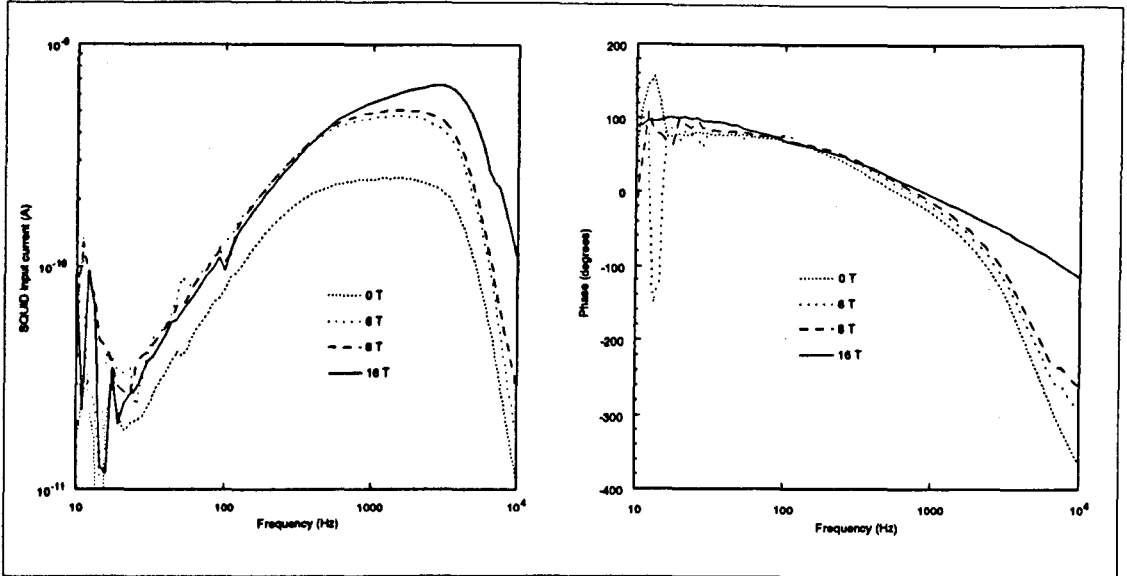
Figure 7.9: The frequency dependence of the amplitude and phase of the out of balance signal from a nominally balanced pickup coil with the CeCu_2Si_2 sample in it. The field applied was 4 \times 10^{-8} T_{RMS} . The form is not as one would expect considering a simple L-R circuit. Also note the effect of the superconducting crystal at 0T. Both these features are discussed in chapter 8.
