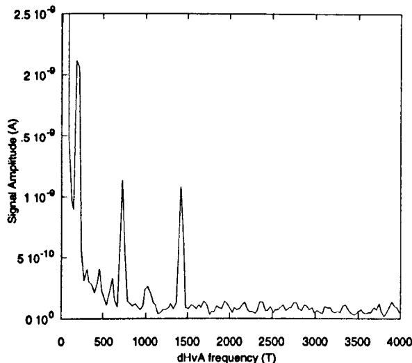
Figure 7.5: The dHvA oscillations observed in the secondary susceptometer that were initially ascribed to CeCu_2Si_2 . The field range was 6.2-7.8 T and the temperature is chosen to be 487 mK, to maximise the 1440 T peak.
