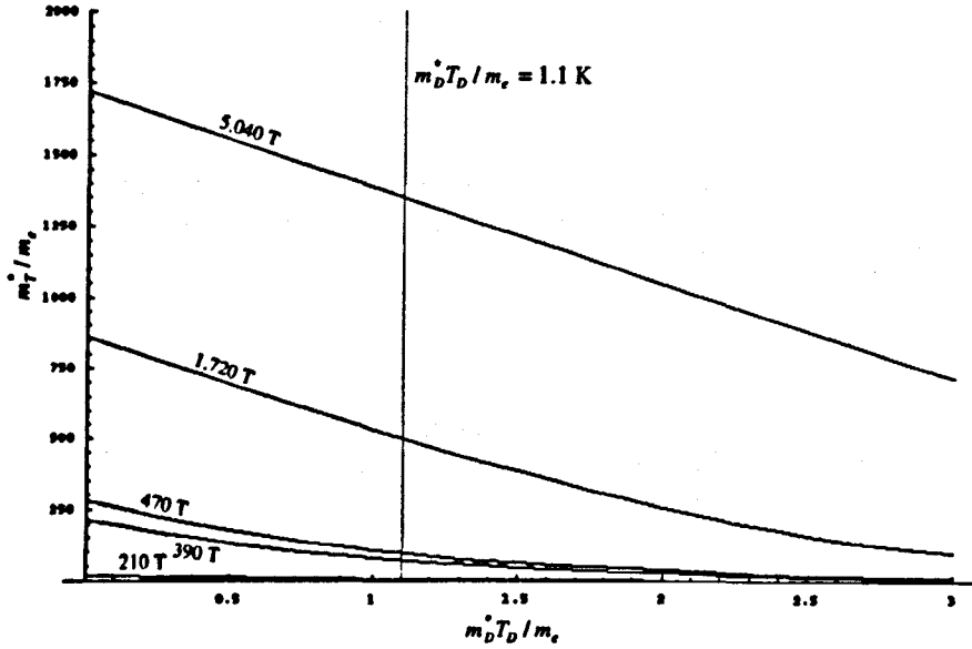
Figure 8.13: Attainable m_T^*/m_e for a given m_D^* T_D / m_e , using the calculated frequencies and curvature factors of Harima and Yanase [65].
