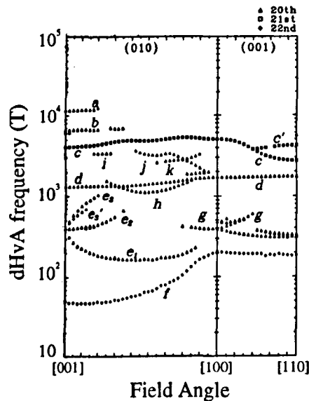
Figure 6.8: The dHvA spectra predicted for CeCu_2Si_2 by Harima and Yanase [65].
