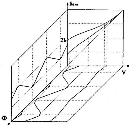
Figure A.3: Plot displaying the behaviour of a d.c. SQUID when biased by a current. The periodic nature of the critical current manifests itself in the V/I curve so a finite current across the ring produces a flux dependent voltage. The voltage swing is a maximum when the SQUID is biased just above its (integer \Phi_0 ) critical current.
