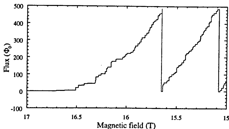
Figure 5.23: The SQUID output during a field sweep from 17 to 15 T. The small steps are unlockings and the large jumps are resets. The gain was set to \times 1 . Typical unlocking sizes are 2-10 \Phi_0 . Note the hysteretic, calm half tesla before unlockings occur.
