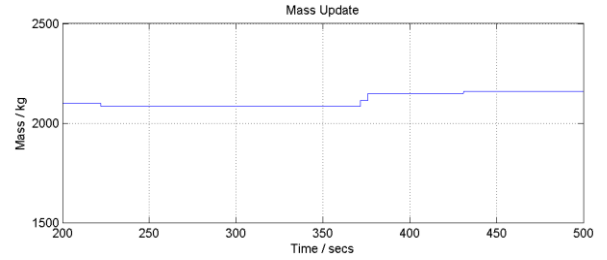
Figure 9. A section of mass estimate from the parameter-convergence method, illustrating the discrete nature of the mass output
