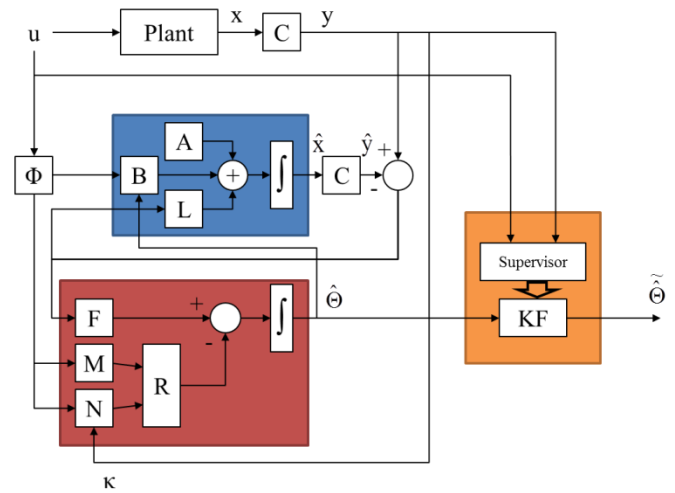
Figure 3. Diagram showing the estimator system structure with the observer and regressor components, the supervisor and output filtering and their dependencies on the real plant inputs and outputs
