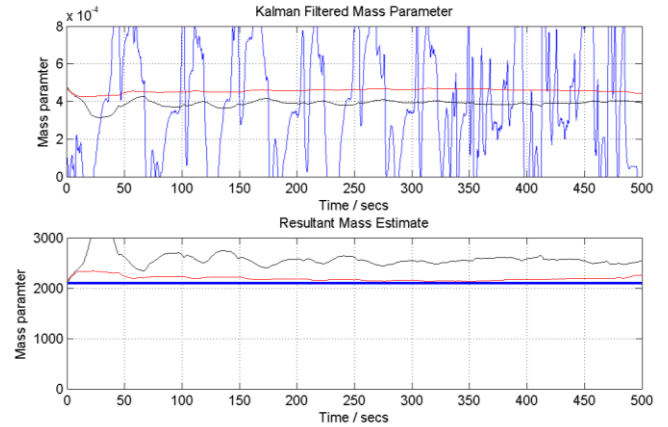
Figure 10. Results of applying Kalman Filtering (black) and supervised Kalman Filtering (red) to the output of the mass estimation process. The unsupervised Kalman filter suffers some colouration from the zero-crossings caused in the output by weak driving force information. The rejection of data from periods of very low driving force magnitude significantly improves on this phenomenon.
