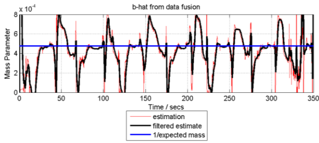
Figure 5. Illustration of the problem of the mass estimation parameter converging on the correct estimate only during certain periods of time. A straight line representing the expected mass may be compared to the raw estimate and its periods of convergence.
