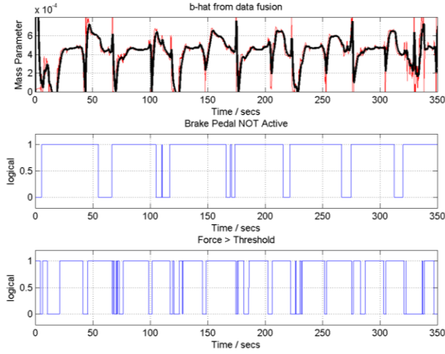
Figure 7. Illustration of two of the logical metrics used to select data for use in the estimate-convergence output filtering method. The raw mass parameter \hat{b} = \frac{1}{m} estimate is shown again (Top) to allow comparison between data rejection and periods of good estimate.
