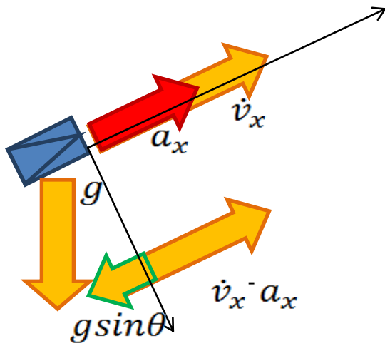
Figure 2. Diagram for the longitudinal accelerometer attached to a vehicular system providing the different accelerations to produce the measured output a_x
