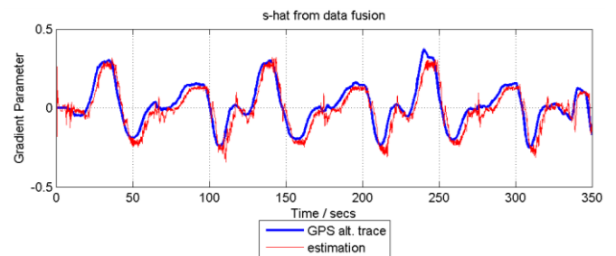
Figure 4. A comparison of gradient estimation from the algorithm presented in this paper and in [1] and the result from a GPS altitude trace for the same driving duty cycle - note the inconsistency of the GPS at around 240 seconds
