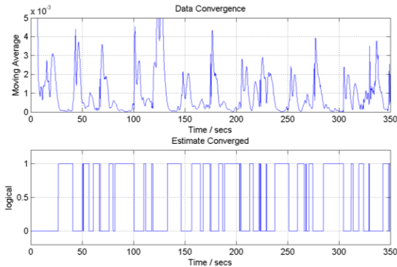
Figure 8. The moving average of the temporal gradient of the error mass estimate \hat{b} = \frac{1}{m} with itself over a predefined time before the present (Top) is compared to a threshold to give an indication of periods of convergence of the estimate (Bottom).
