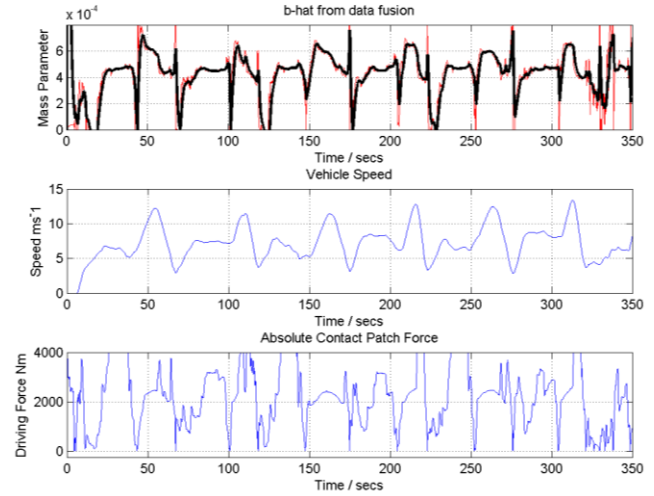
Figure 6. Illustrations of the effect of certain aspects of the driving duty cycle on the quality of the mass parameter \hat{b} = \frac{1}{m} (Top). The vehicle speed being low (stationary) at the beginning of the run has a large impact on initial conditions because this introduces a set of conditions where the measured accelerations and forces do not match and errors between them are greatly amplified (Middle), it should also be noted that the local minima in the speed trace represent the vehicle negotiating a tight turn, which introduces additional losses and these points coincide with the end of periods of low confidence in the driving force estimate due to deceleration. The absolute value of driving force (bottom) shows a clear correlation with the shape of the mass parameter estimate, especially between 'small' force measurements and singularities in the output solution.
