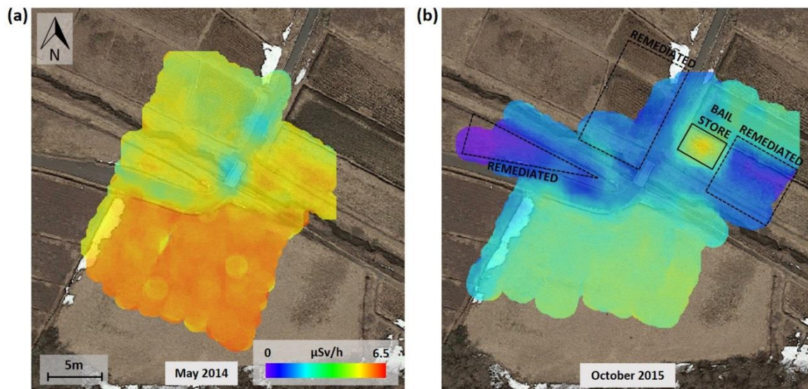
Fig. 3. Radiation intensity distribution maps taken from Iitate (Location 2), displayed as normalised to 1 m above the ground surface in dose rate ( \mu\text{Sv/h} ), (a) taken in May 2014 and (b) the same site surveyed later during October 2015.
