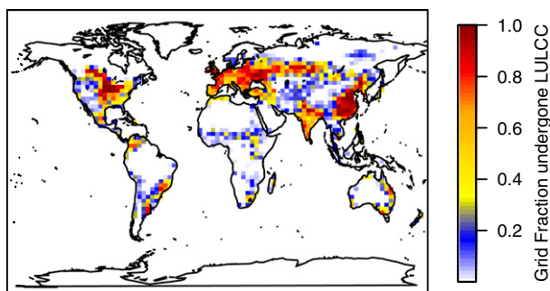
Figure 1. Map showing the proportion of each grid square in HadCM3 that has undergone LUC according to the land-cover mask of Betts et al. (2007b). Final disturbed fraction is calculated with this mask minus the non-vegetation types simulated by TRIFFID.
