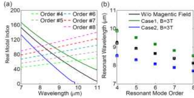
Fig. 4. The real modal indices on from Eq. (3) (solid lines) and Eq. (4) (dashed lines) are shown in (a). The crossover points in (a) and the resonant wavelengths from numerical simulations are illustrated using star markers and square markers, respectively.
