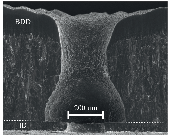
Figure 4. Scanning electron micrograph of a bisected microdischarge device, showing cross-section of eroded cathode (original hole diameter D = 200 \mu\text{m} ) and unaffected dielectric layer after \approx 5 h continuous operation at \approx 1 W discharge power under p(\text{He}) = 3 atm.
