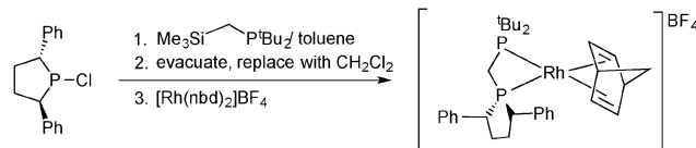
Scheme 2 One pot synthesis of [\text{Rh}(\text{nbd})(\text{L}_j)] .
