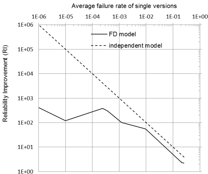
Fig. 2. Reliability improvement for 1-out-of-2 pair (FD model)
