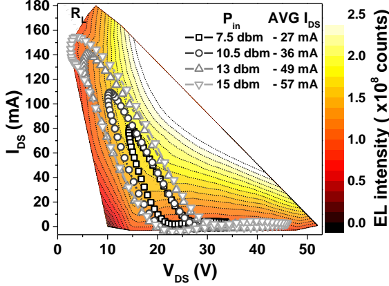
FIG. 1: (Color online) Contour map of the EL intensity of an AlGaIn/GaN HEMT as a function of drain voltage and drain current obtained under DC operation. Superimposed are the load lines for Class B for the indicated input powers ( P_{in} ) and average drain current ( AVG I_{DS} ). The quiescent bias point is located at V_{DS} = 24 V and V_{GS} = -3.7 V. The black dotted line represents the load line used for the DC EL intensity measurements with load resistance R_L .
