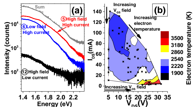
FIG. 5: (Color online) (a) Spectra of three representative points of the 15 dBm Class B load line with index numbers shown in Fig. 3(a) and the spectrum obtained as a sum of all the spectra over all the indices. (b) Electron temperature contour map in the I_{DS} - V_{DS} plane measured under DC conditions. The crosses represent the points of measurement.
