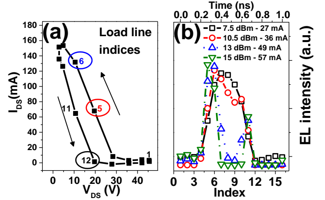
FIG. 3: (Color online) (a) Load line for Class B RF operation used, indicating points used for the detailed analysis of the EL intensity and EL spectrum. Only the 15 dBm load line is shown for clarity. (b) EL intensity spectrum versus index on the load line, over a full RF cycle. On the top x-axis the time scale is shown.
