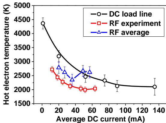
FIG. 4: (Color online) Electron temperature obtained on an AlGaIn/GaN HEMT operated under RF and DC as a function of average drain current determined by the EL spectrum. The curves are a guide for the eye.
