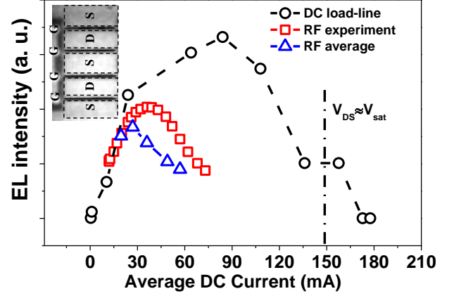
FIG. 2: (Color online) Electroluminescence (EL) intensity from an AlGaIn/GaN HEMT as a function of average DC drain current for RF Class B and DC operations, and the intensity integrated over the RF load line. The dashed lines are a guide to the eye. The vertical dash-dot line indicates where the current saturation onset starts (i.e. V_{DS} \approx V_{sat} ). In the inset the false color EL image is overlaid on a white-light image from the 4 \times 100 \mu\text{m} -wide device.
