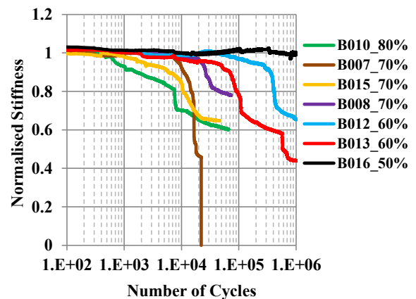
Fig. 10. Initial results obtained for the bolted ply-level fatigue tests.
