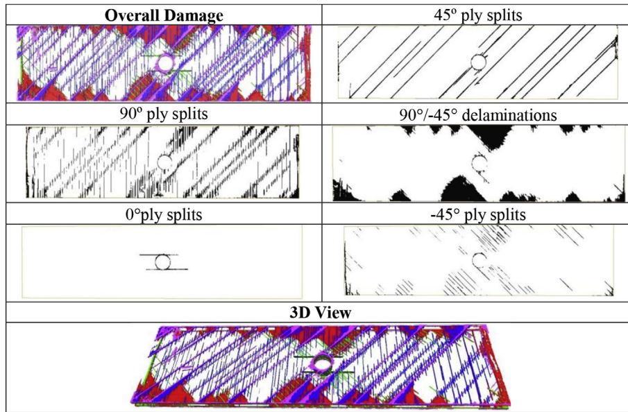
Fig. 13. CT images of a runout specimen at 50% severity for a ply-level test at 70 MPa.
