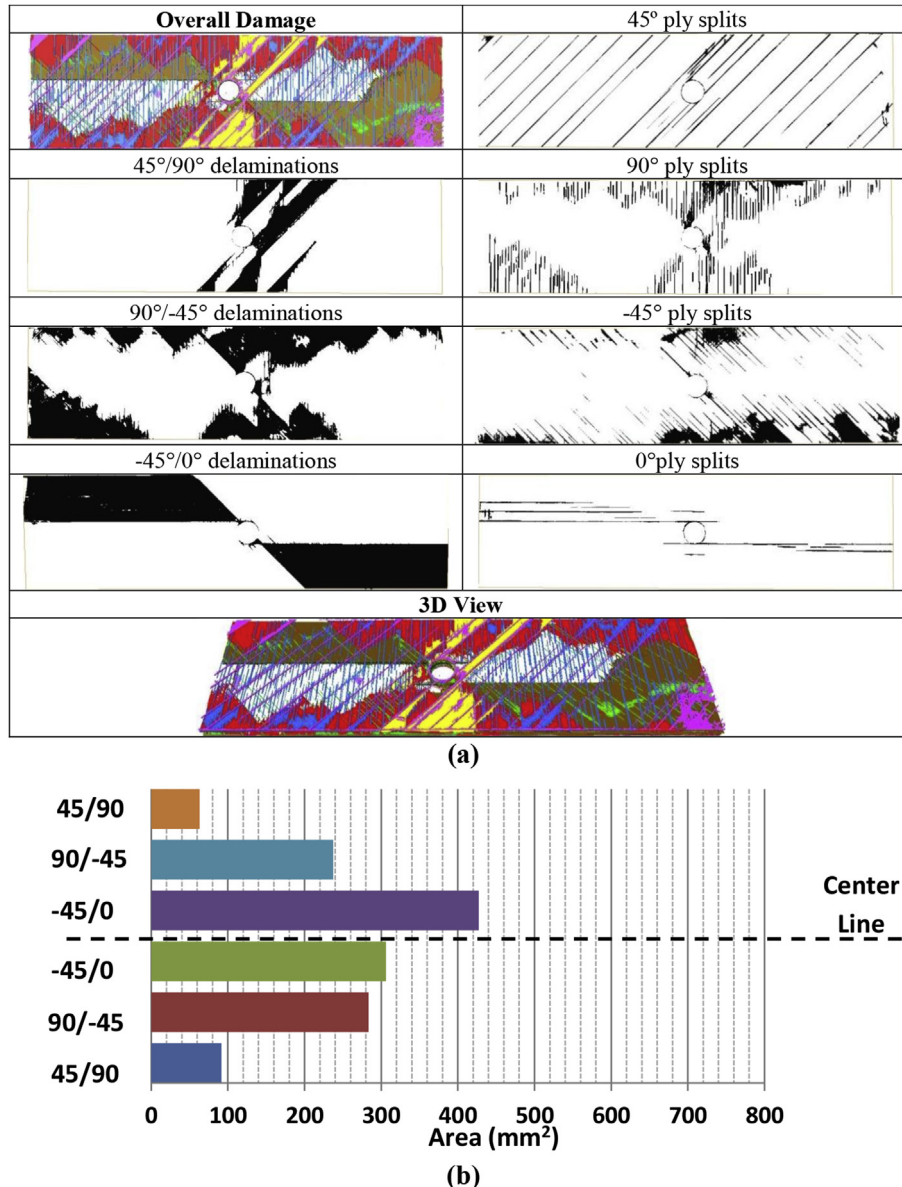
Fig. 11. Specimen B012 – 60% severity: (a) CT images, and (b) Damage area quantification through the thickness.
