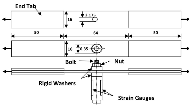
Fig. 1. Open and bolted hole specimen dimensions.
