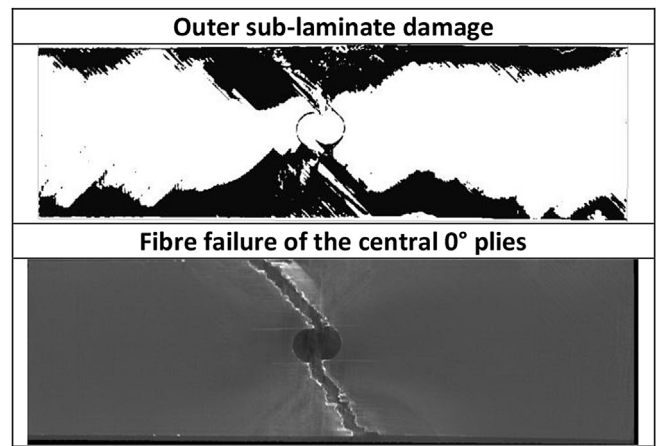
Fig. 19. Damage in the surface sublaminated, with the un-segmented image of the central 0° plies showing fibre-failure.
