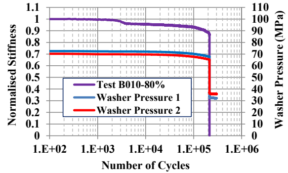
Fig. 18. Washer Pressures (primary axis) and stiffness (secondary axis) for the sublaminated-level bolted test B010-80%.
