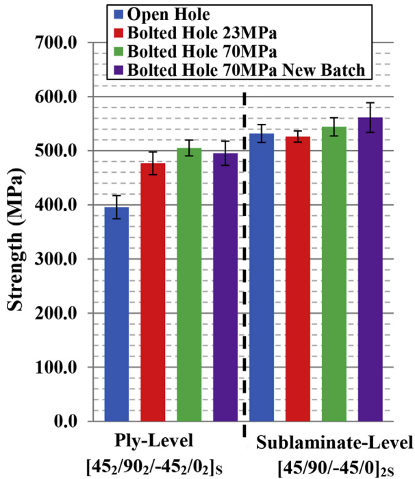
Fig. 7. Bar chart for all configurations for ply and sublaminates tests with their failure strengths.
