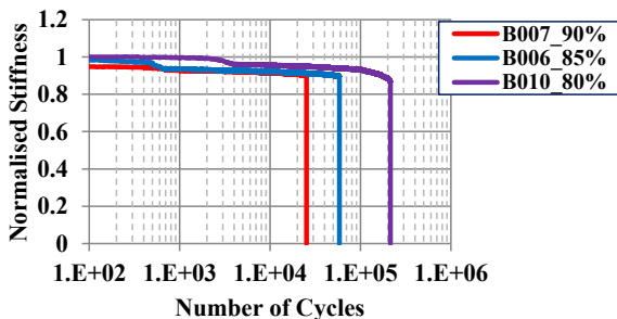
Fig. 17. Stiffness loss curve for each of the three severities tested for the bolted sublaminated specimens.
